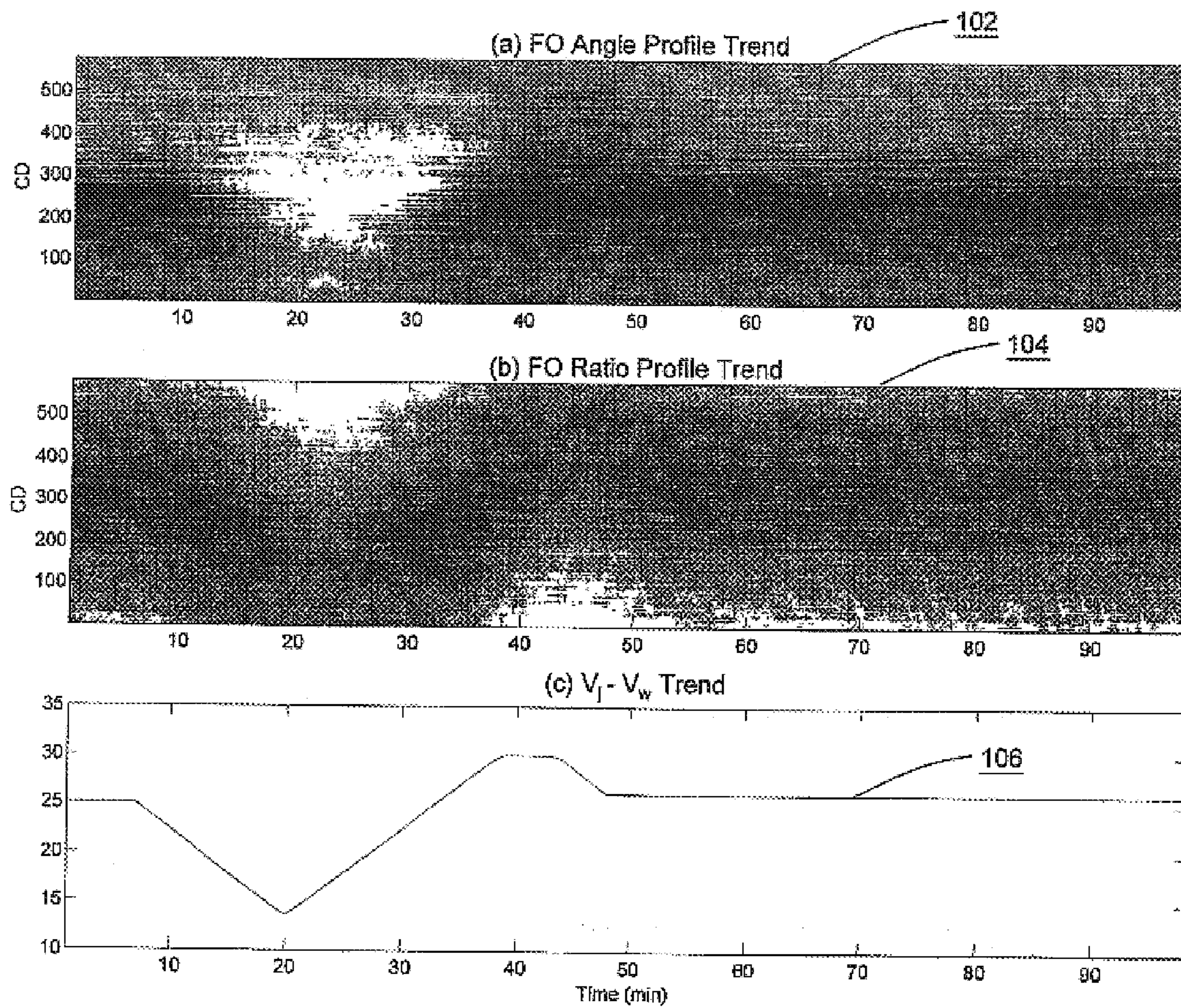
Fig. 8 Two FO profile contours and V_{jw} trend (100)
