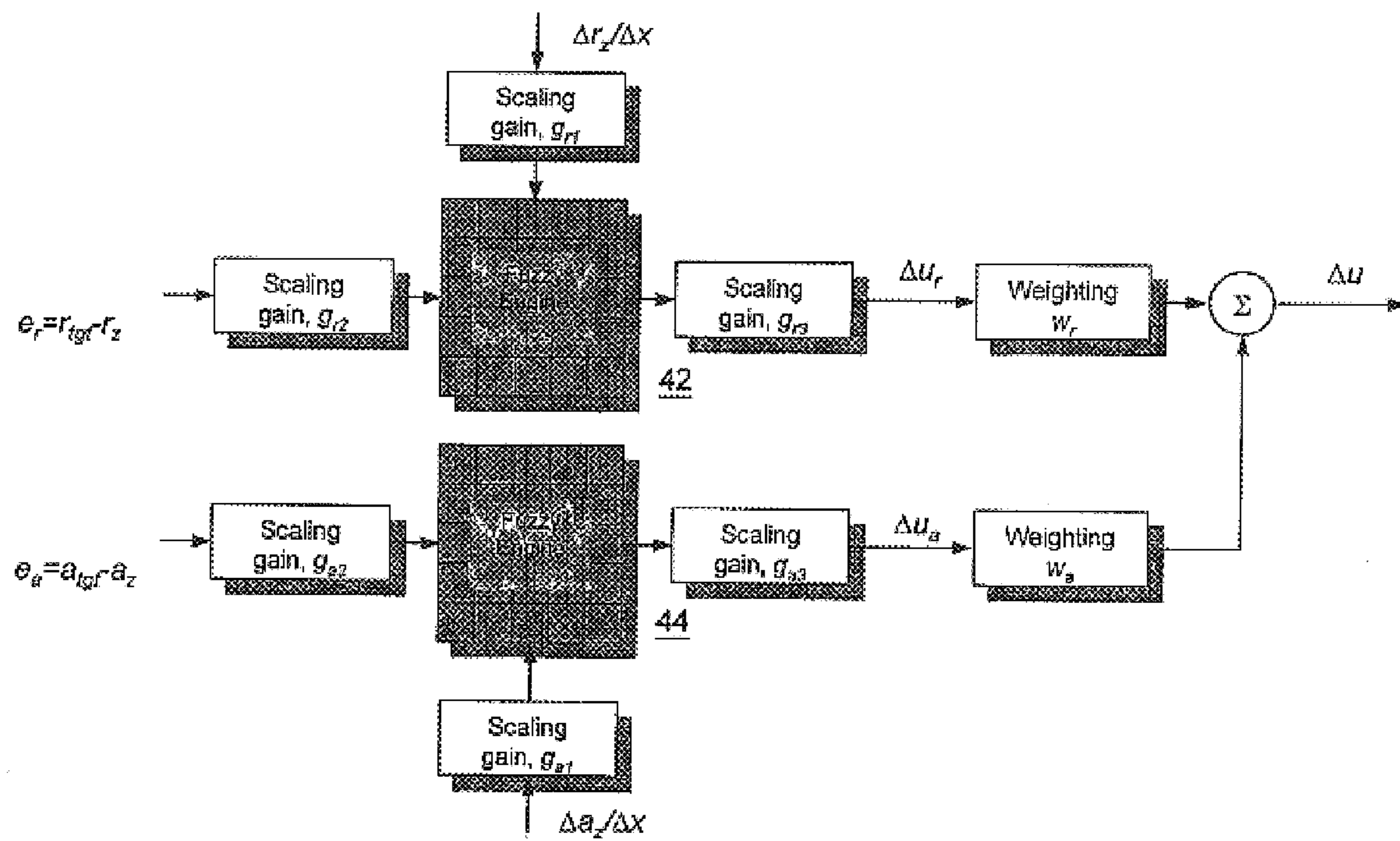
Fig. 3 Base FO controller (BFOC) implementation: embodiment 2 (40)
