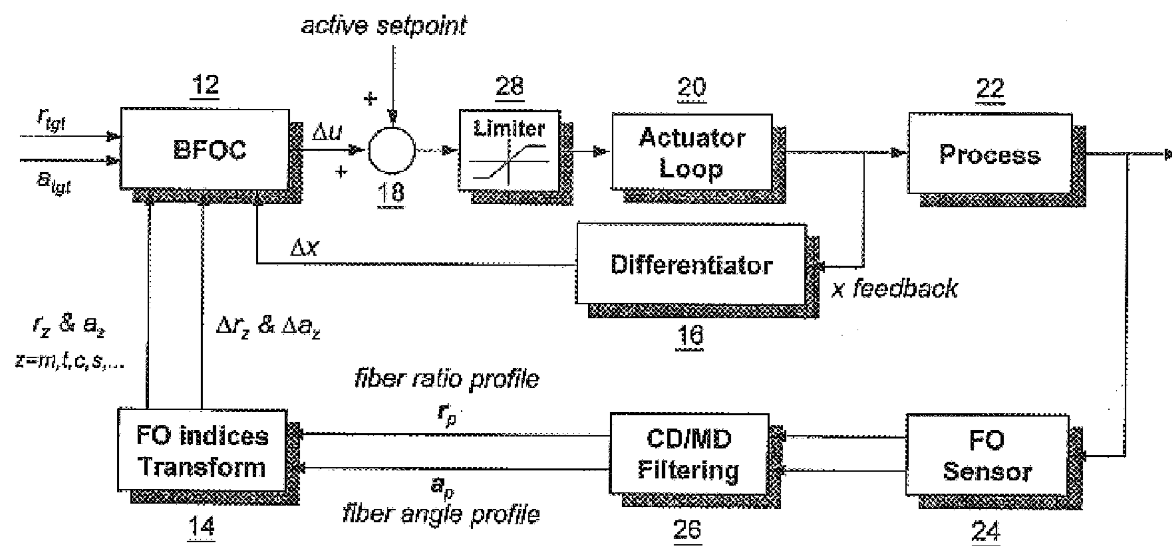
Fig. 1 Block diagram of base FO control (BFOC) system (10)
