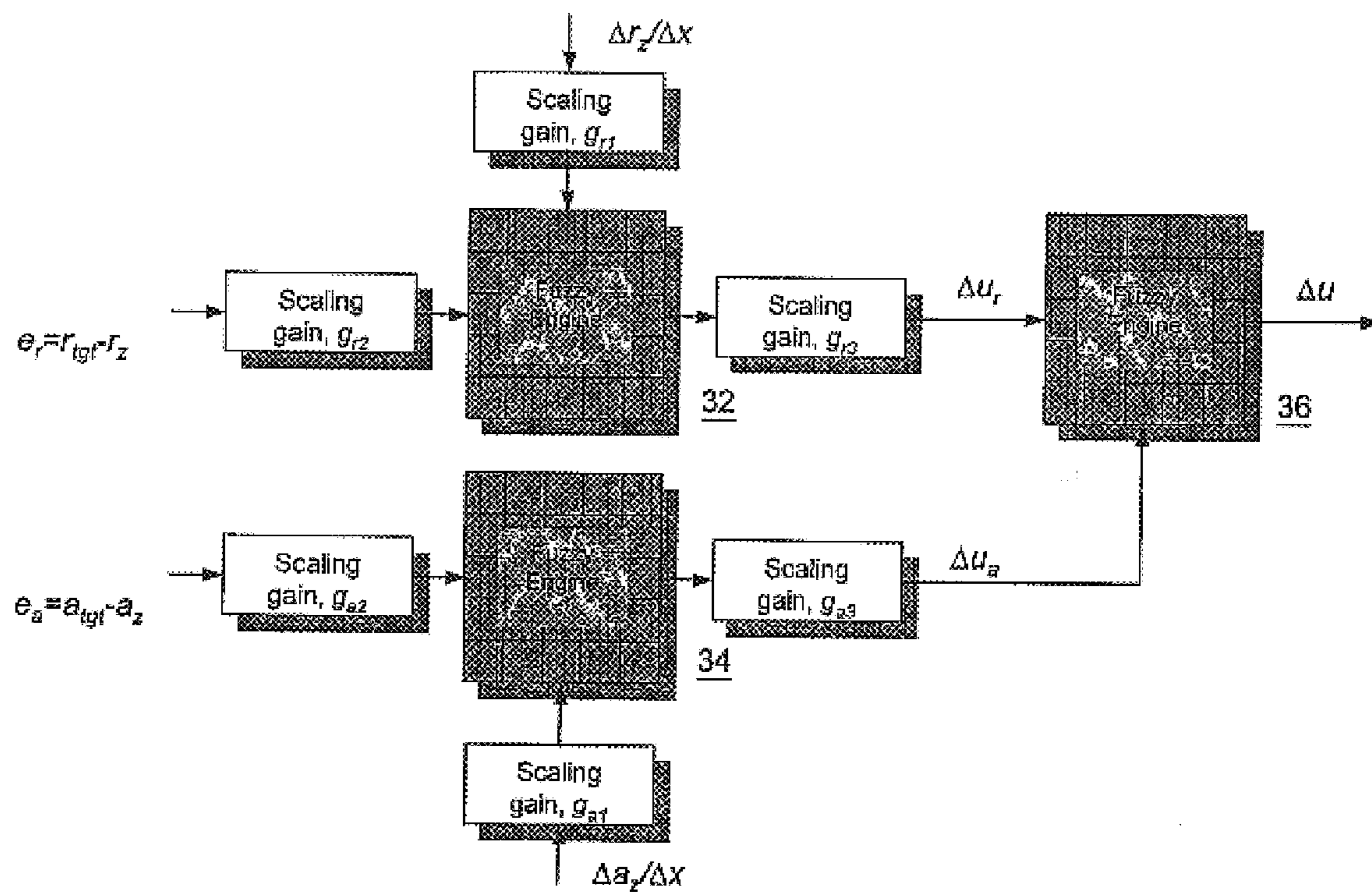
Fig. 2 Base FO controller (BFOC) implementation: embodiment 1 (30)
