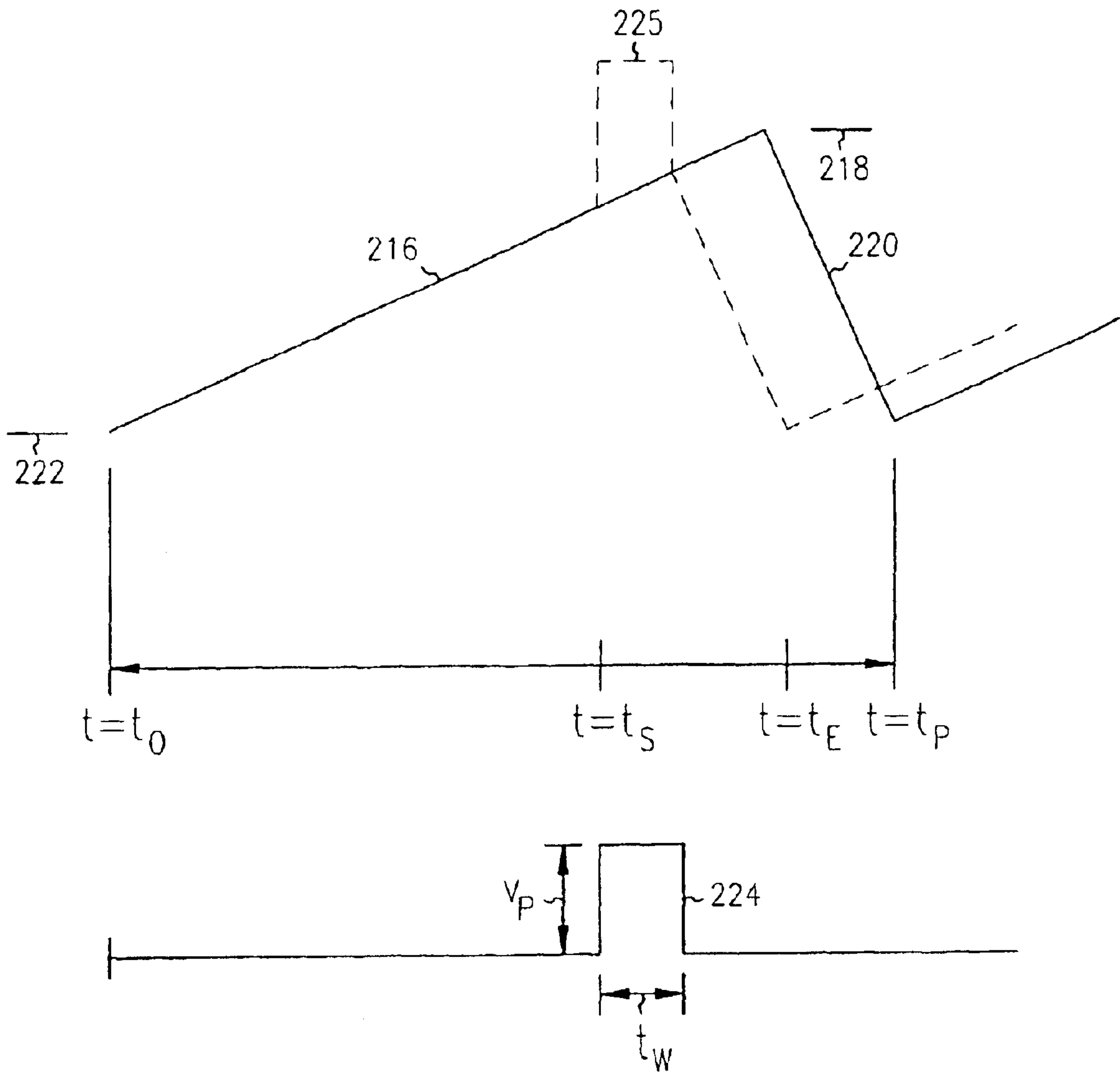
FIG. 2 (PRIOR ART)
