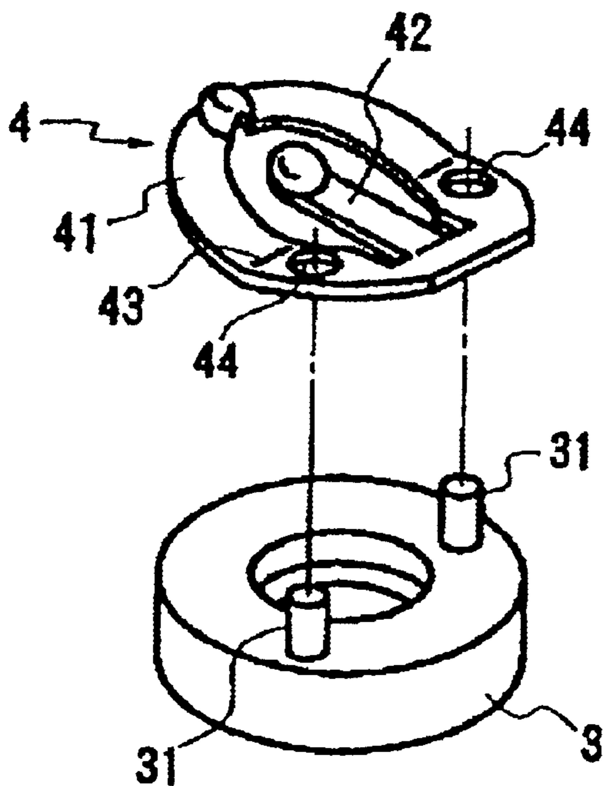
FIG. 4 PRIOR ART
