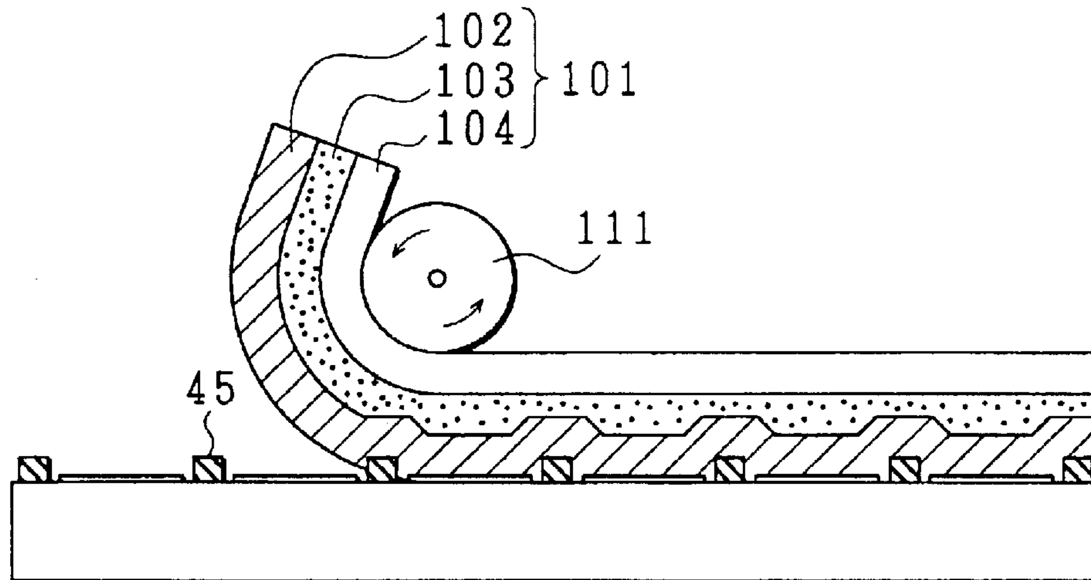
FIG. 11 (a) TRANSFER STEP
