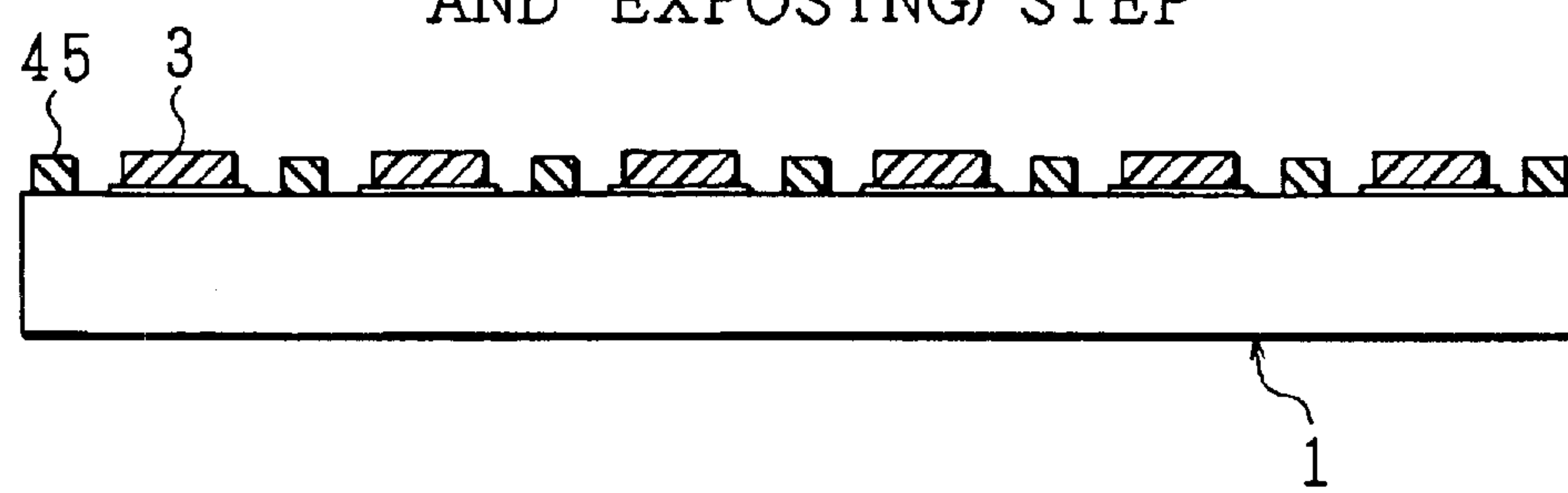
FIG. 11 (c) PHOTOLITHOGRAPHY (DEVELOPING AND EXPOSING) STEP
