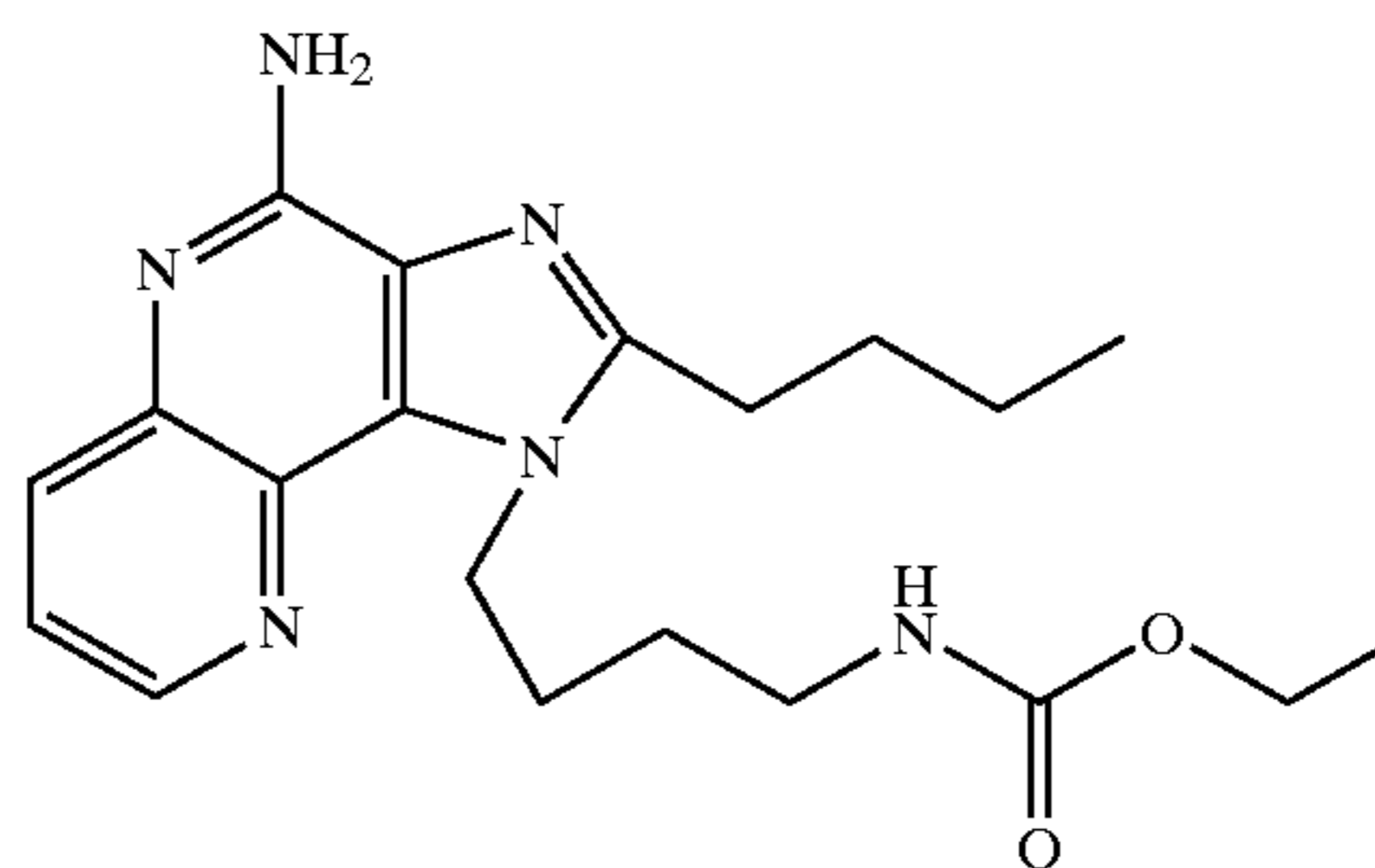
Ethyl N-[4-(4-Amino-2-butyl-1H-imidazo[4,5-c][1,5]naphthyridin-1-yl)butyl]carbamate
