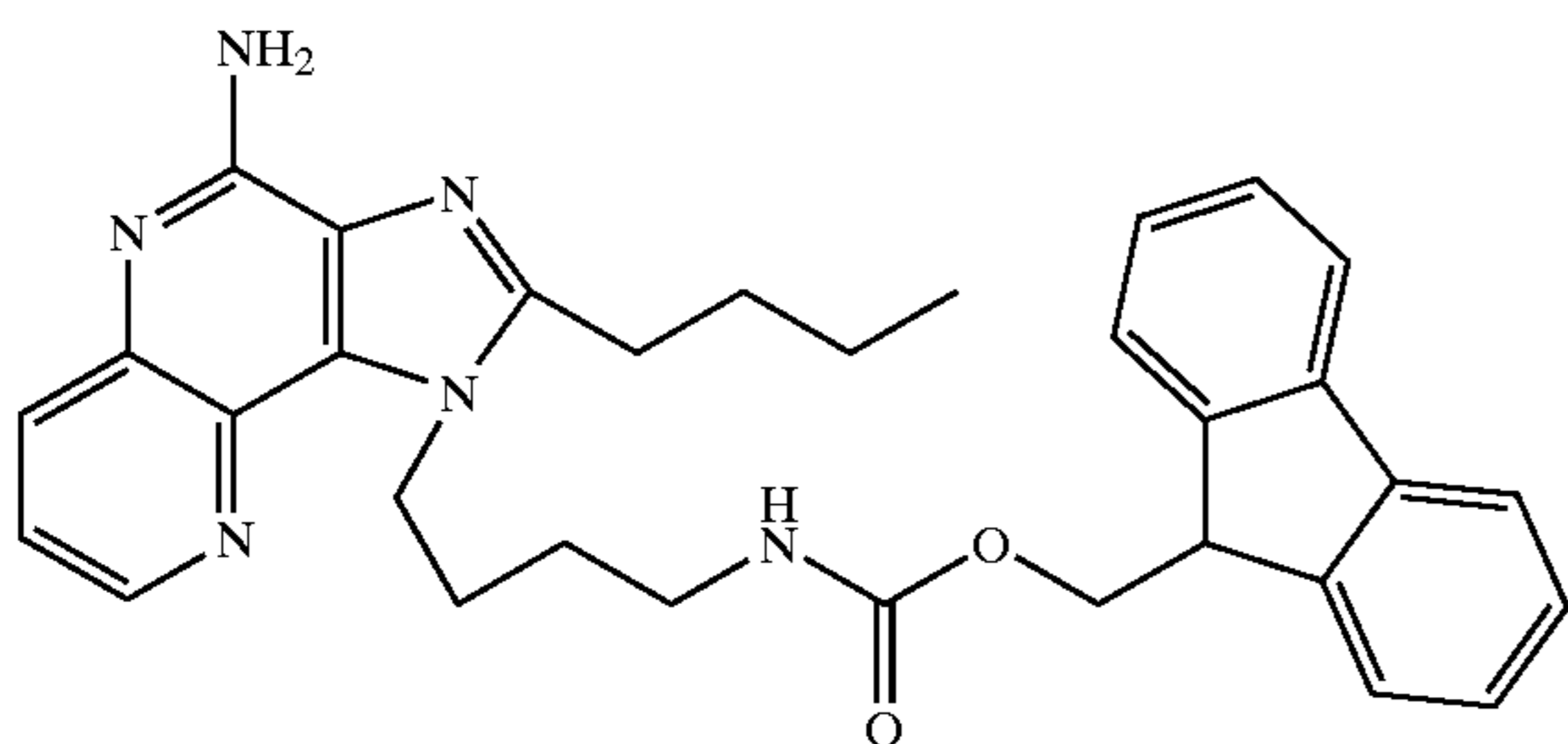
9H-9-Fluorenylmethyl N-[4-(4-Amino-2-butyl-1H-imidazo[4,5-c][1,5]naphthyridin-1-yl)butyl]carbamate
