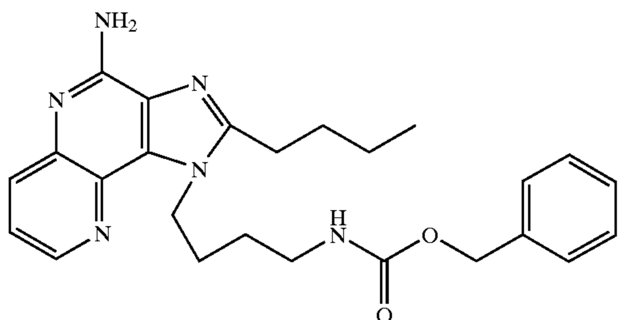
Benzyl N-[4-(4-Amino-2-butyl-1H-imidazo[4,5-c][1,5]naphthyridin-1-yl)butyl]carbamate
