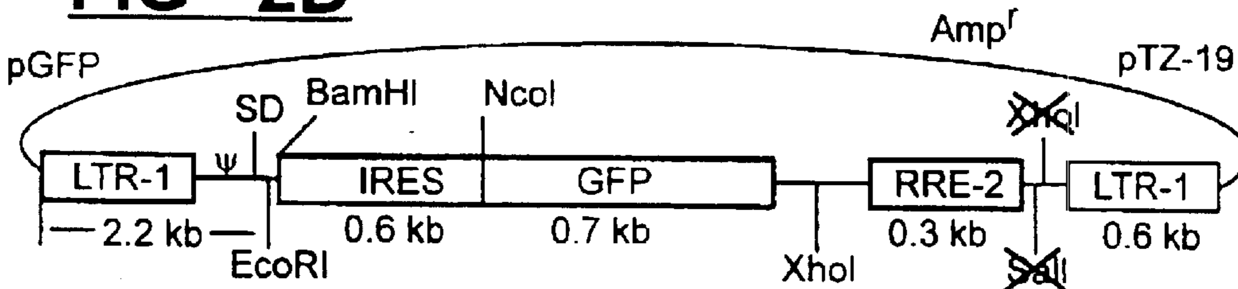
FIG - 2D
