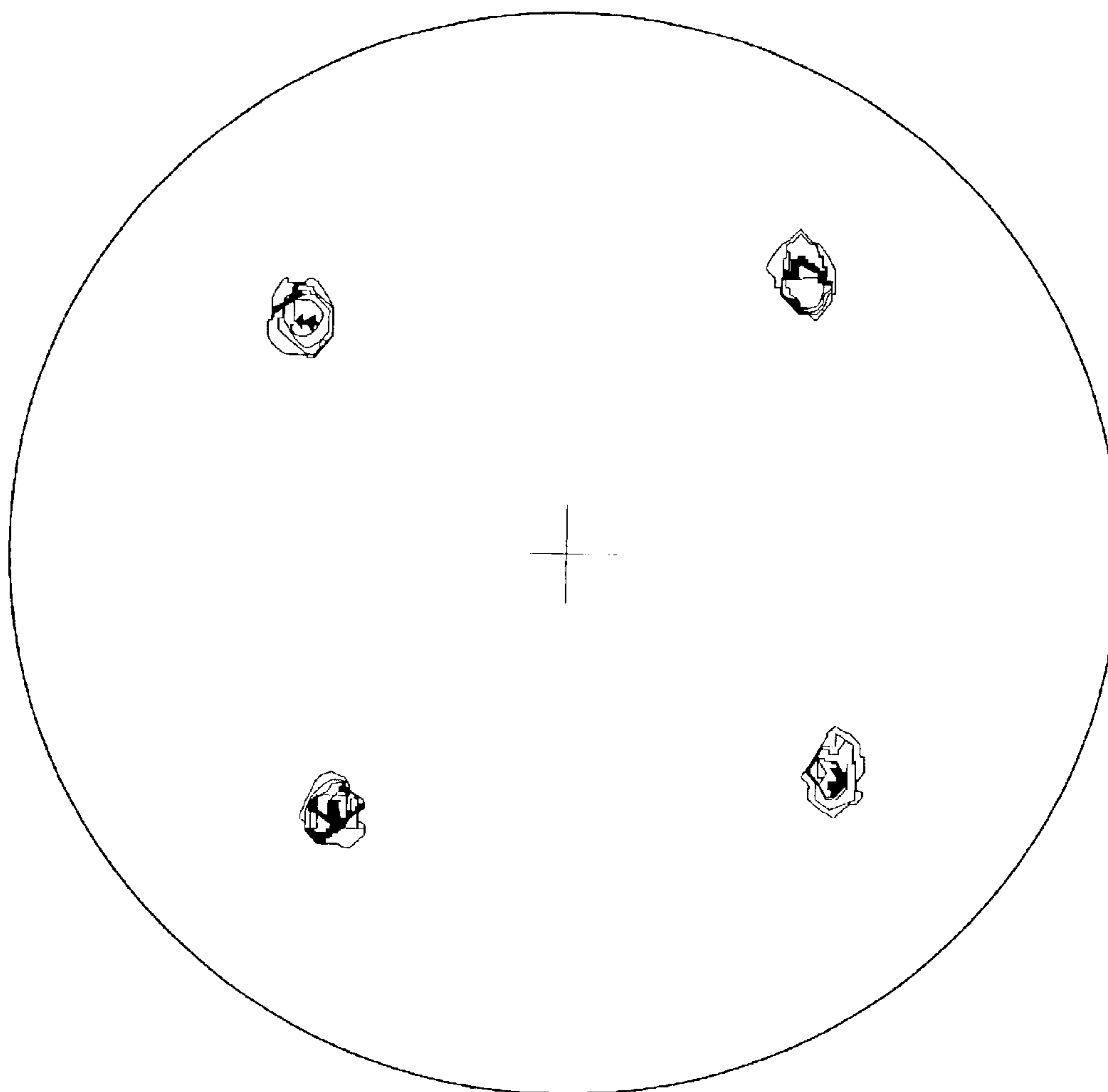
Ni-13at%Cr alloy Annealing Temperature = 1400°C
