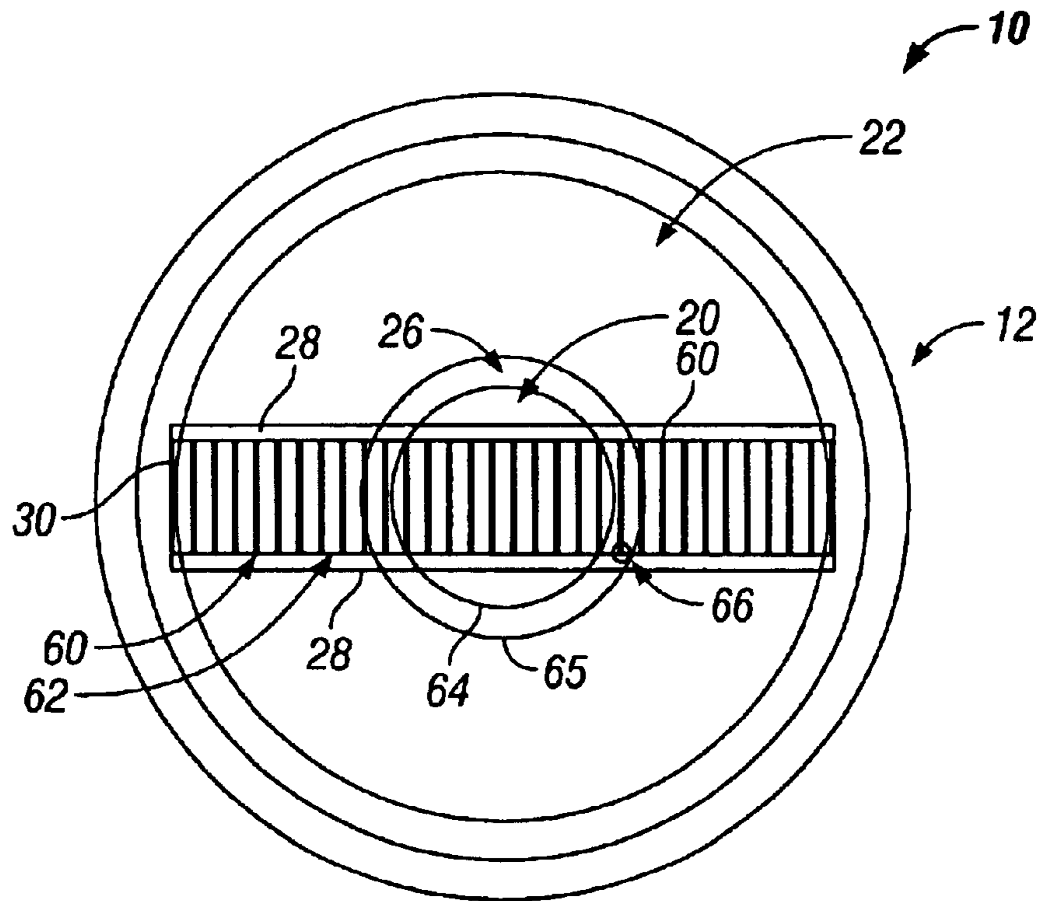
FIG. 3 (Prior Art)
