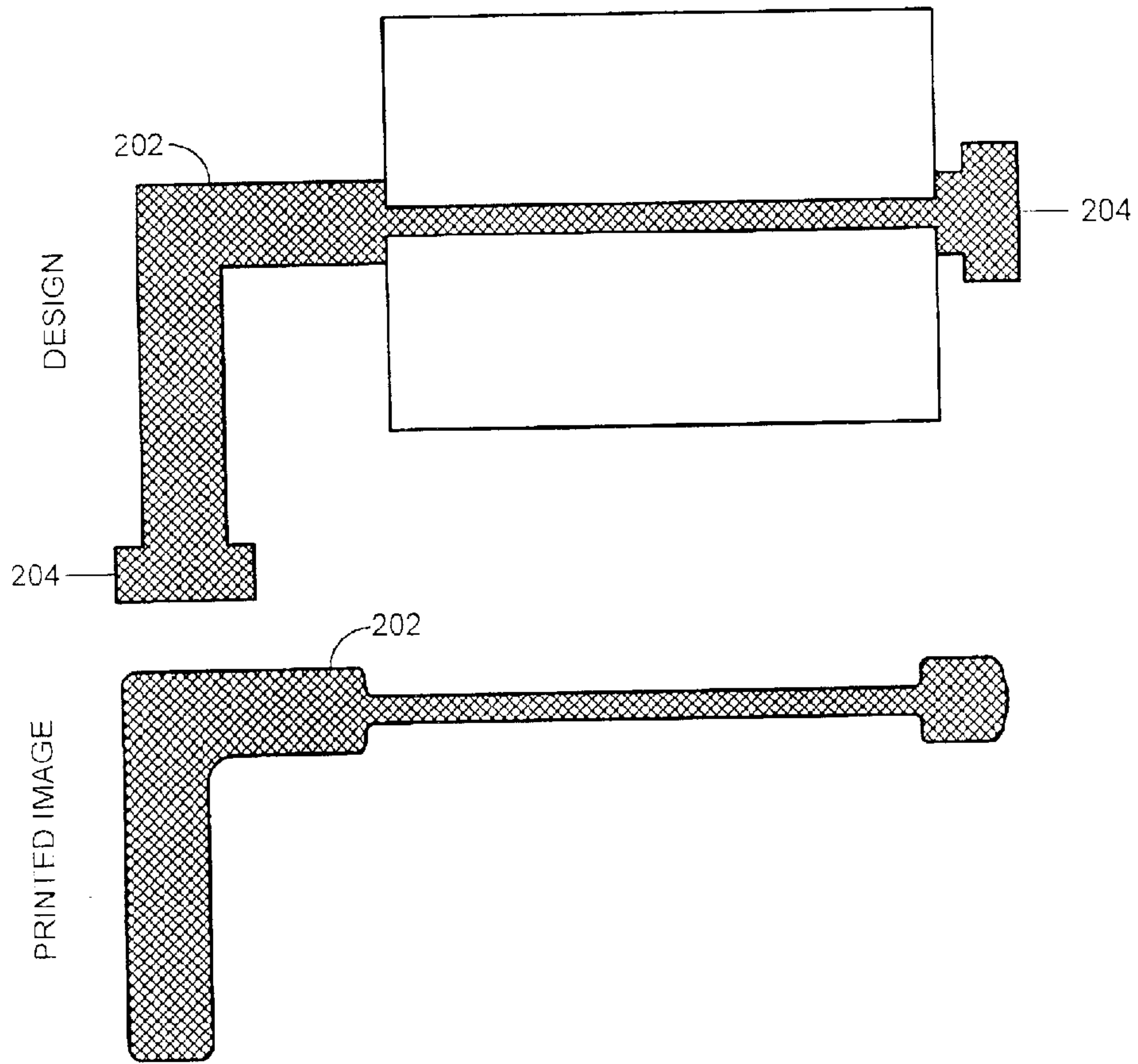
FIG. 2 (PRIOR ART)
