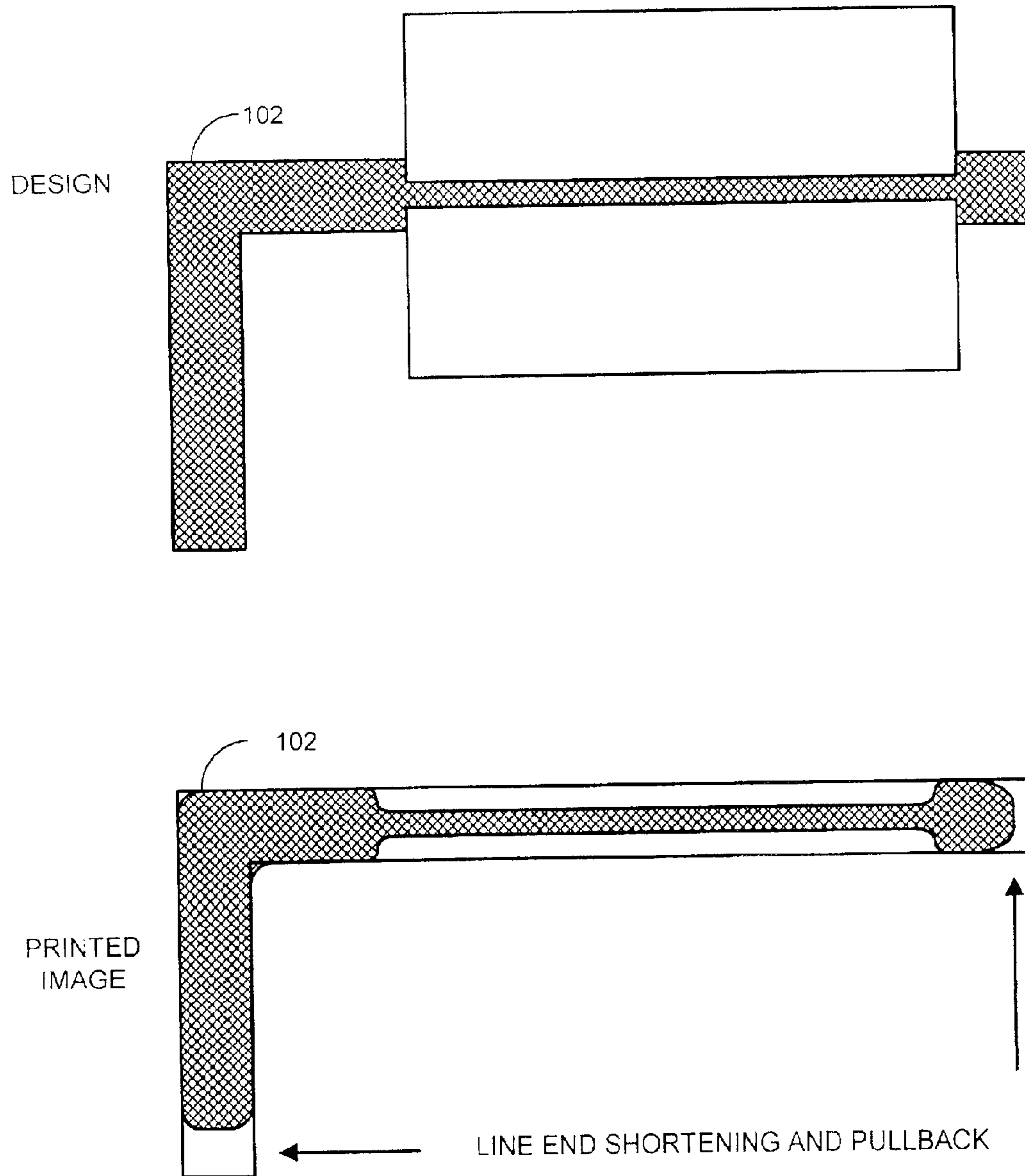
FIG. 1 (PRIOR ART)
