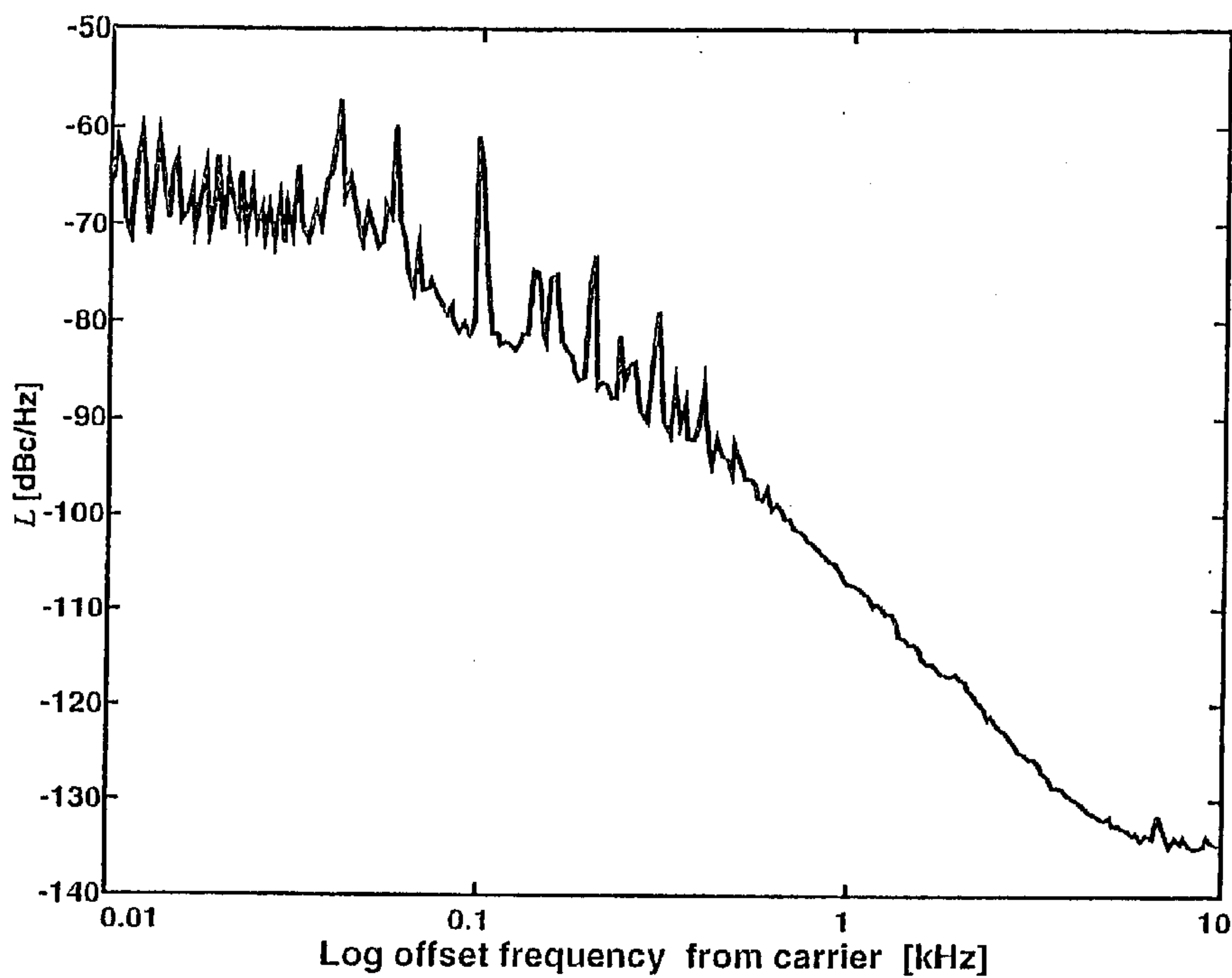
FIG. 28 PRIOR ART
