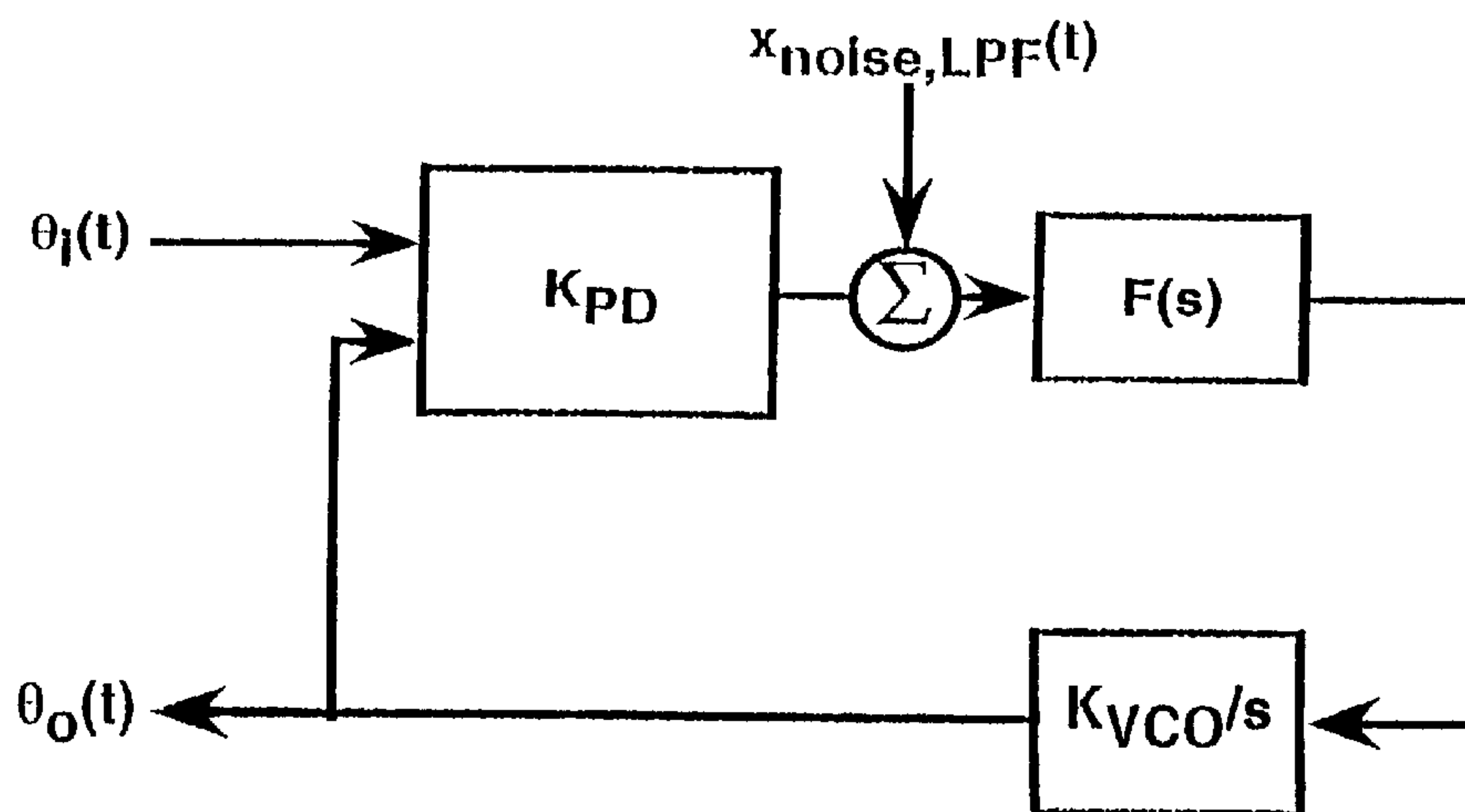
FIG. 18 Prior Art
