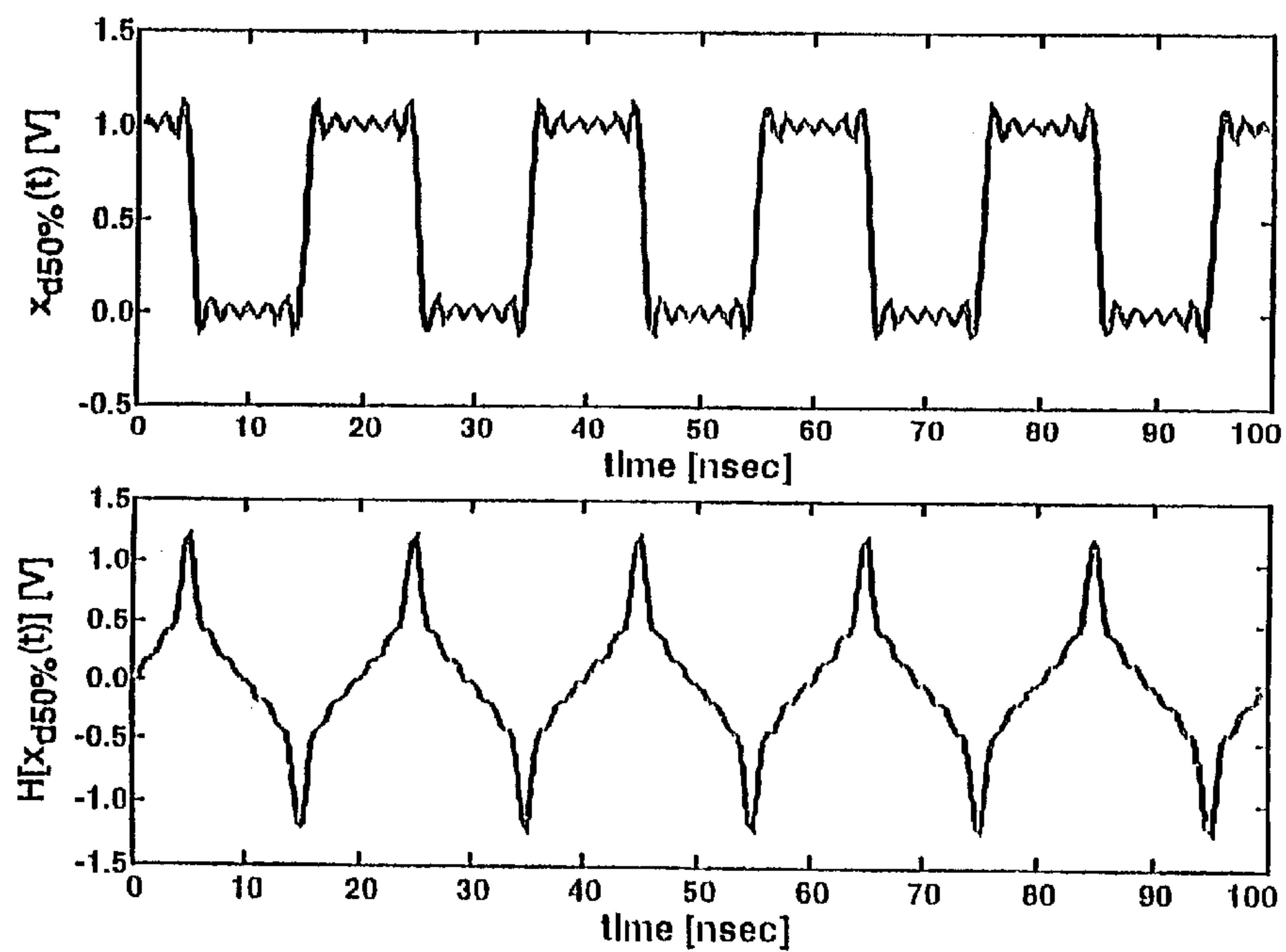
FIG. 22 Prior Art
