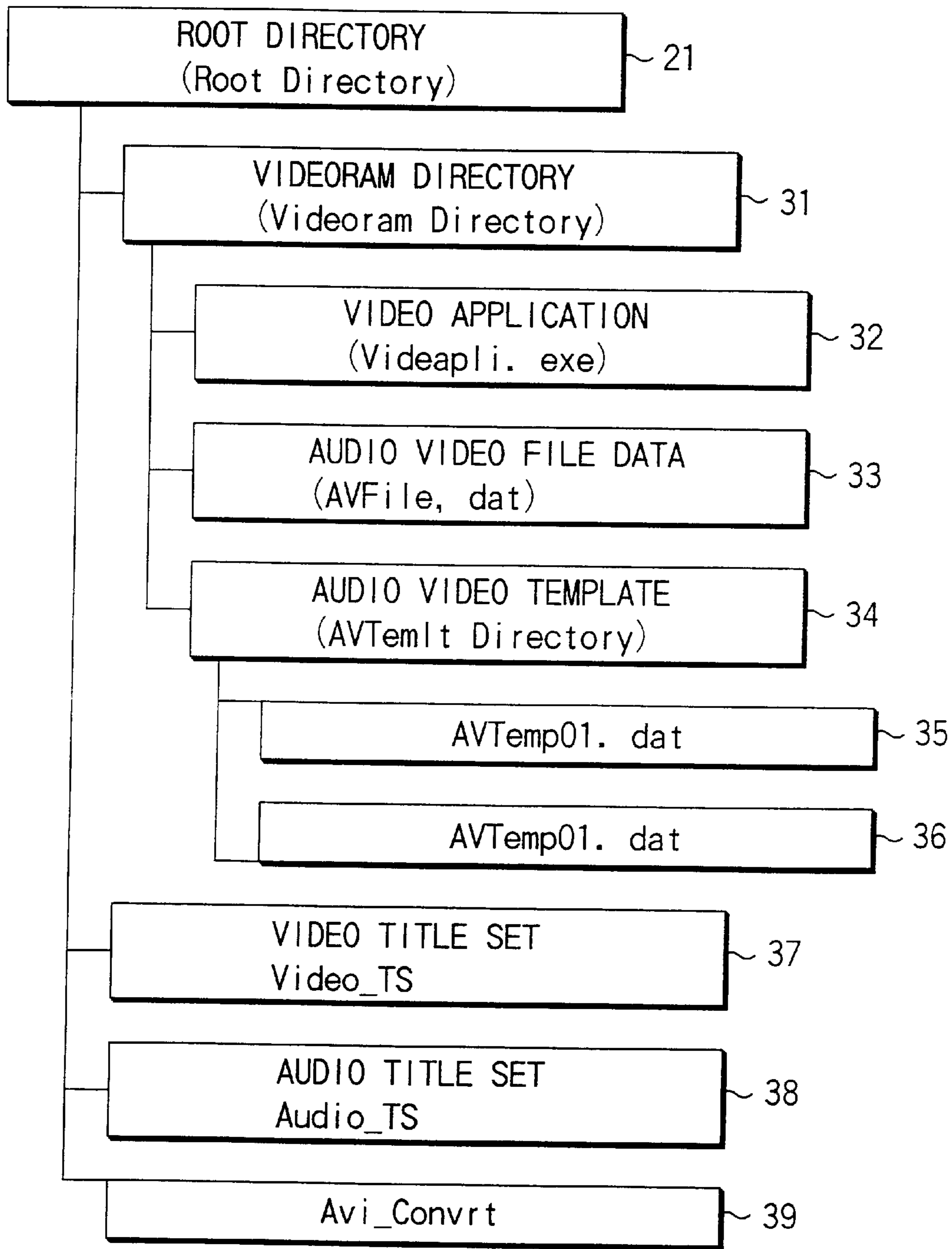
DIRECTORY STRUCTURE OF INFORMATION STORAGE MEDIUM FOR VIDEO INFORMATION PROCESSING
