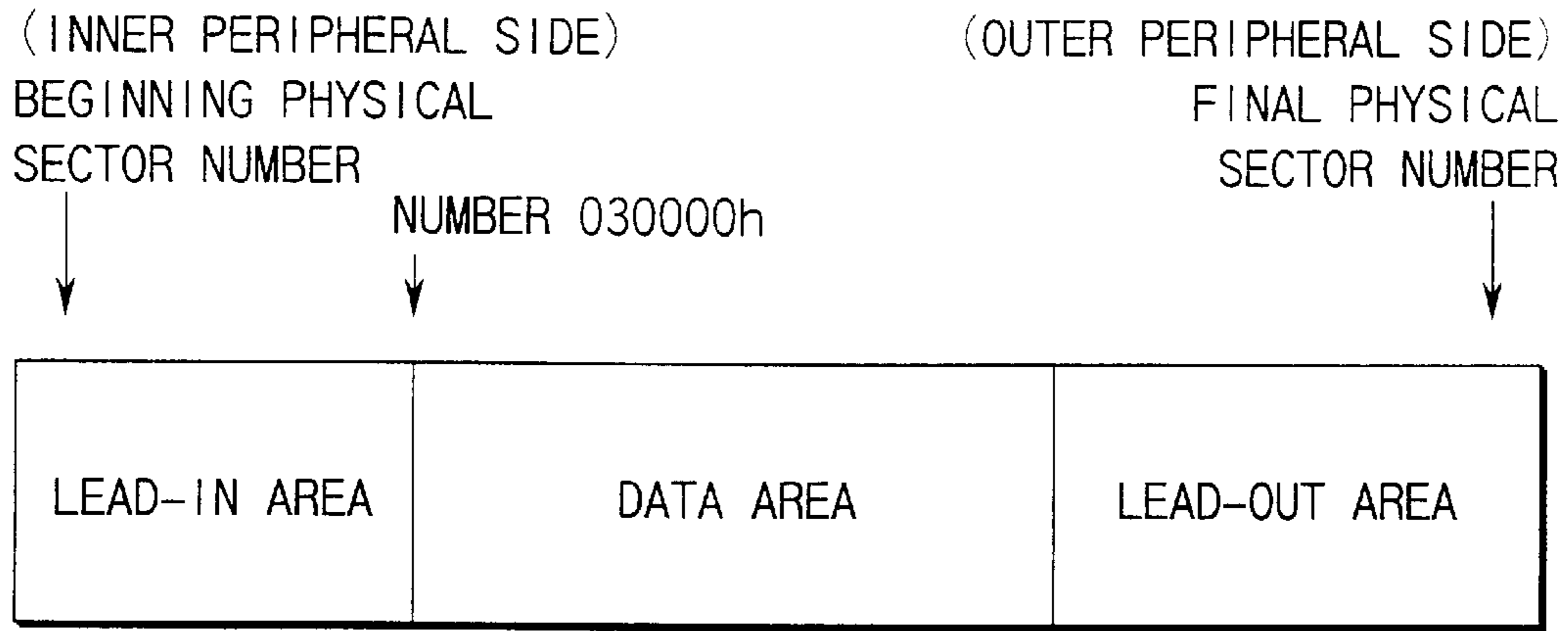
AREA STRUCTURE ON DVD-ROM DISK
