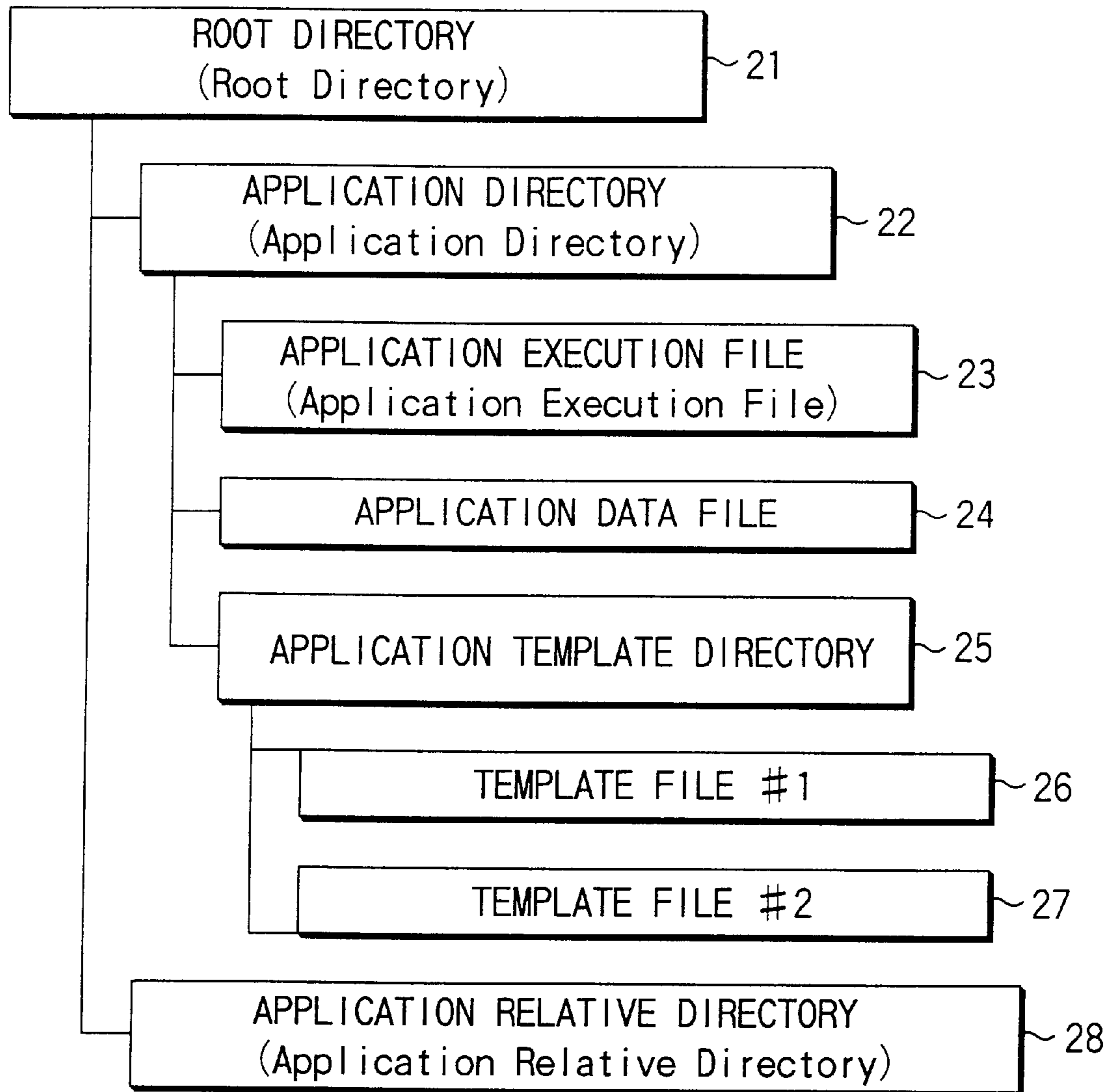
DIRECTORY STRUCTURE OF INFORMATION RECORDED ON INFORMATION STORAGE MEDIUM
