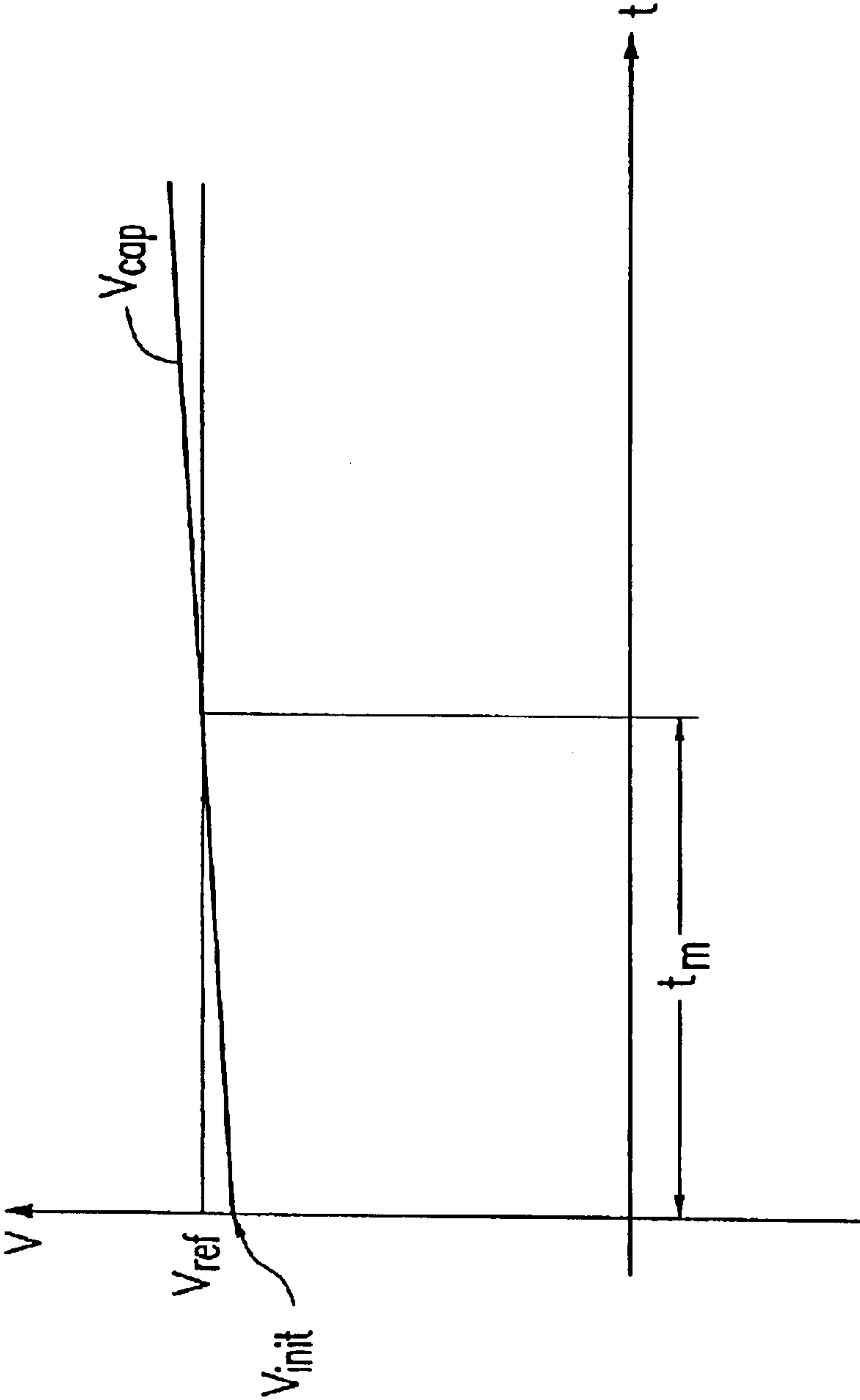
FIG. 2 (PRIOR ART)
