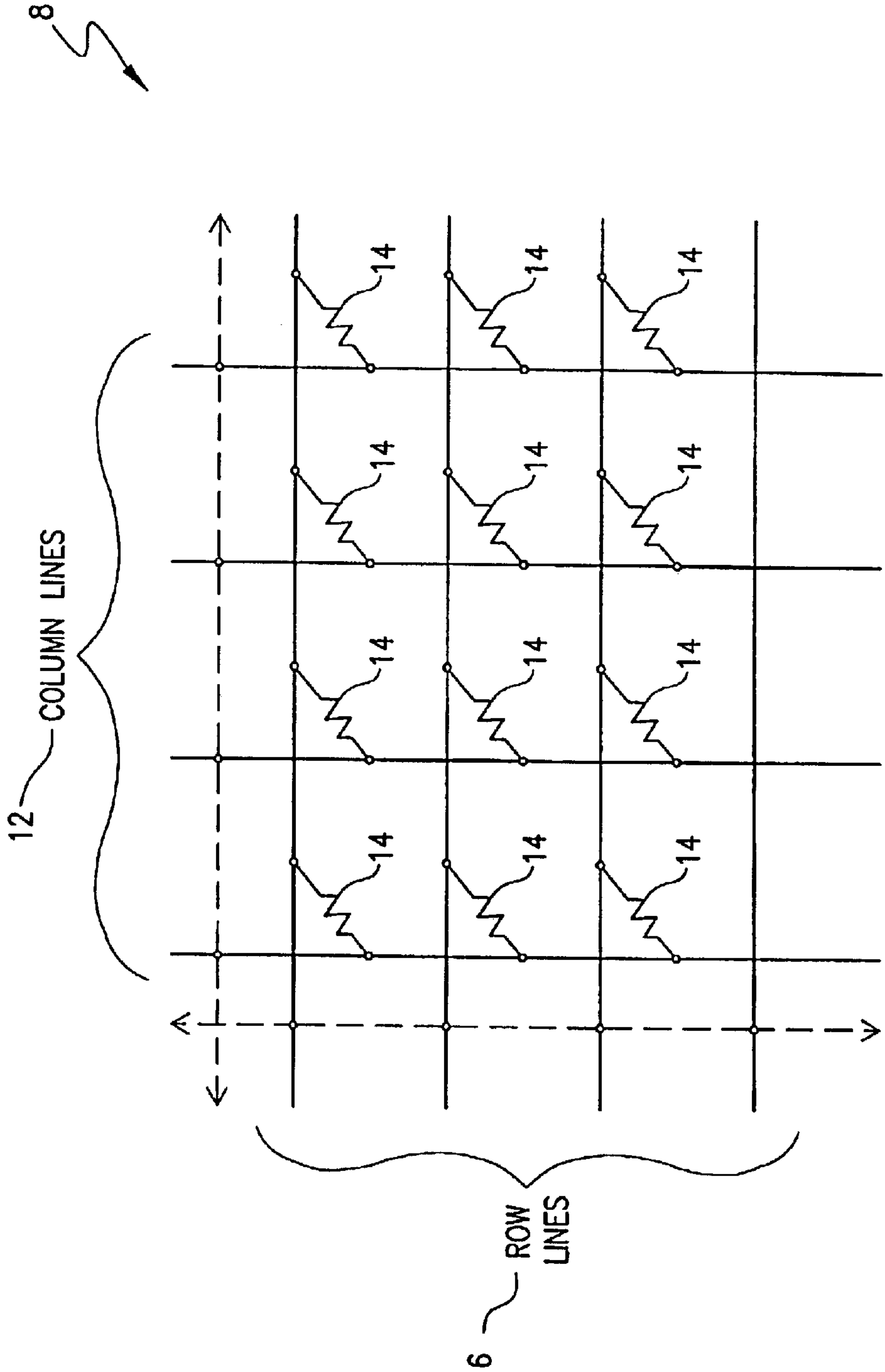
FIG. 1 (PRIOR ART)
