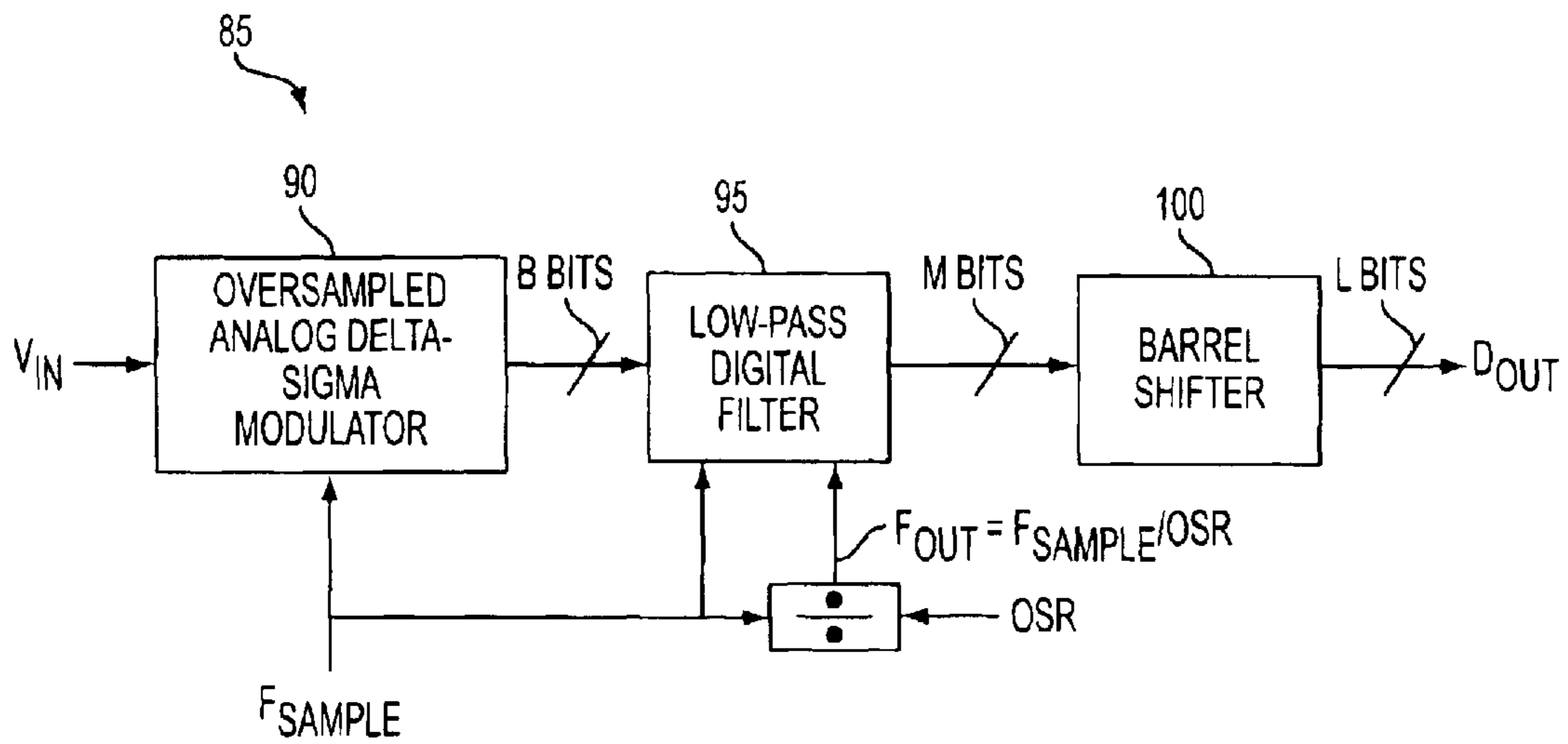
FIG. 5 (PRIOR ART)
