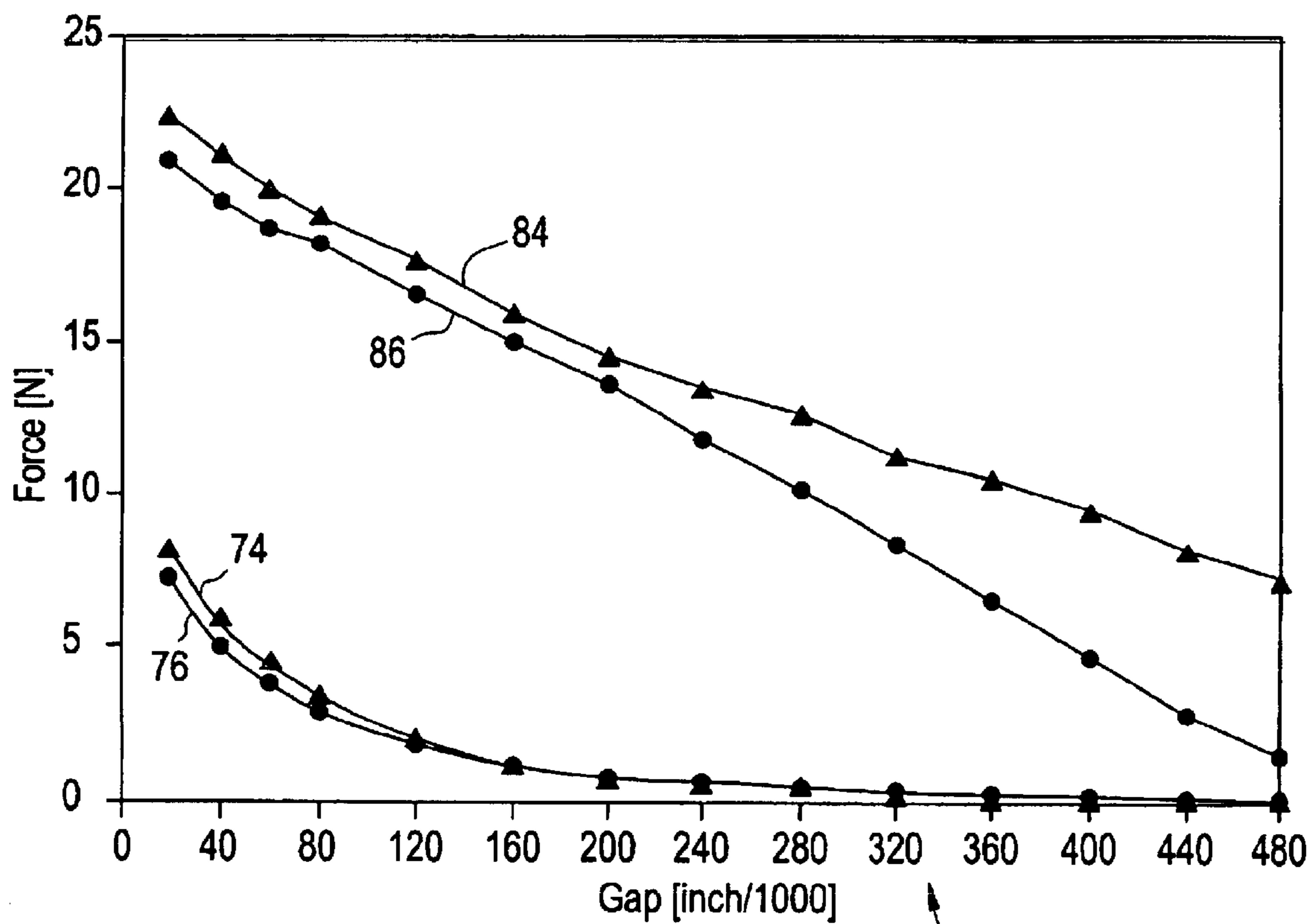
Force vs. Gap
