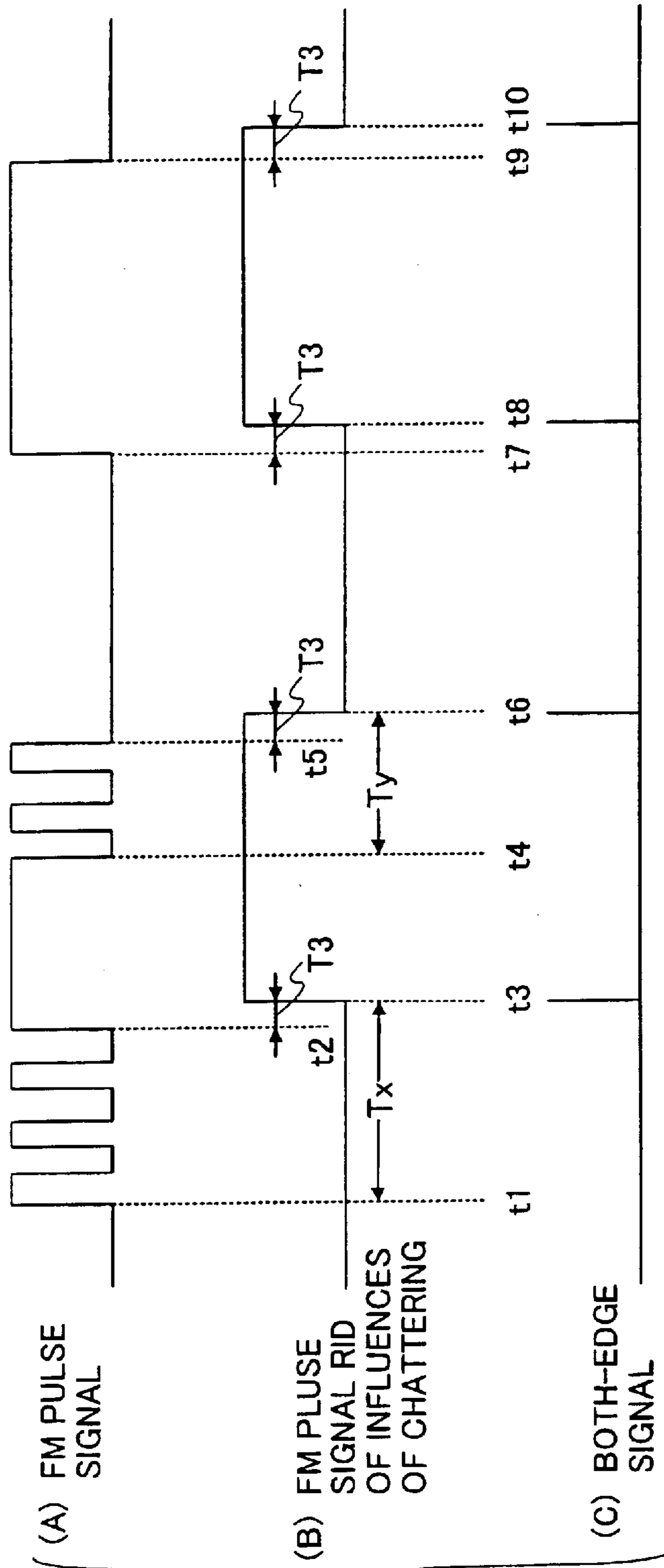
FIG. 7 PRIOR ART
