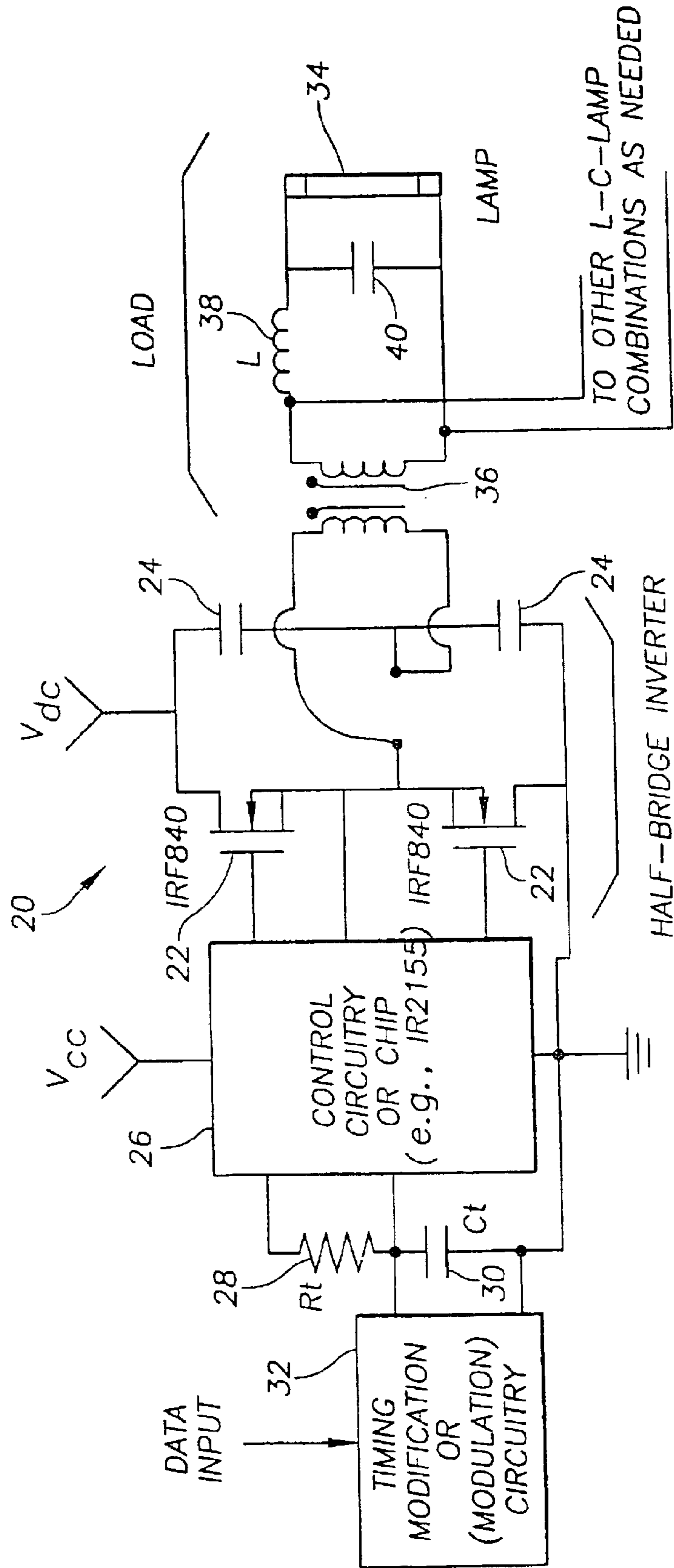
FIG. 2 HALF-BRIDGE INVERTER
