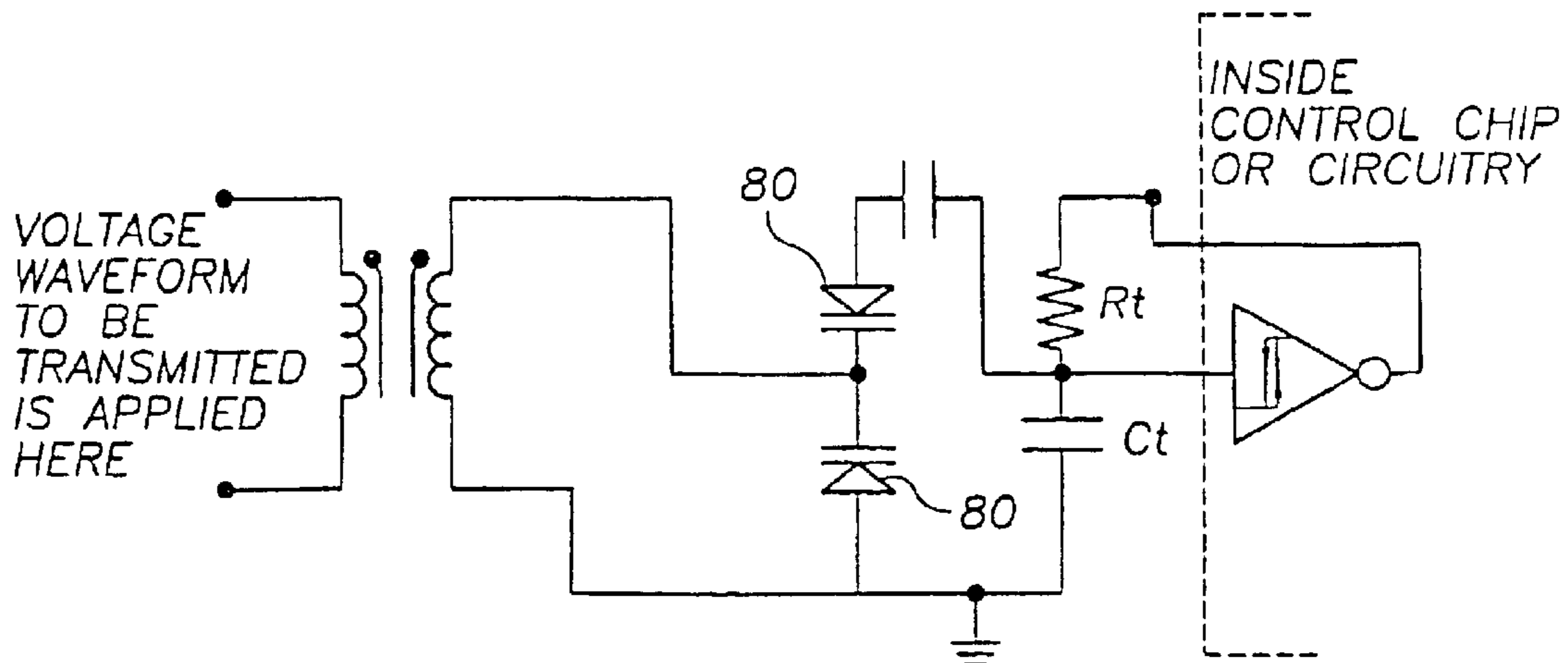
FIG. 7c MODULATION CIRCUITS.
