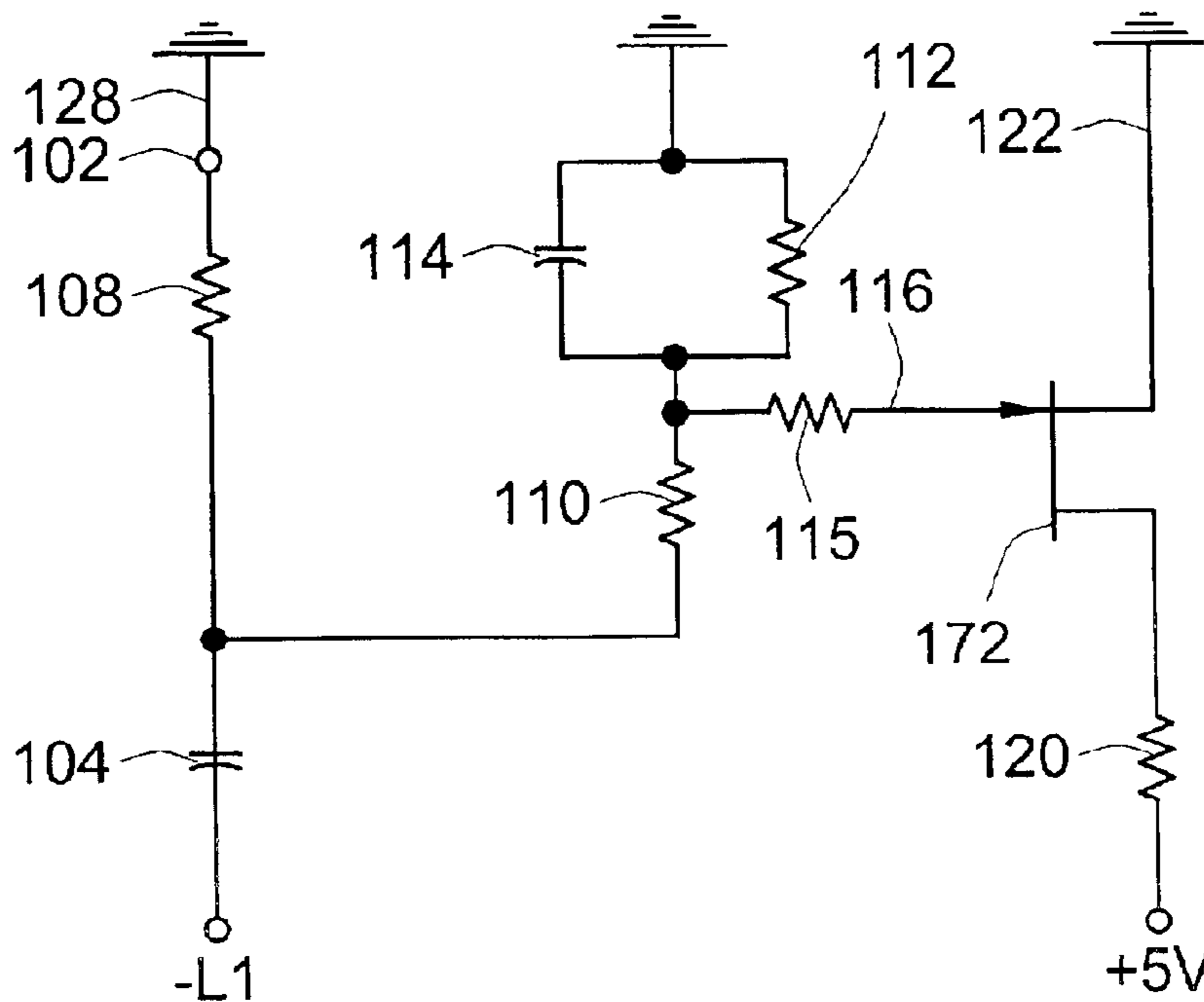
FIG. 4 (PRIOR ART)
