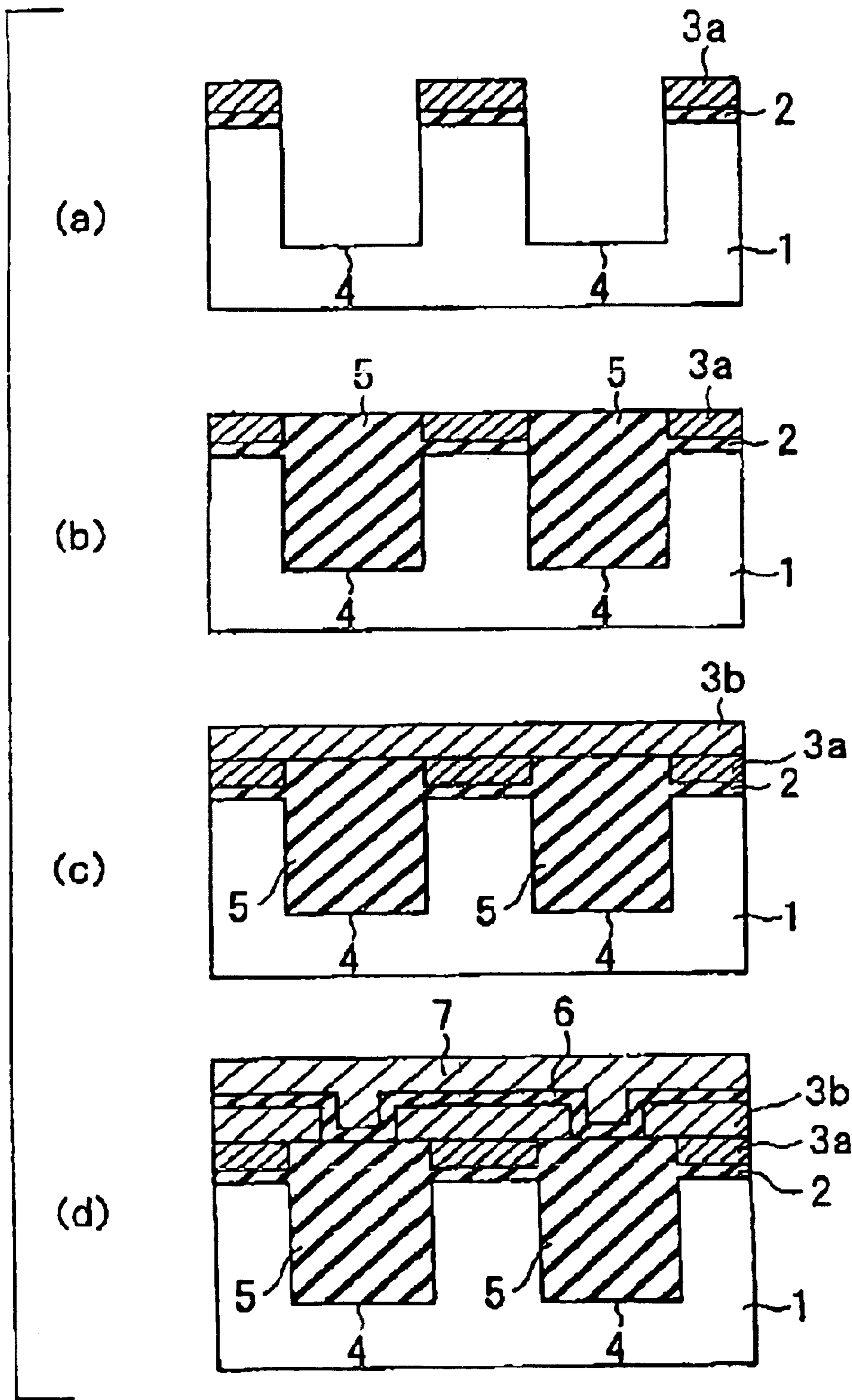
FIG. 35 PRIOR ART
