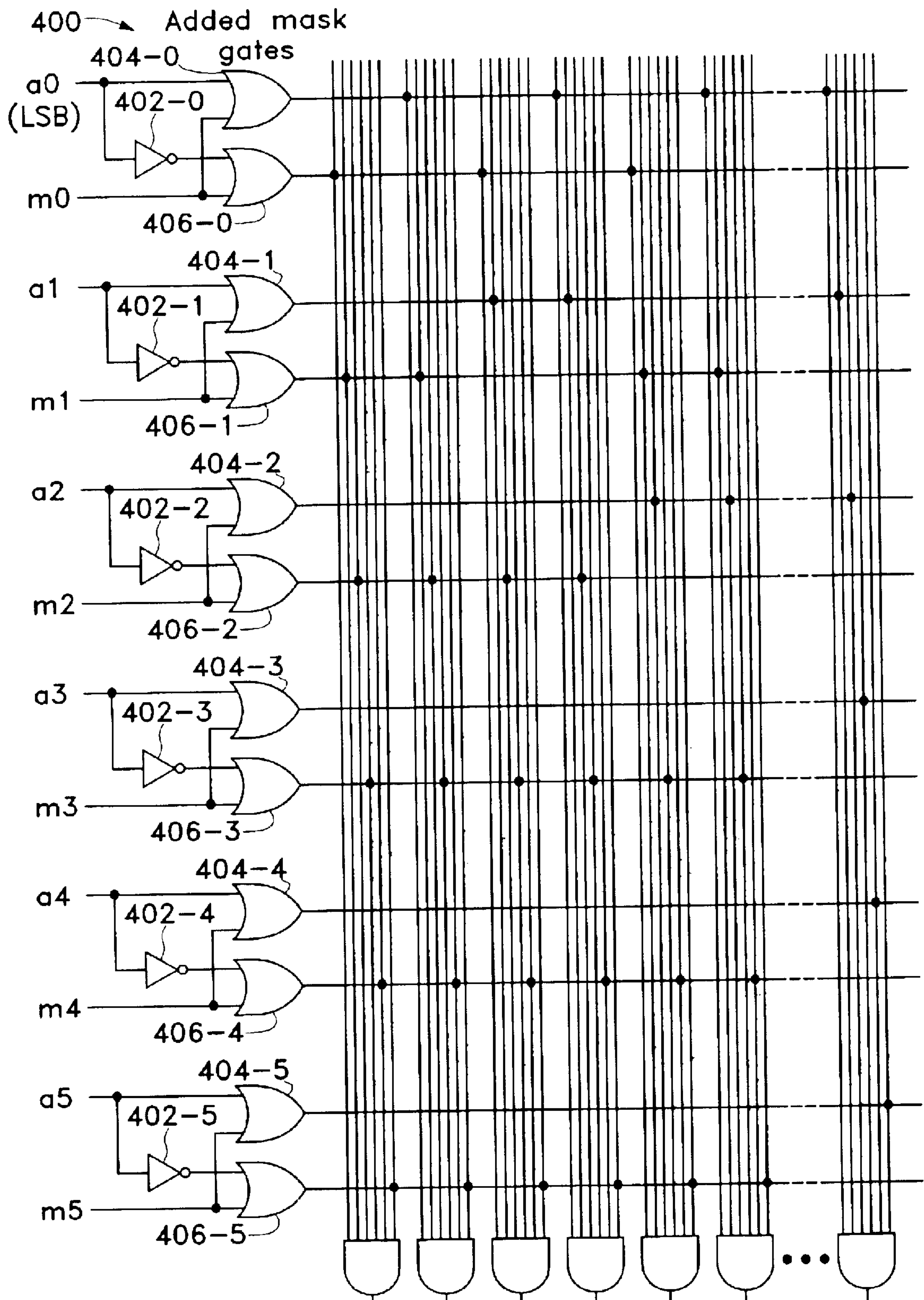
FIG. 4 Decoded row (or column) select signals
