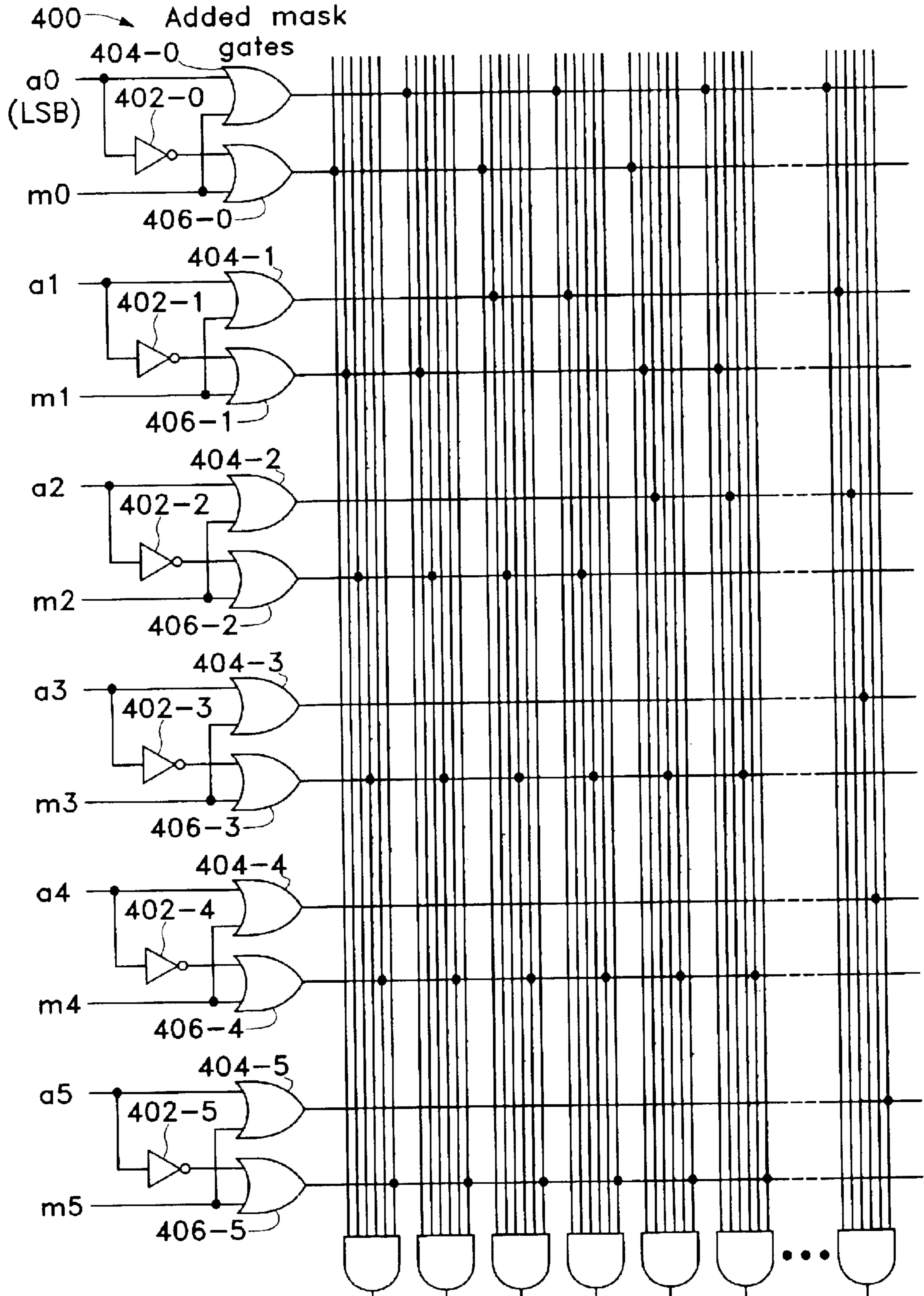
FIG. 4 Decoded row (or column) select signals
