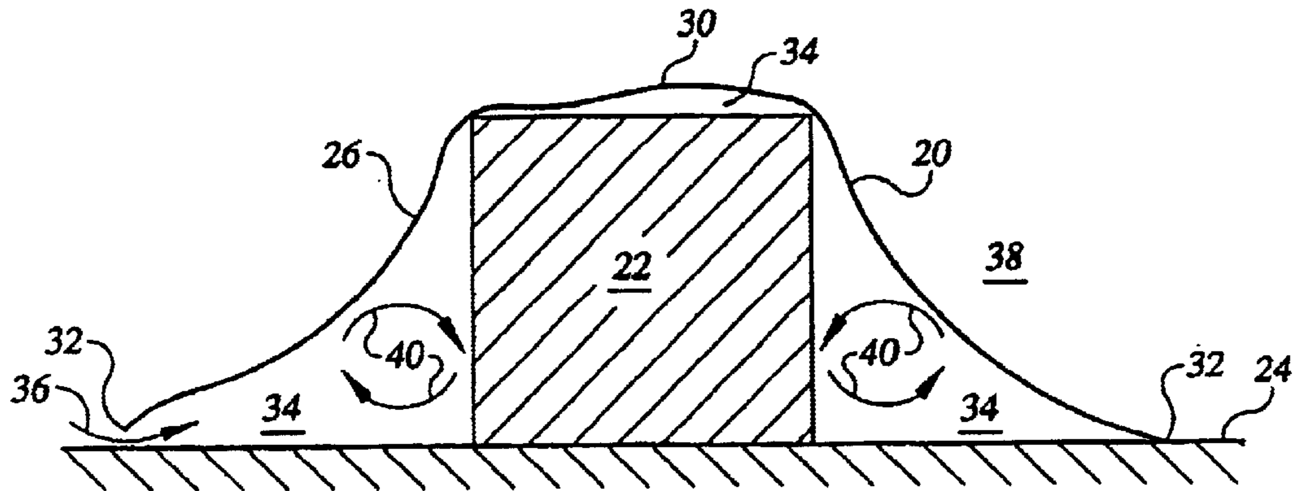
FIG. 1 PRIOR ART
