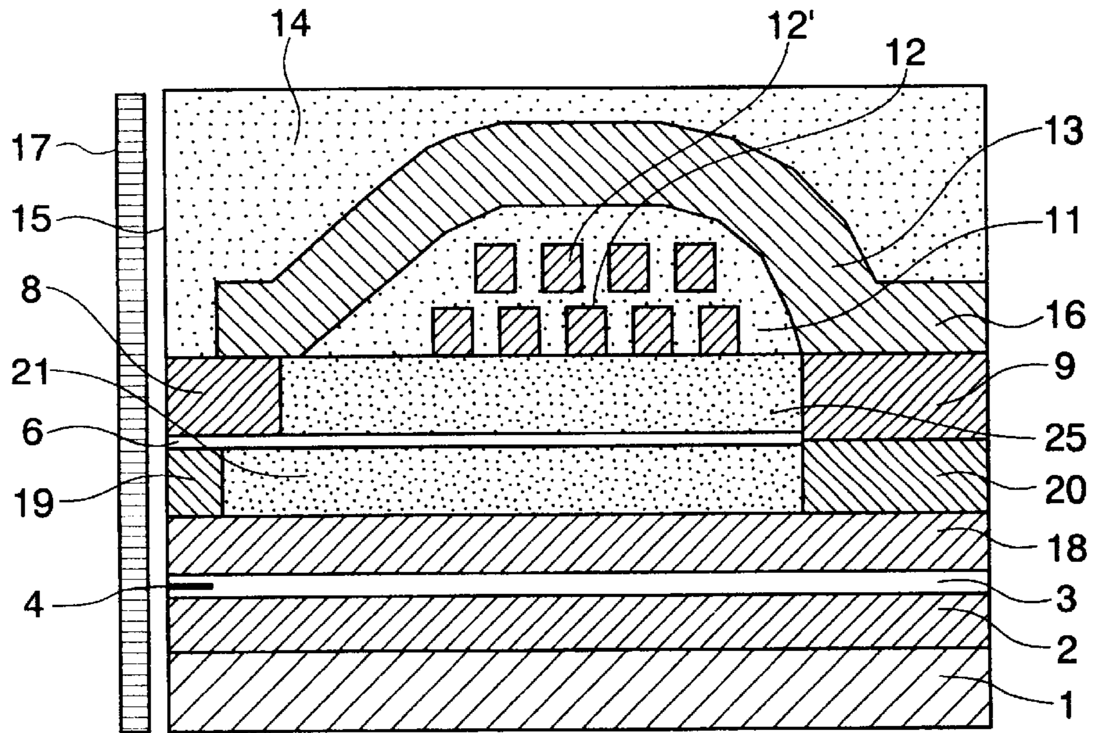
FIG.4 PRIOR ART
