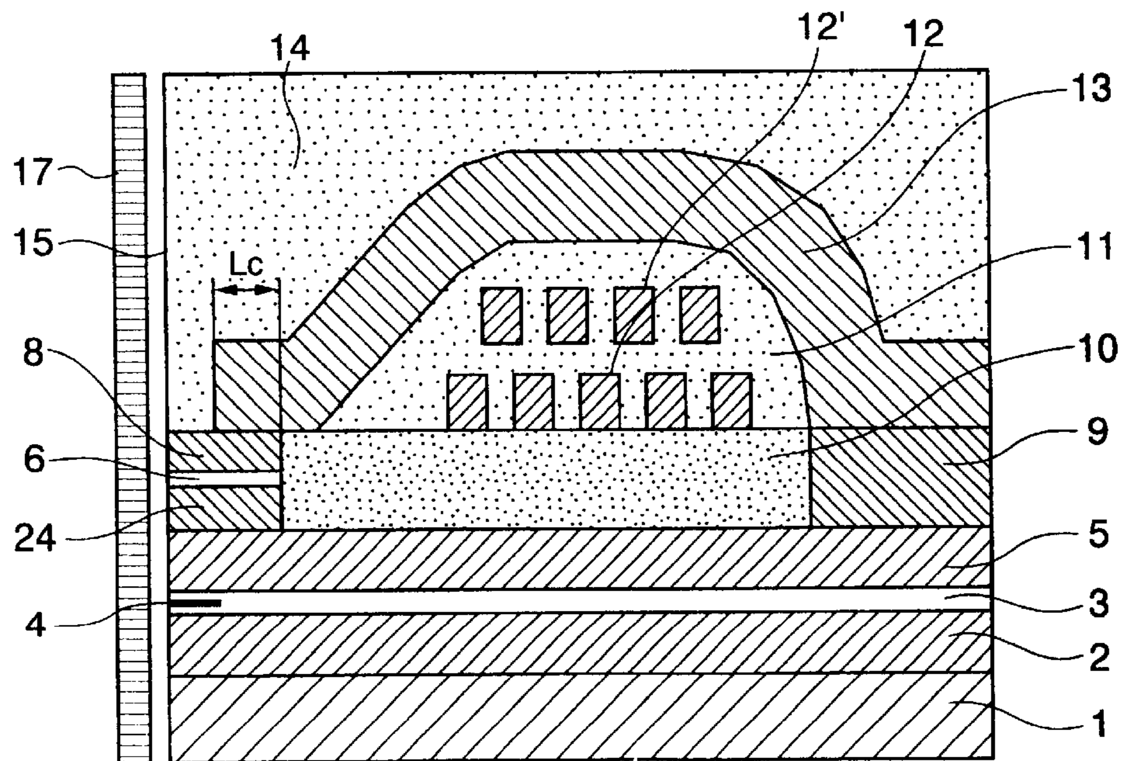
FIG.5 PRIOR ART
