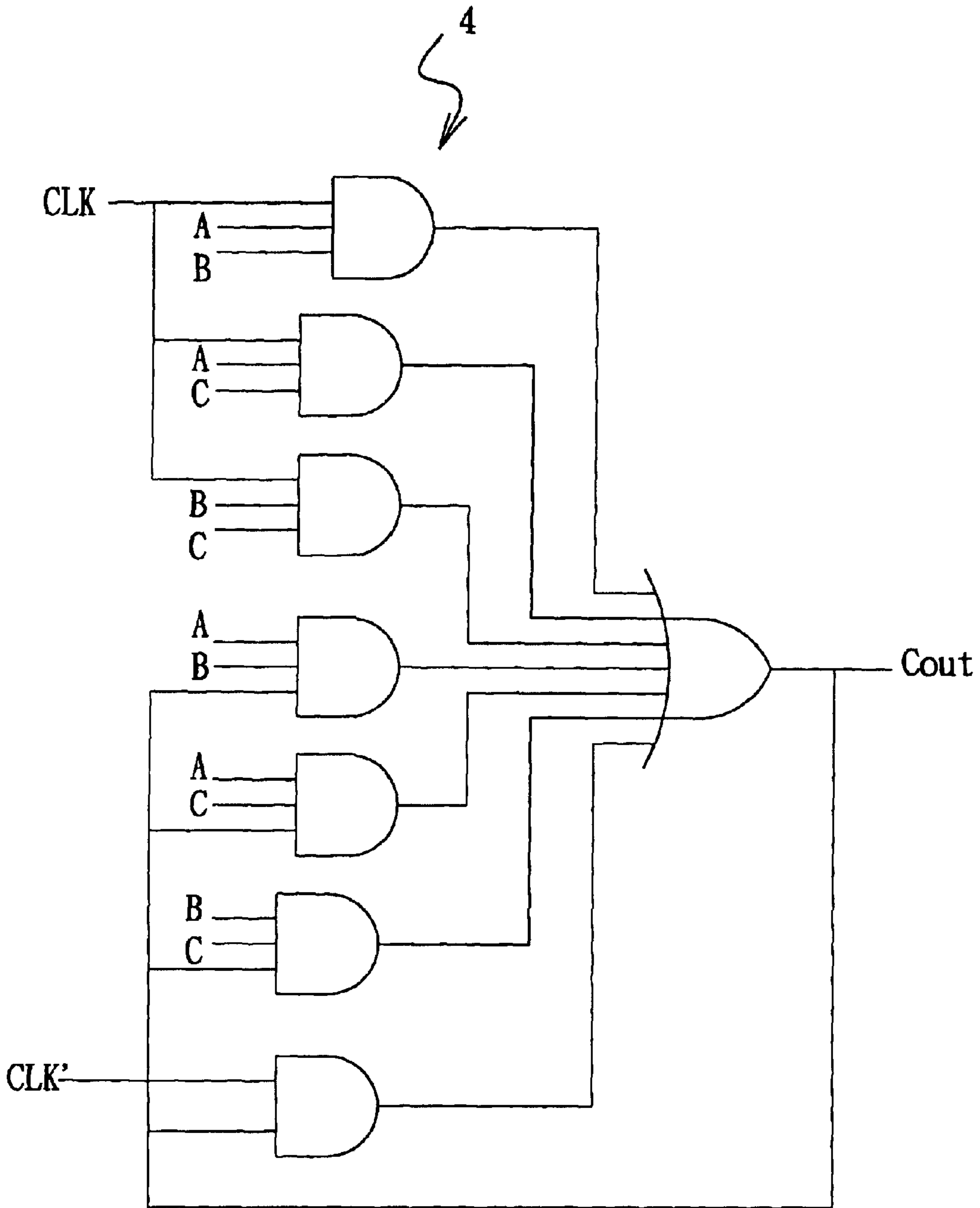
FIG. 3 PRIOR ART
