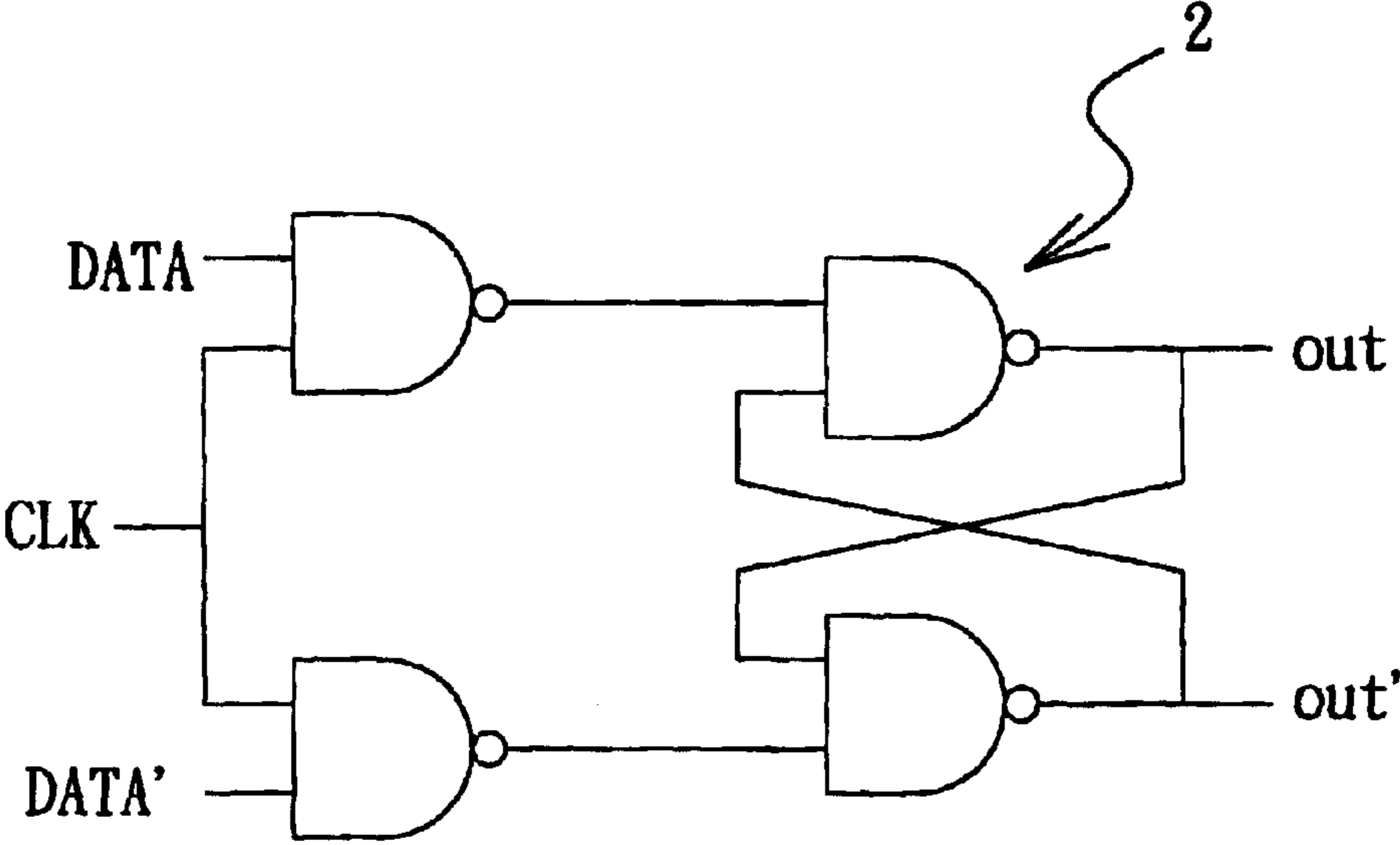
FIG. 1 PRIOR ART
