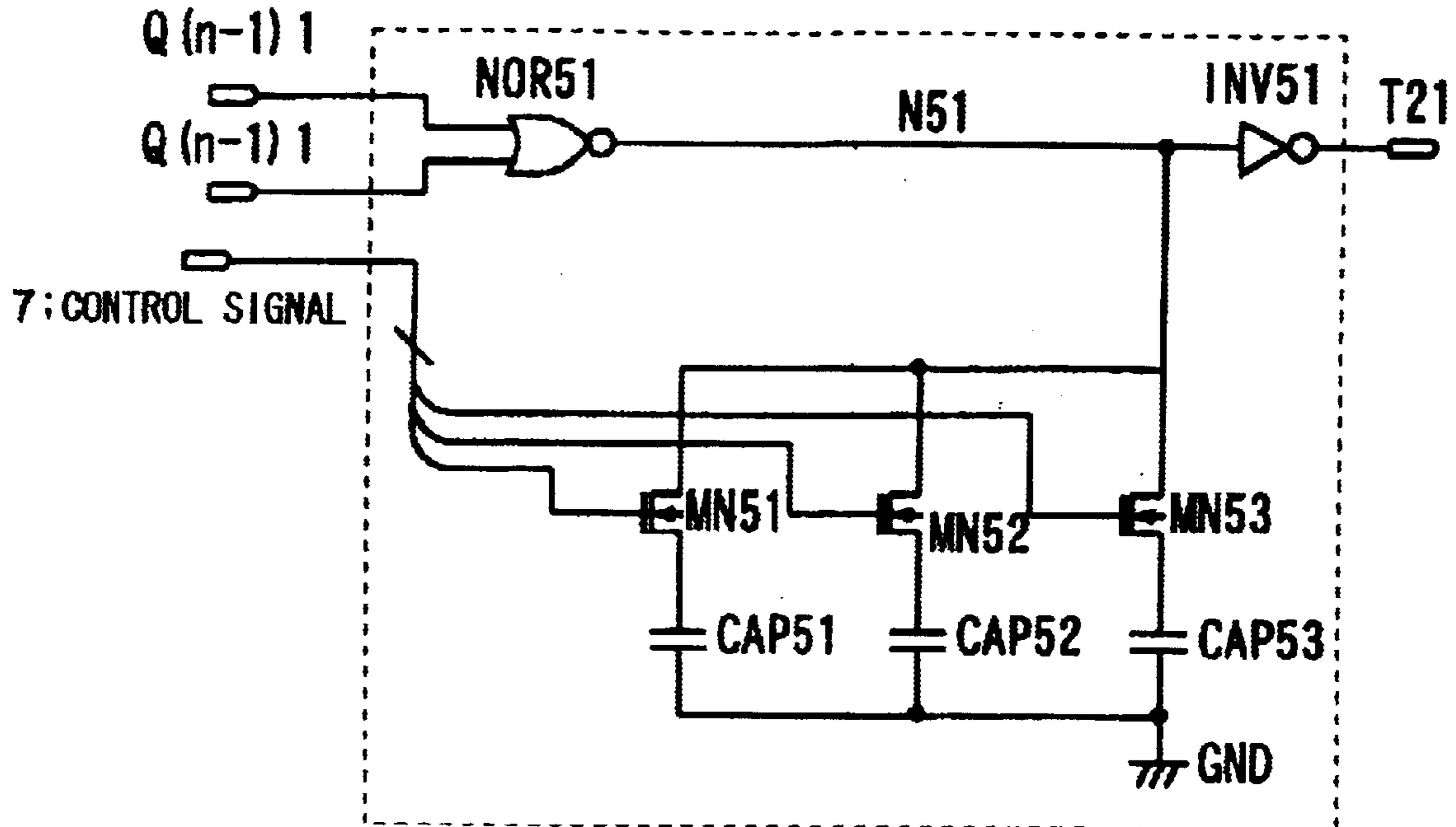
4a1; TIMING DIFFERENCE DIVISION CIRCUIT
