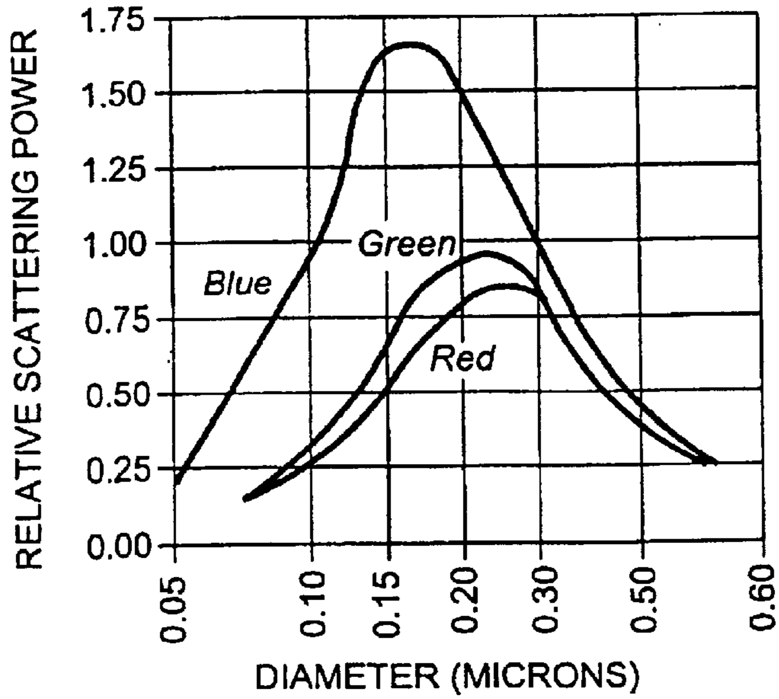
fig. 6 (PRIOR ART)
