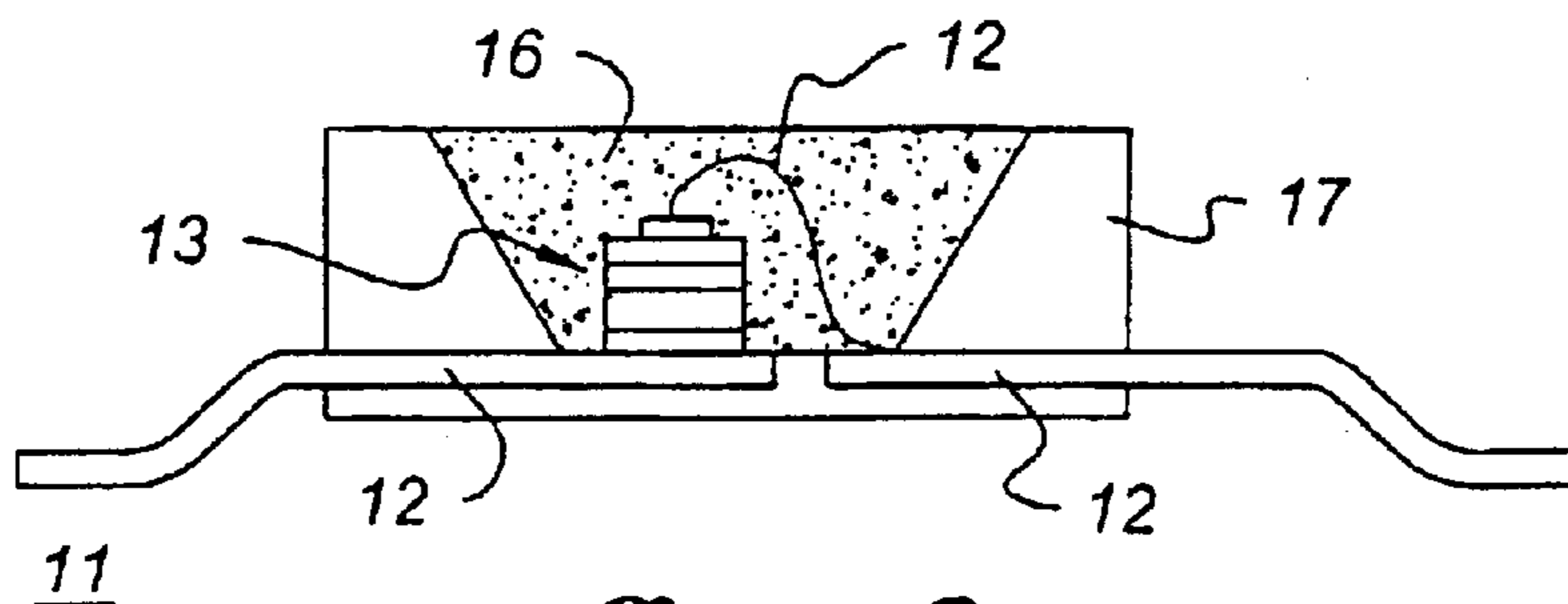
fig. 3 (PRIOR ART)
