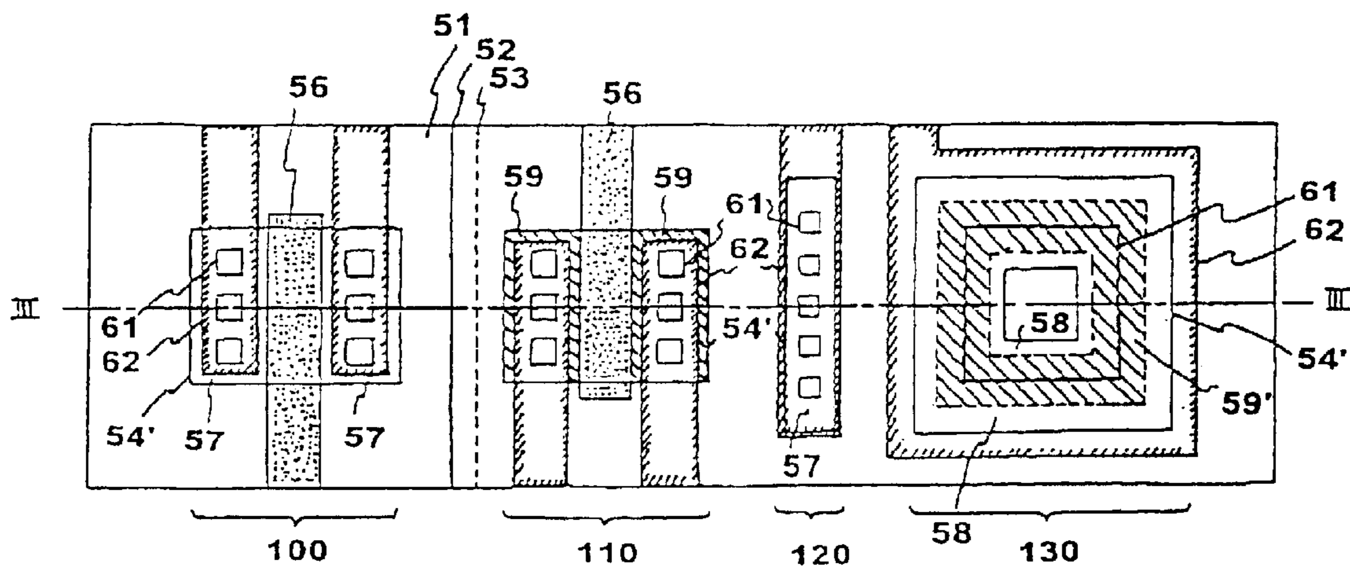
Fig. 5 PRIOR ART
