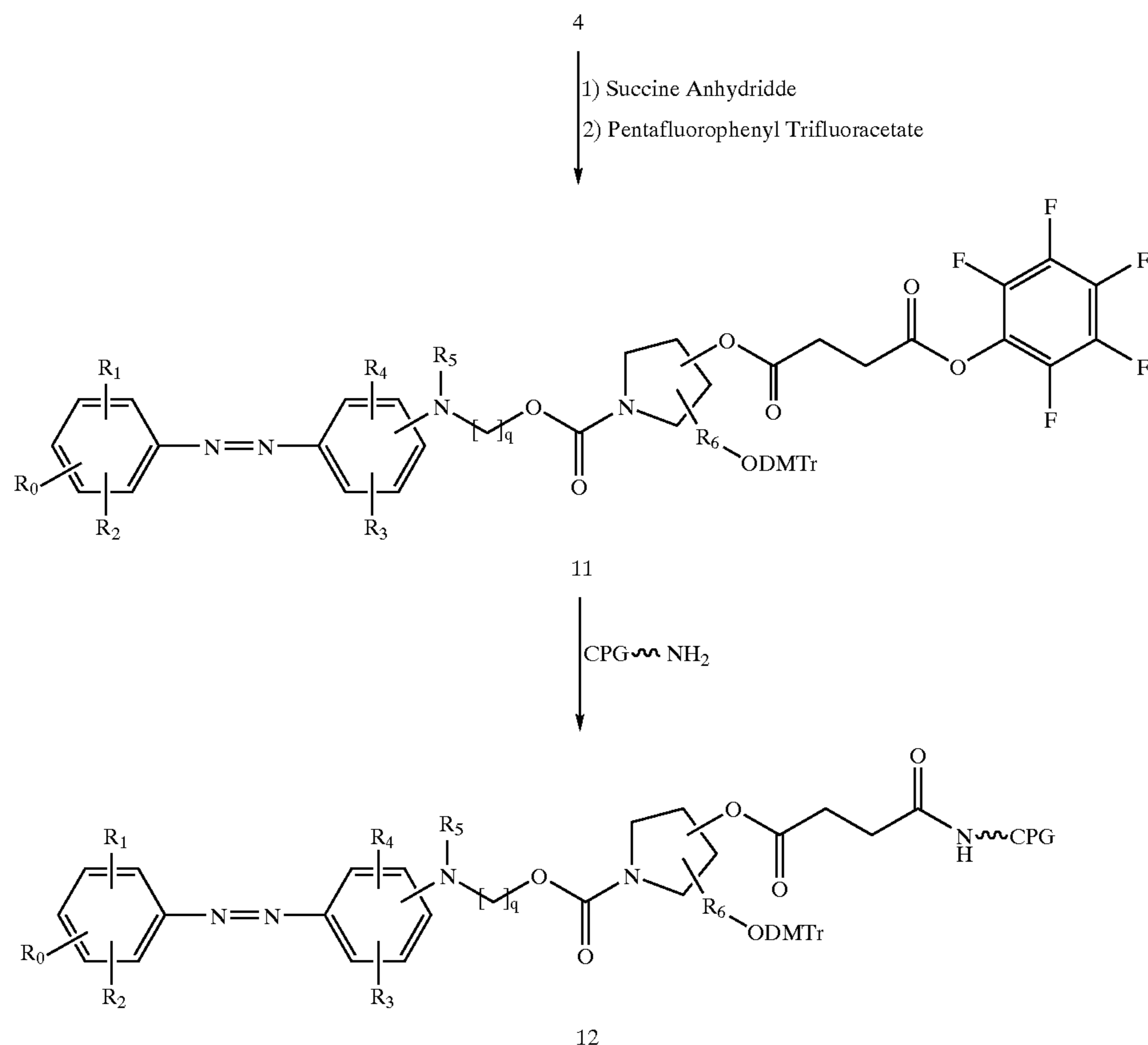
REACTION SCHEME 3
