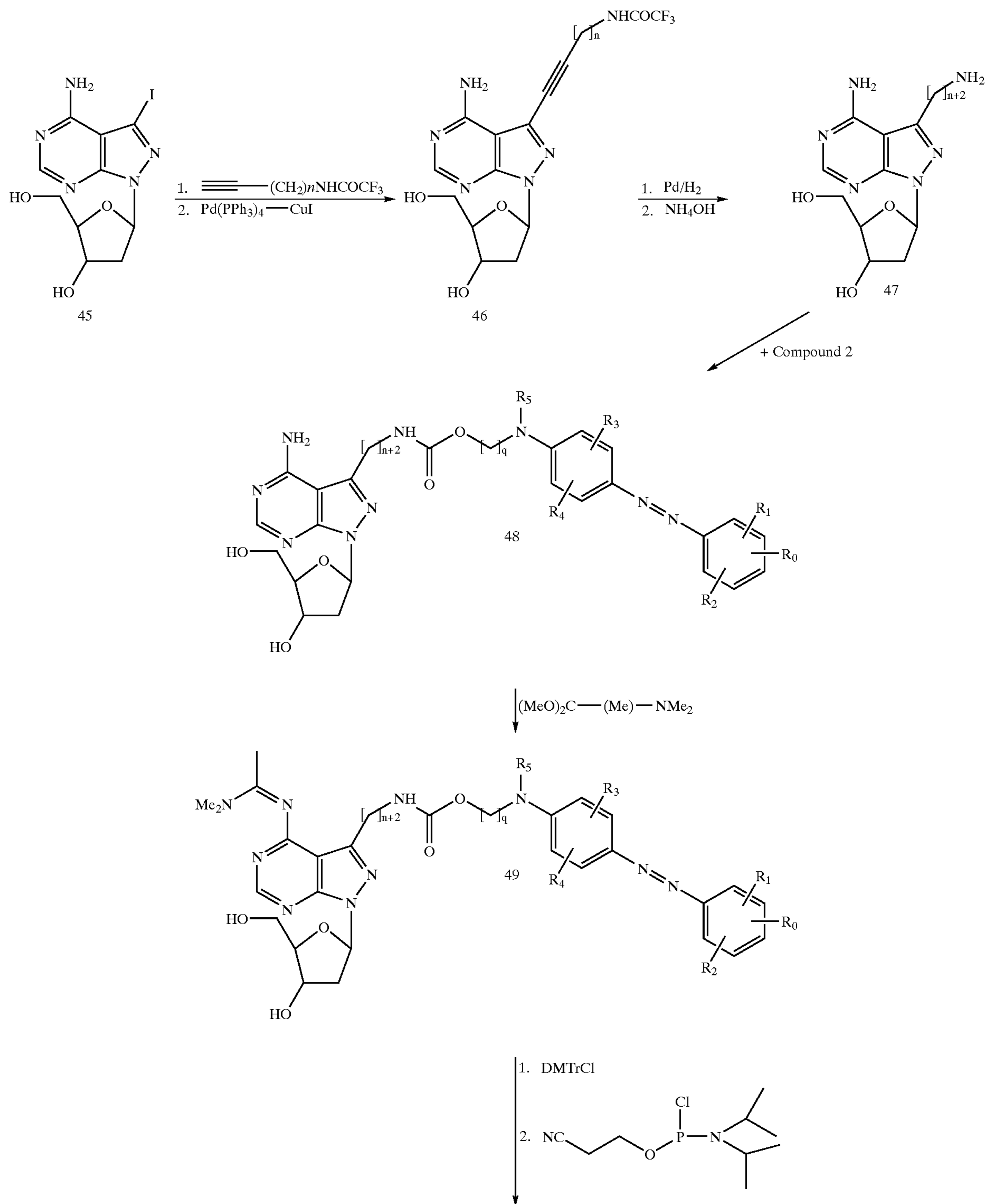
REACTION SCHEME 11
