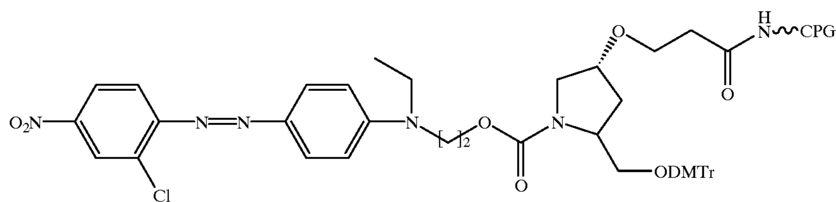
RED 13-pyrrolidine-DMTr-CPG, 12
