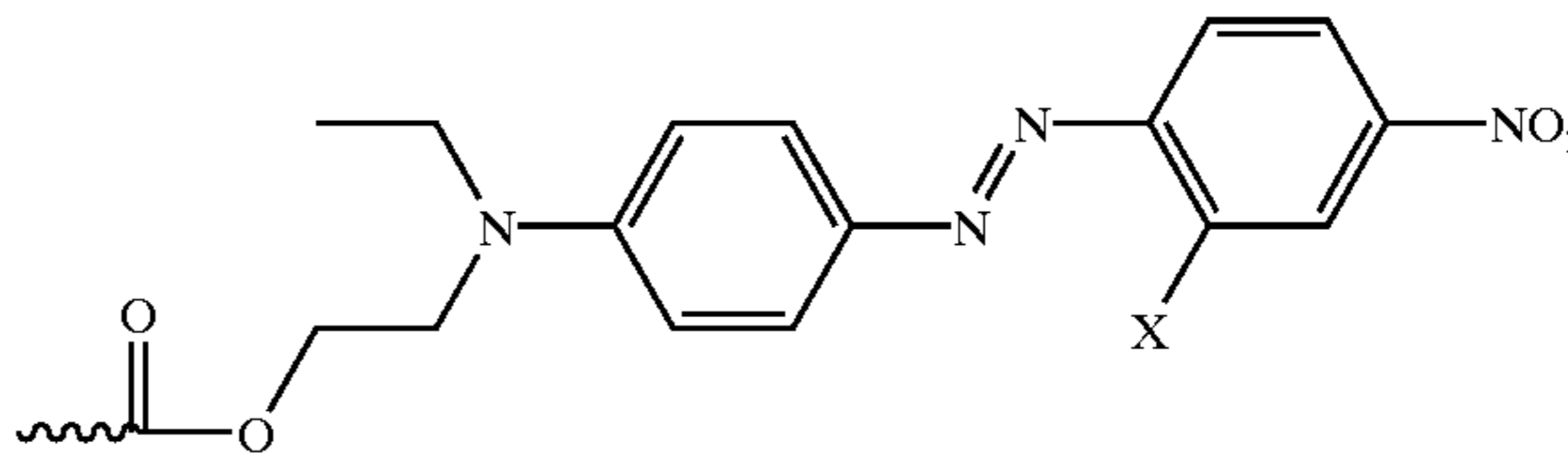
Formulas 17 to 18
