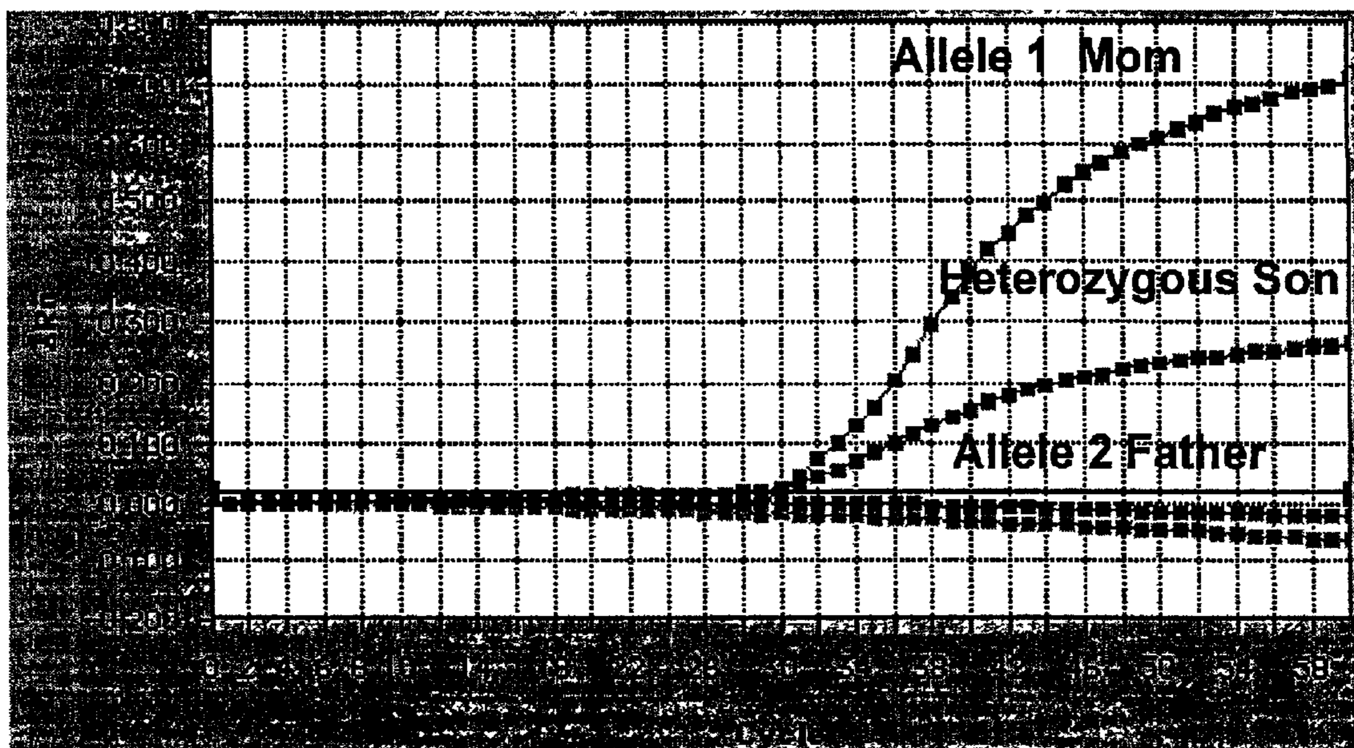
Figure 5. Real-time detection of RRM1 allele 1 (T/C mismatch) with a non-cleavable MGB-Q-ATA TCT AGC GTT GA-F1 (30) where t=v=m=3 , R_0=4\text{-NO}_2 , R_1=2\text{-Cl} , R_2=R_3=R_4=H and F1=fluorescein.
