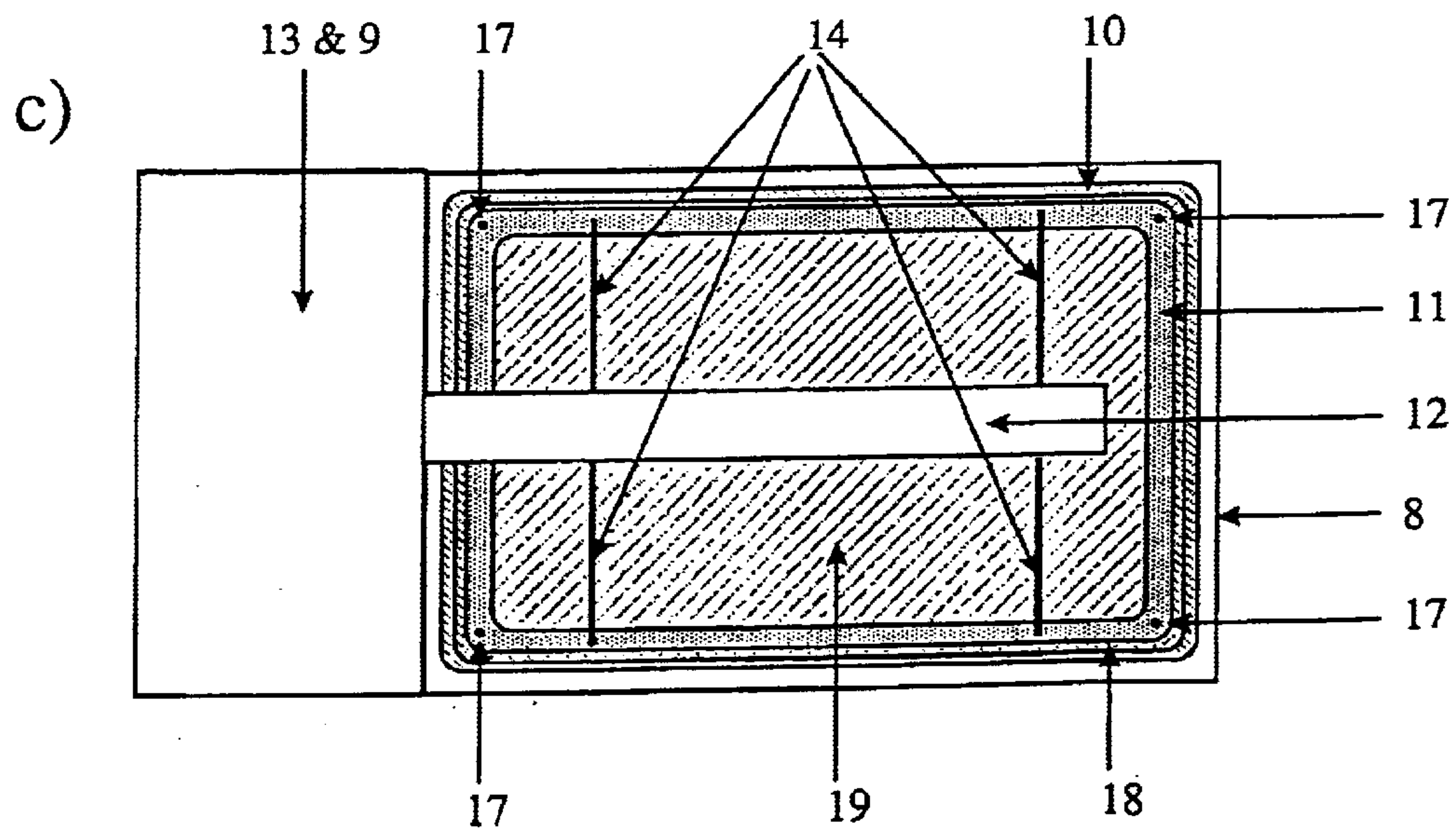
Top view of test stage; not to scale
