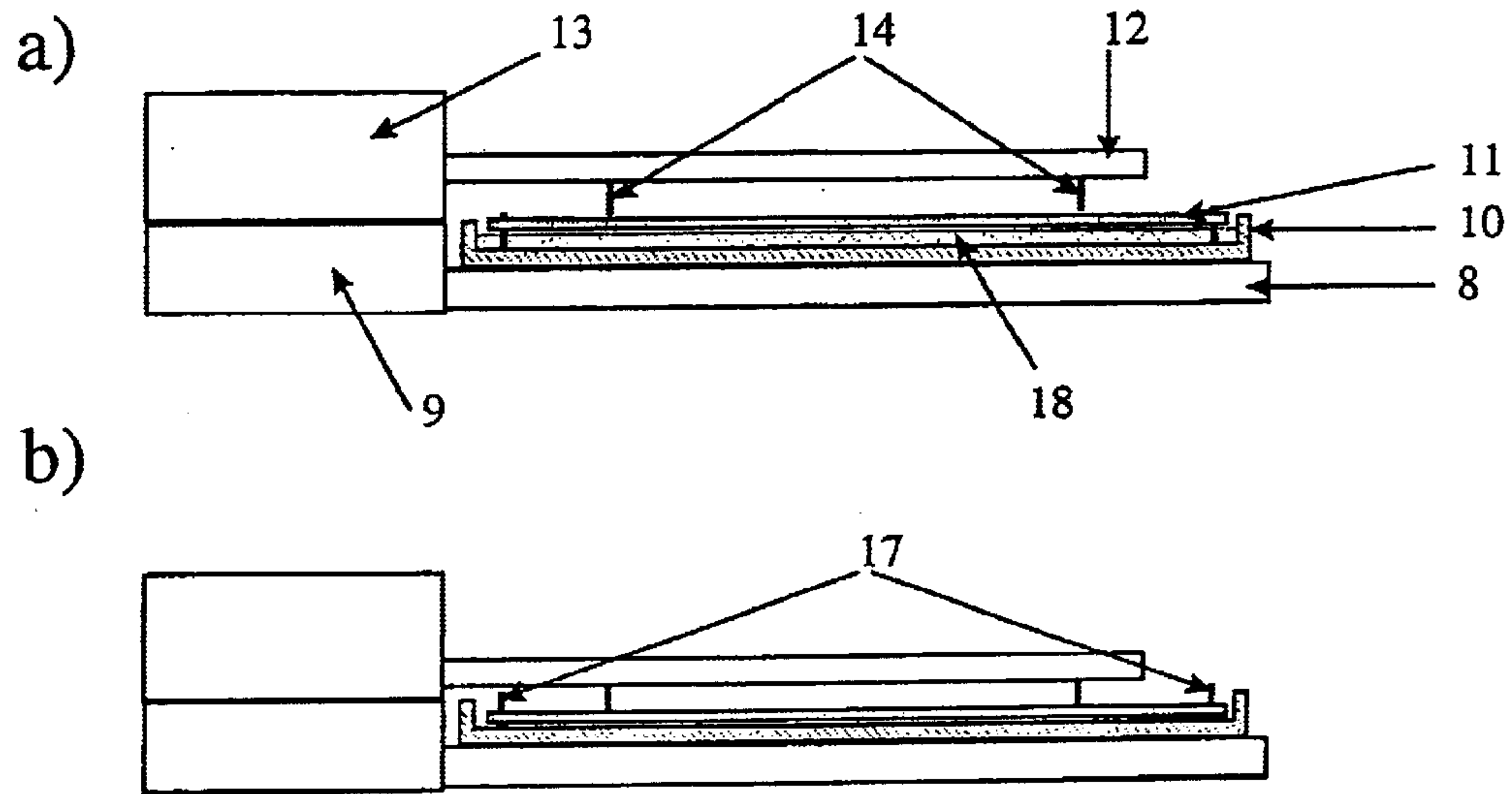
Side views of test stage; not to scale
