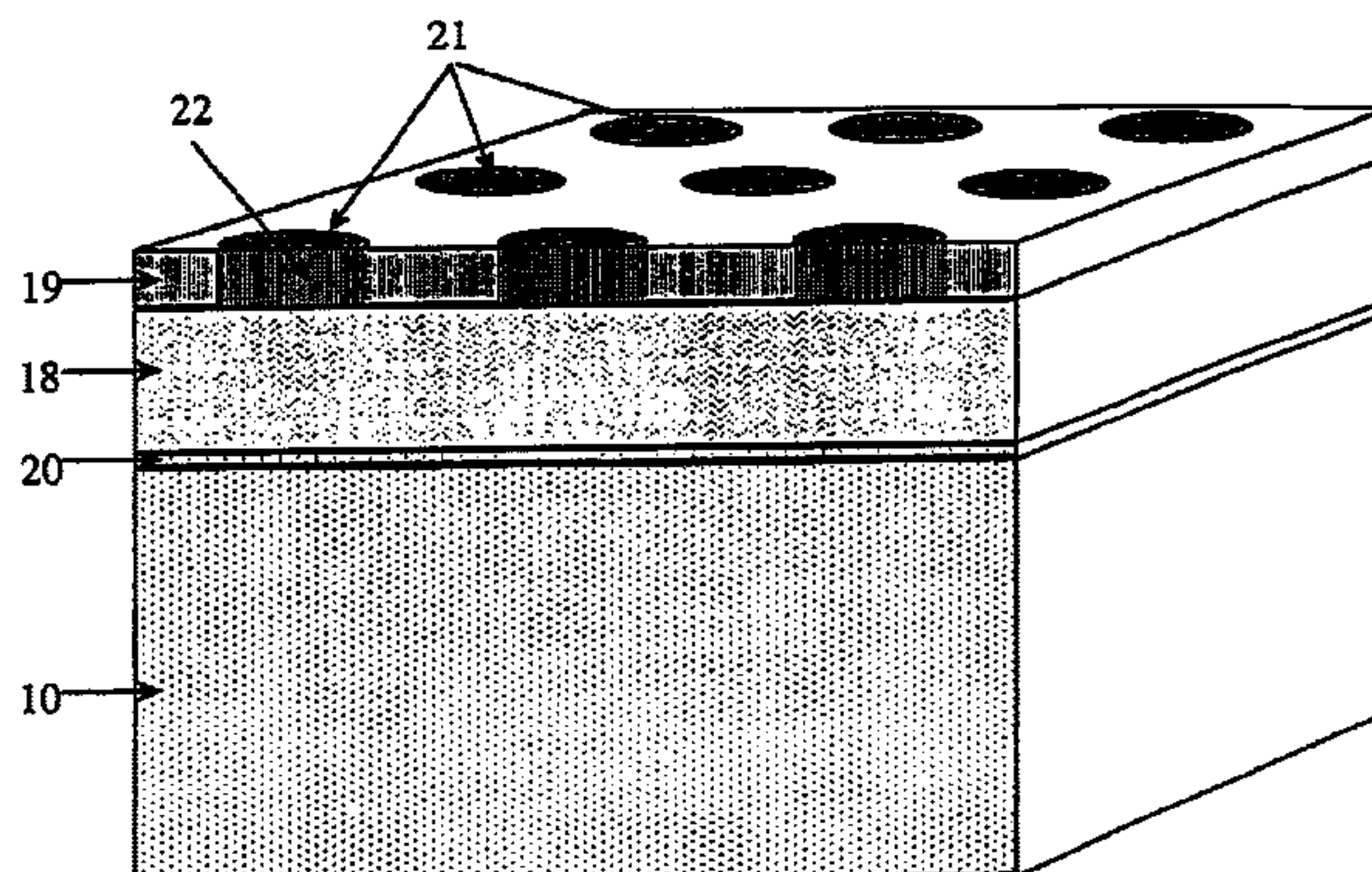
3-D sectional representations of portions of the test-array/detector layers: not to scale
