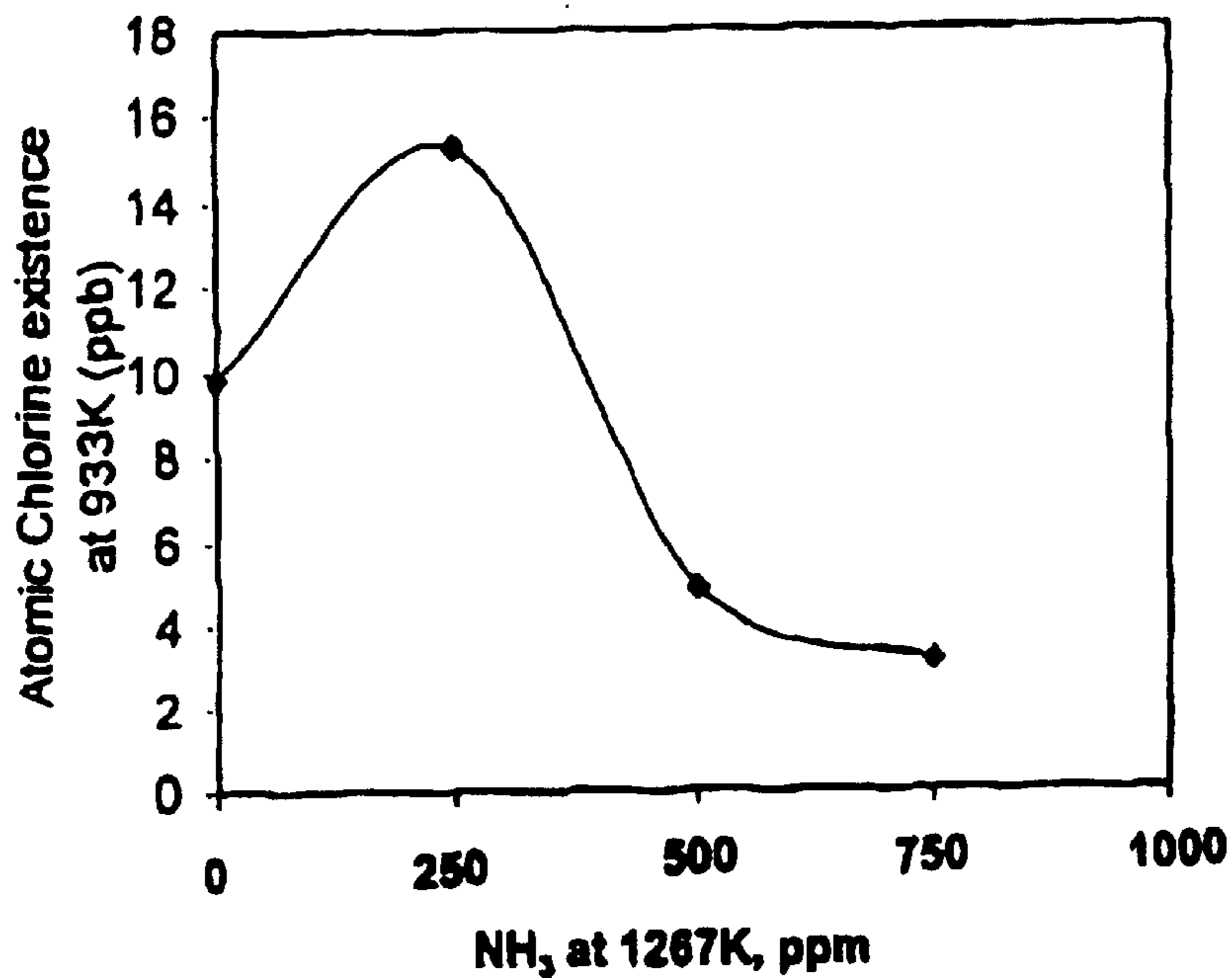
NH 3 injection effect on the Atomic Chlorine existence
