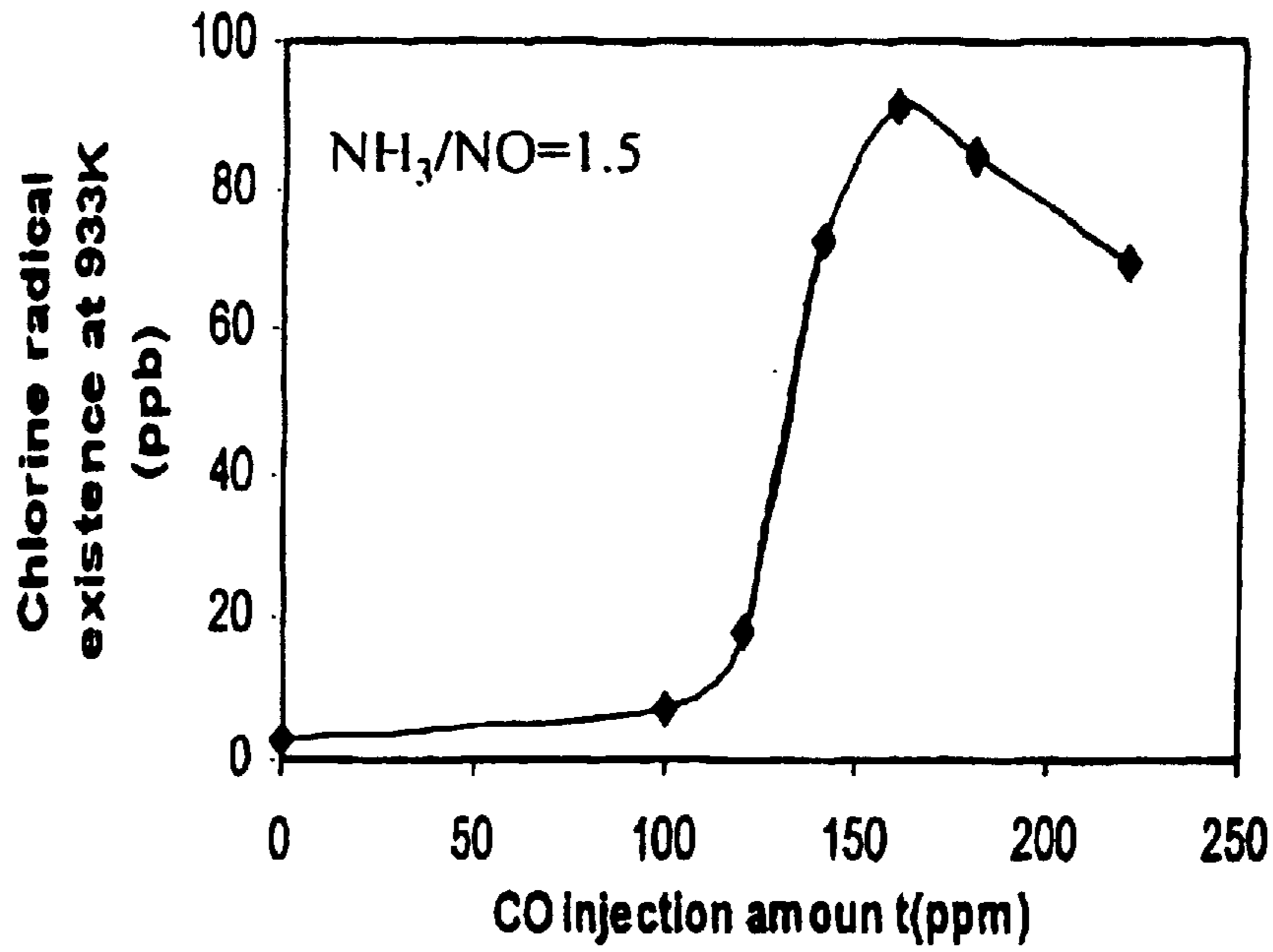
CO local Conc. in the SNCR injection zone effect on the Atomic Chlorine existence
