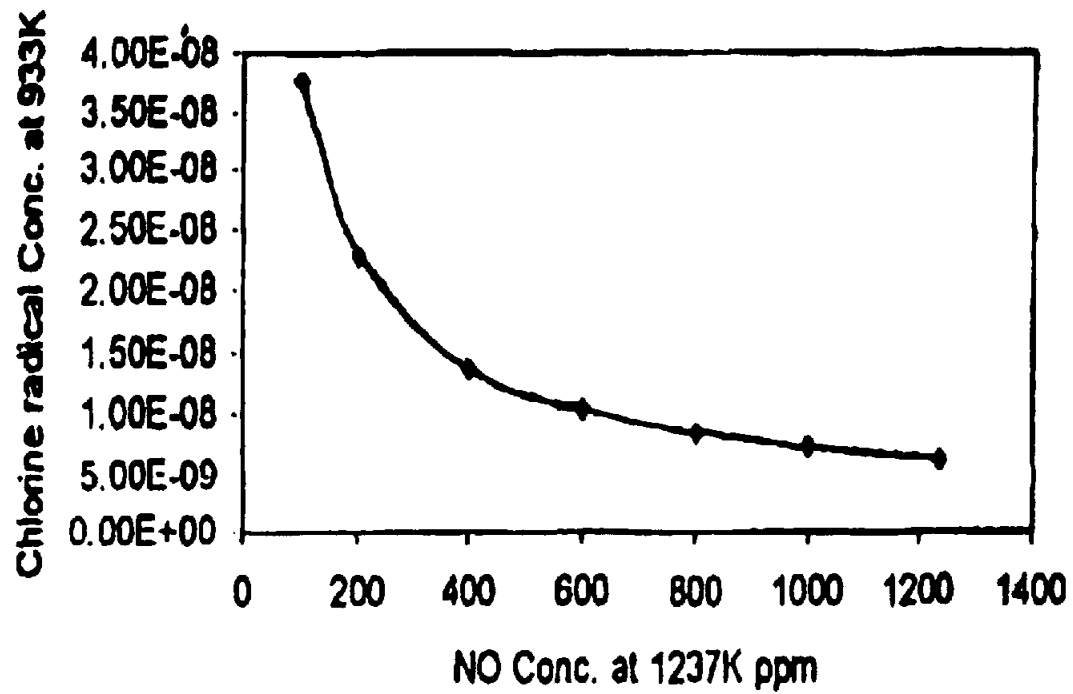
NO Conc. Effect on the Chlorine radical existence
