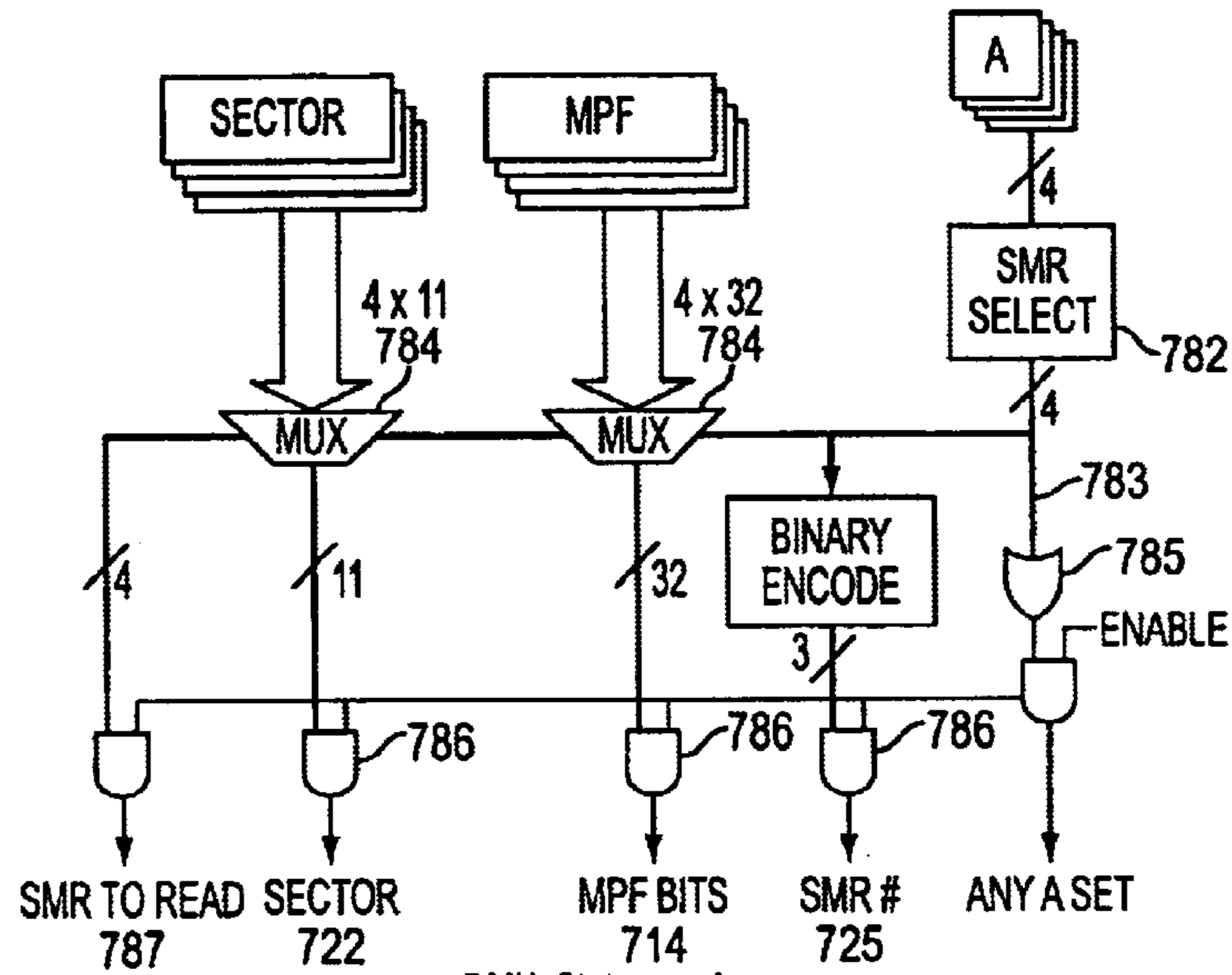
DMU_Status read FIG. 7H
