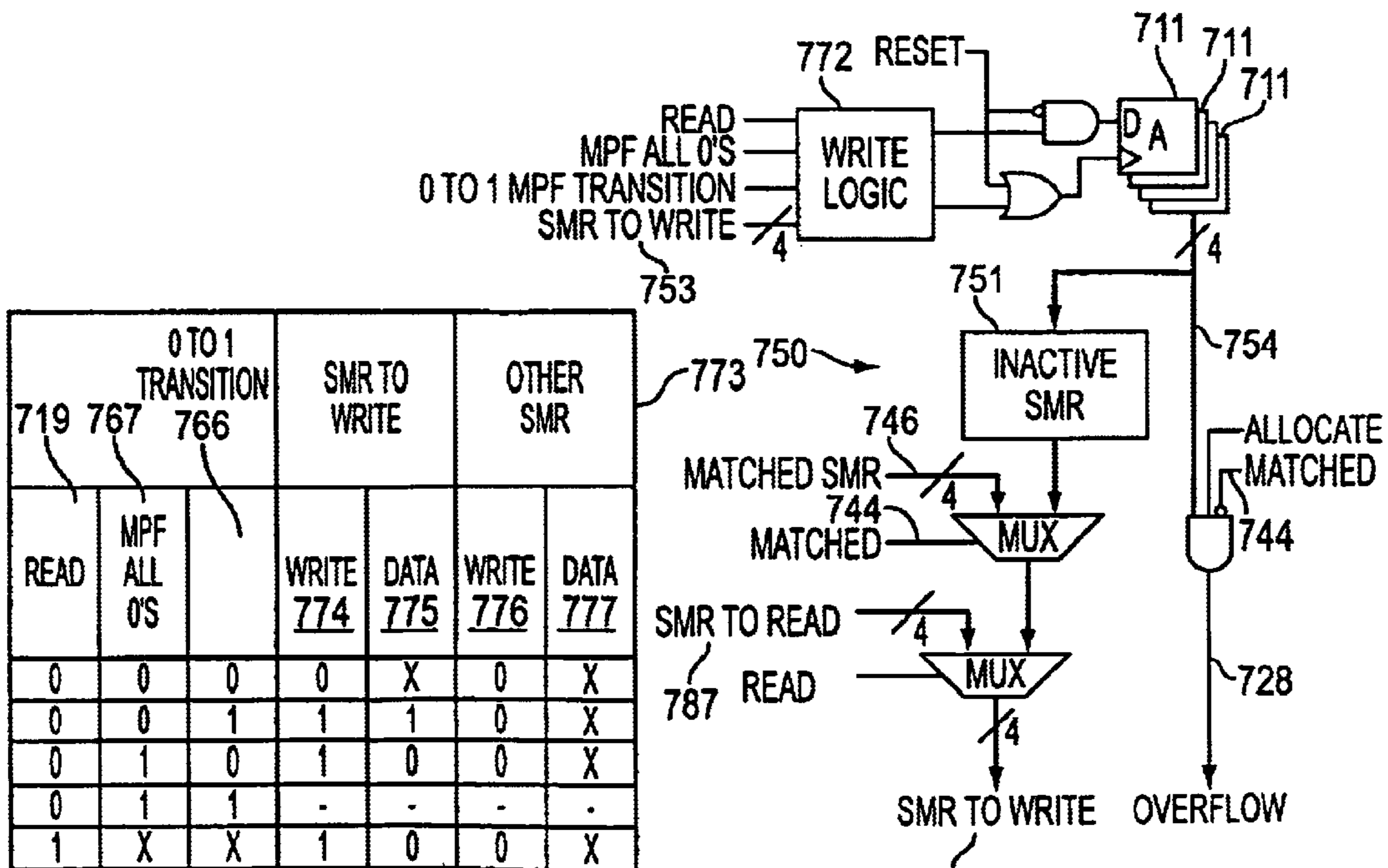
SMR Allocation logic FIG. 7F
