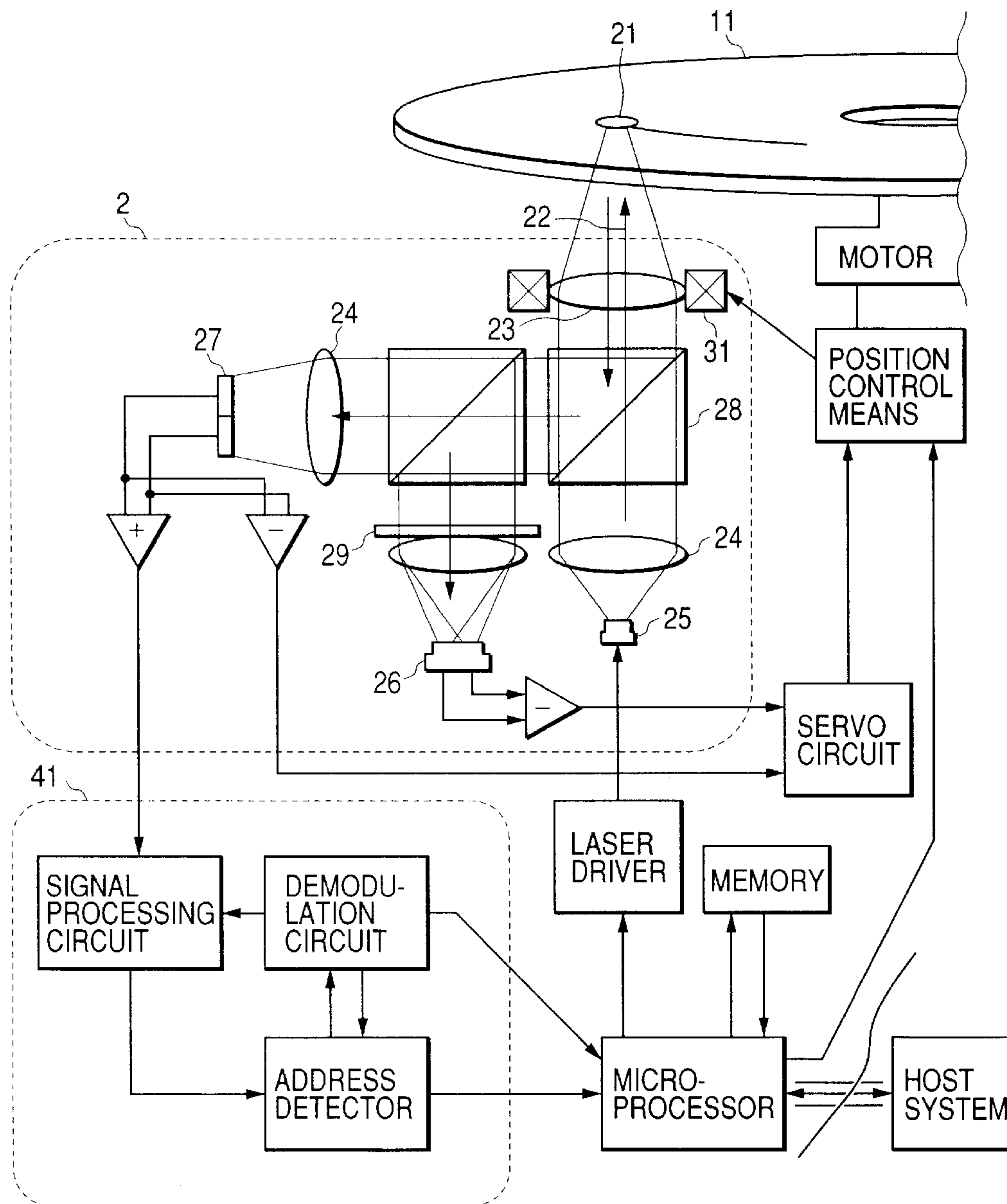
FIG. 3 - PRIOR ART
