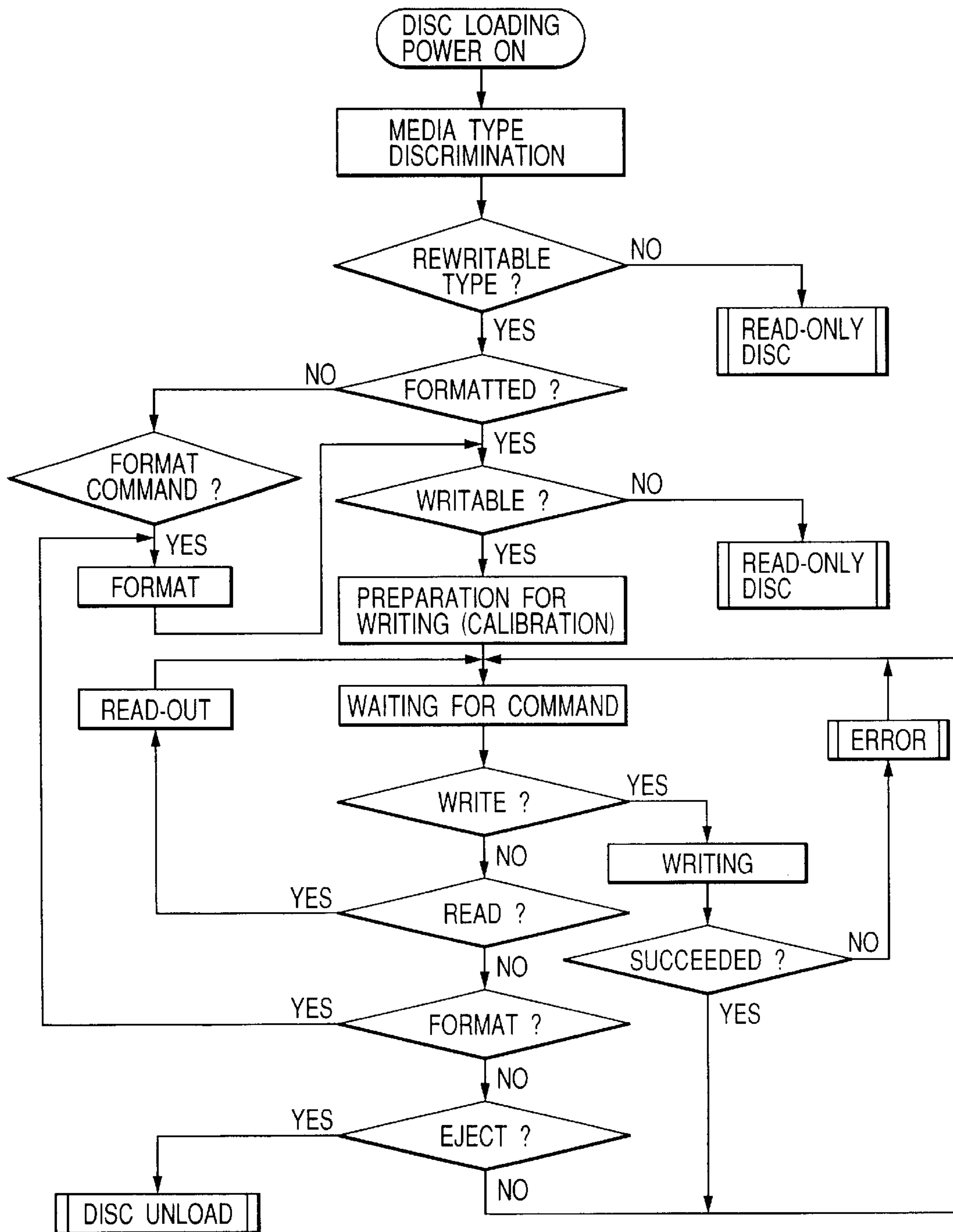
FIG. 5 - PRIOR ART
