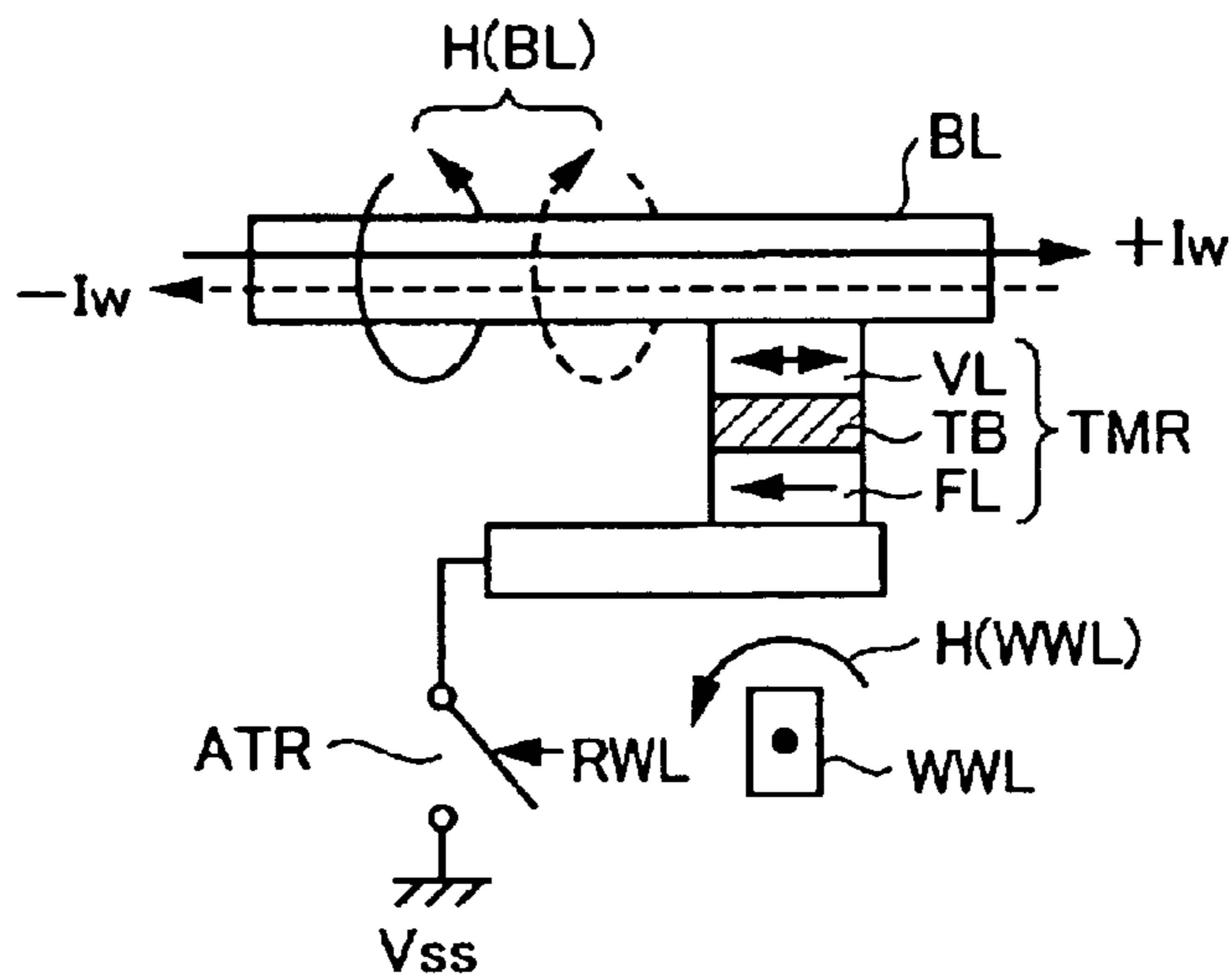
FIG.68 PRIOR ART
