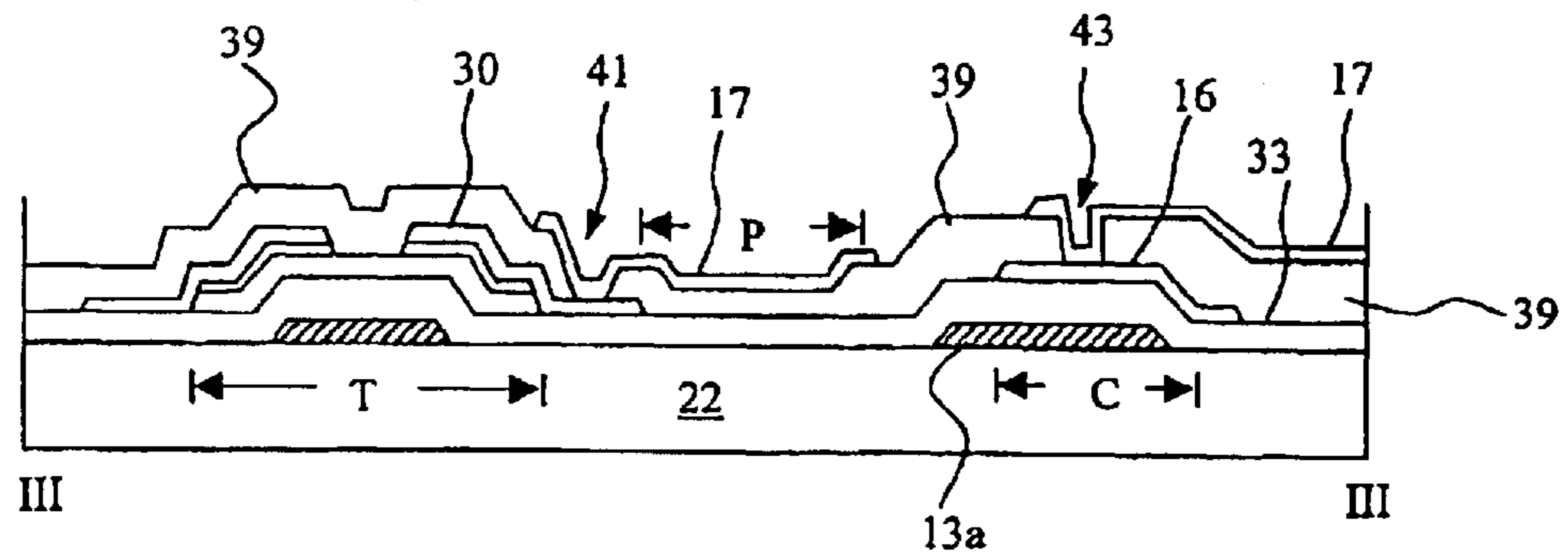
FIG. 3J (RELATED ART)
