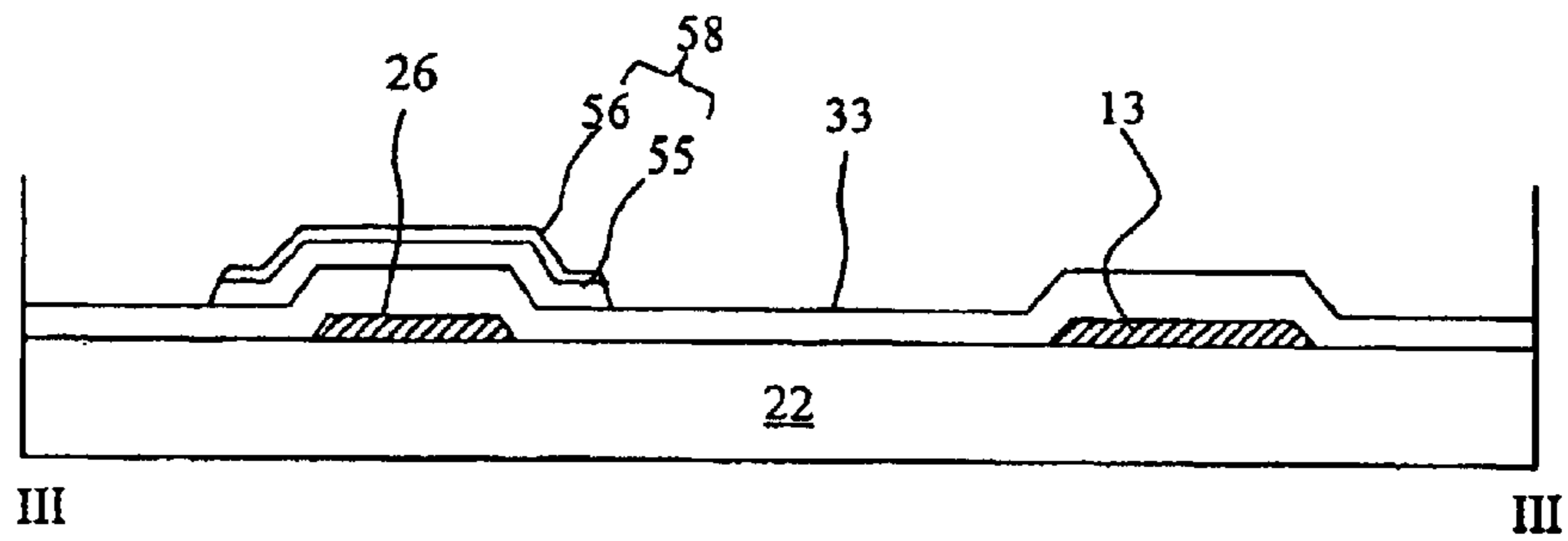
FIG. 3D (RELATED ART)
