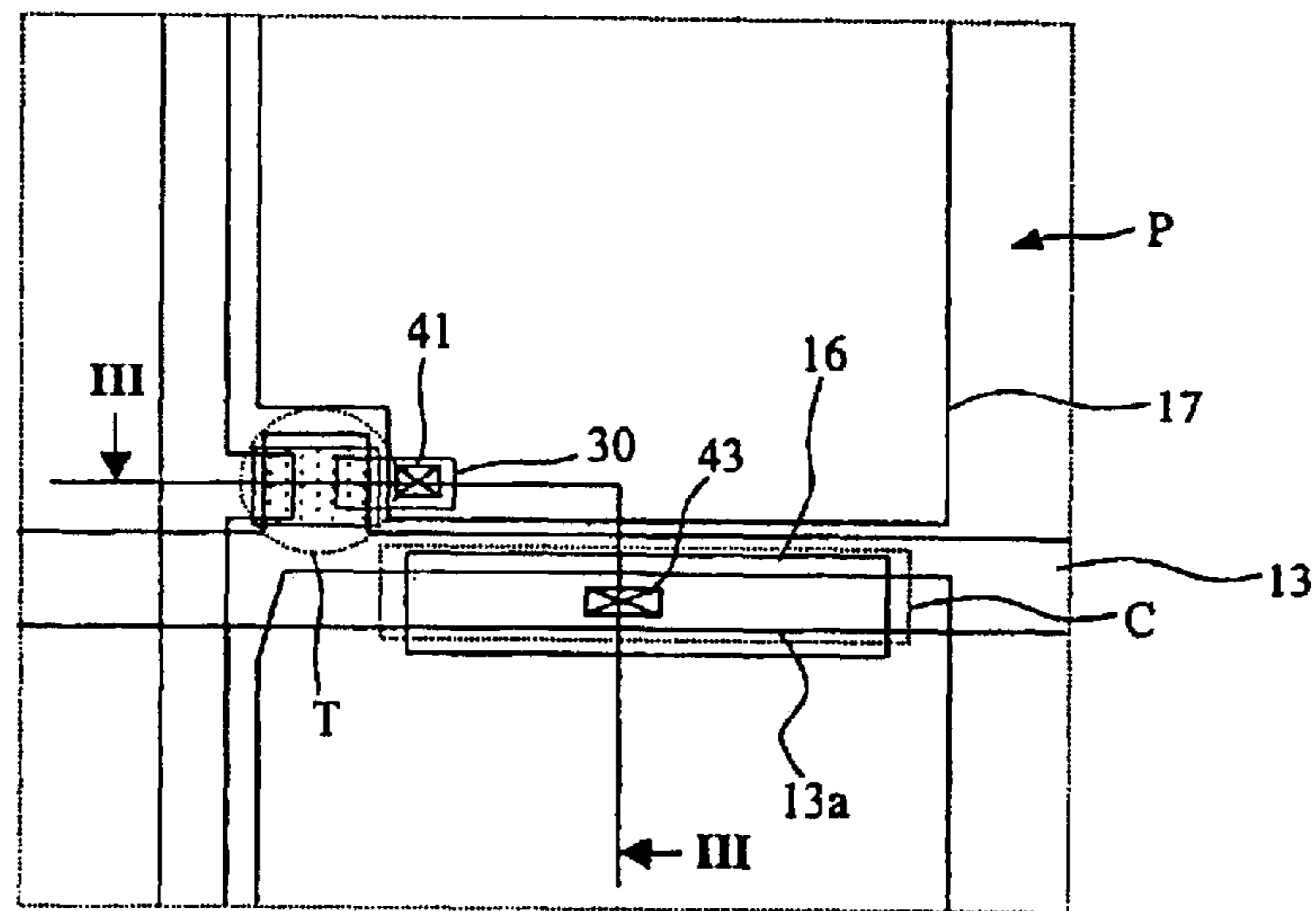
FIG. 3J (RELATED ART)
