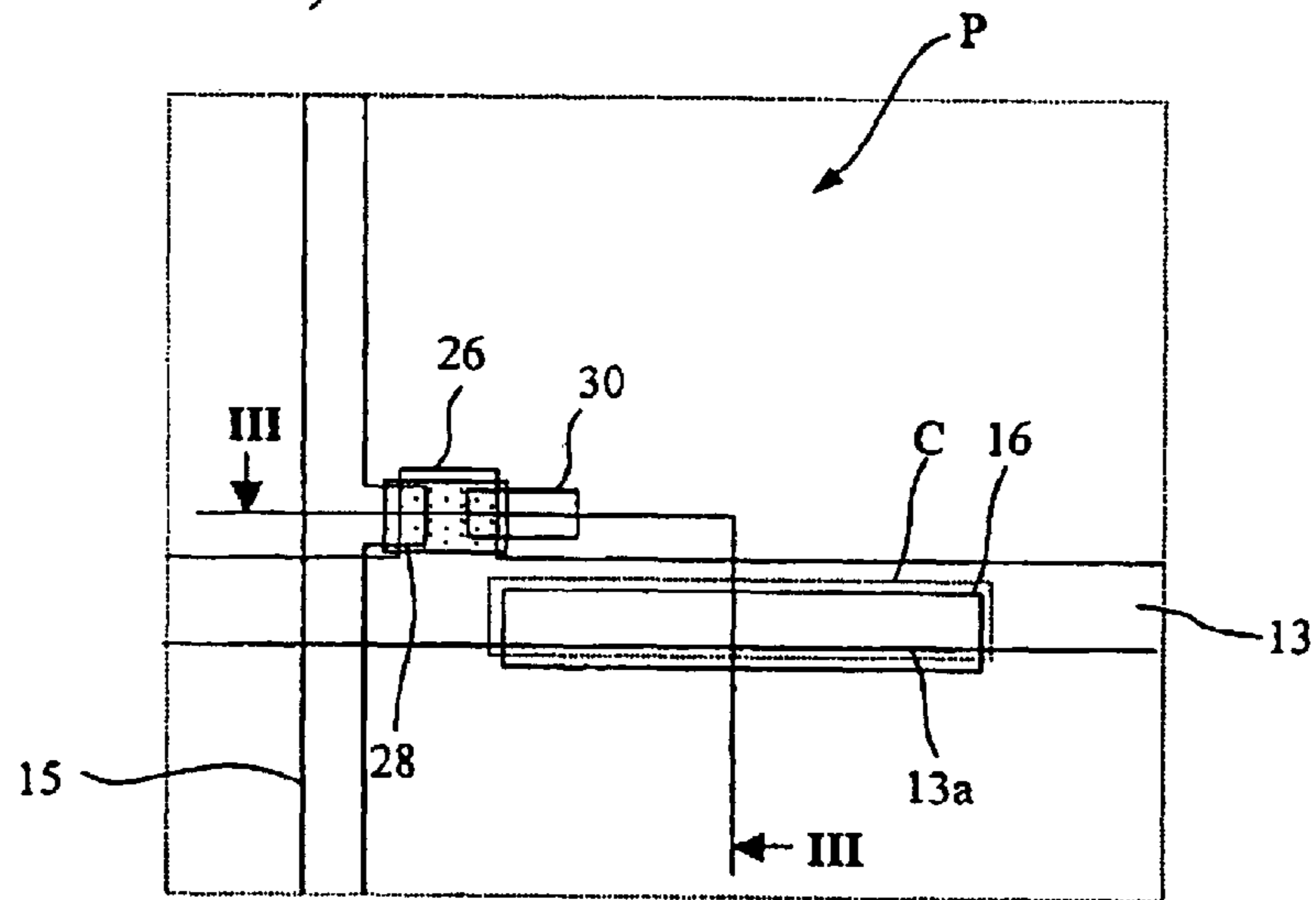
FIG. 3E (RELATED ART)
