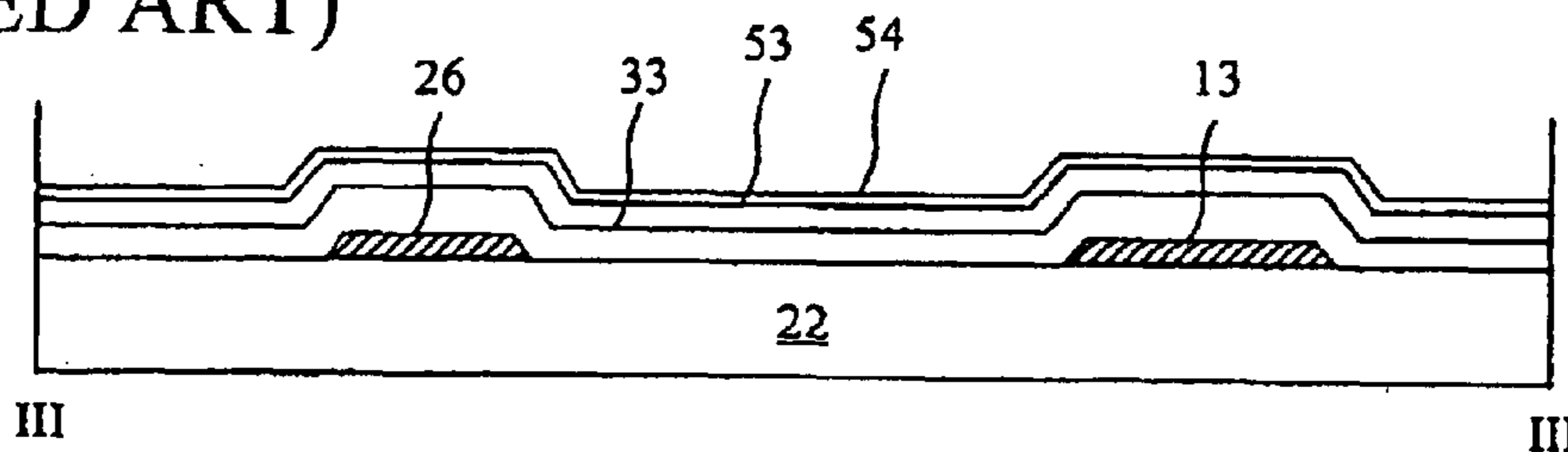
FIG. 3B (RELATED ART)
