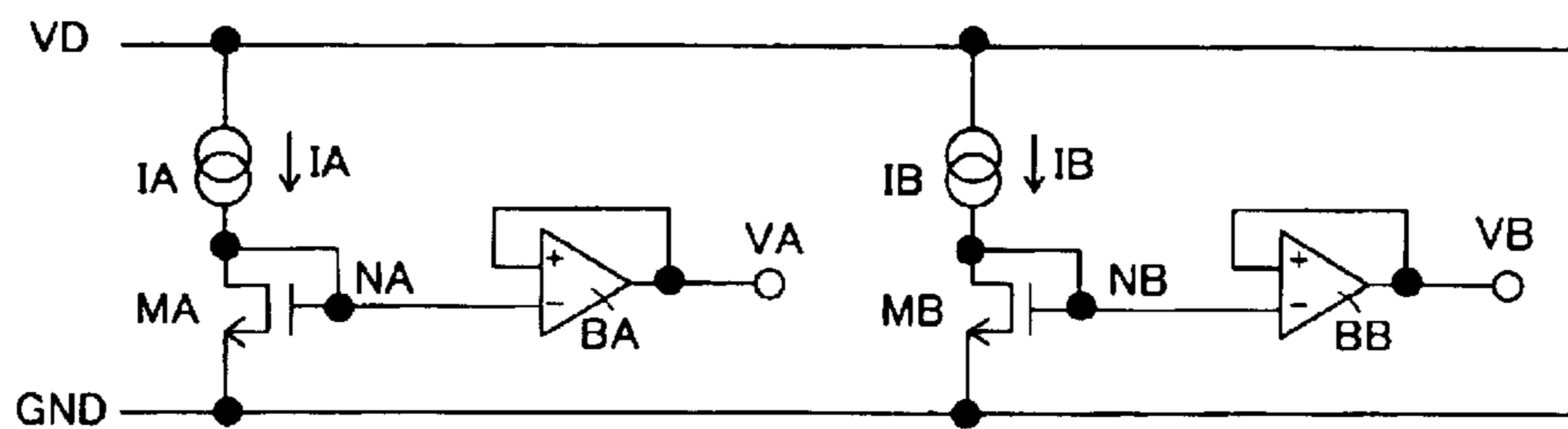
CIRCUIT DIAGRAM OF BIAS VOLTAGE GENERATOR CIRCUIT
