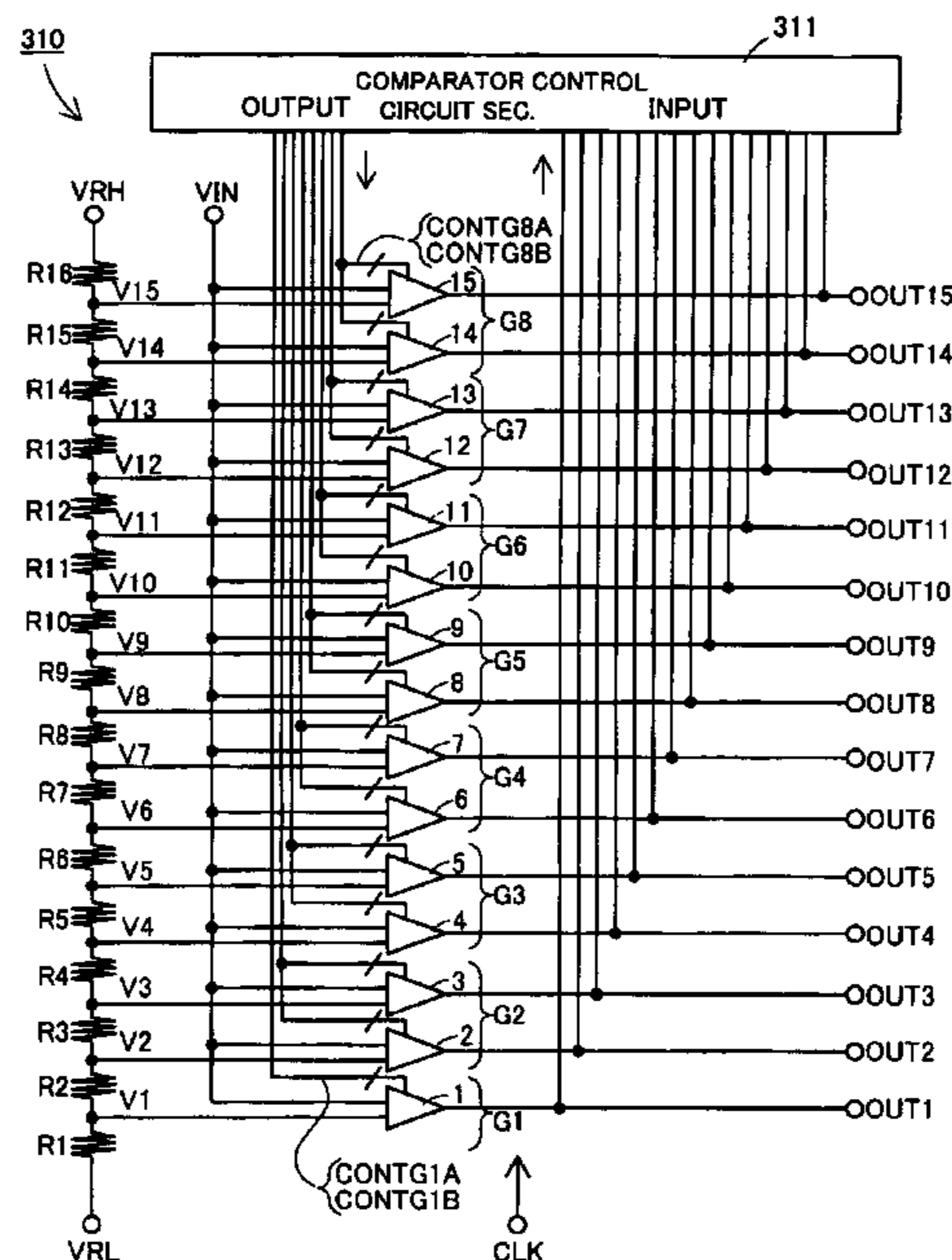
EXPLANATORY VIEW SHOWING OUTLINE OF COMPARISON SECTION OF A/D CONVERTER CIRCUIT DIRECTED TO EMBODIMENT 3
