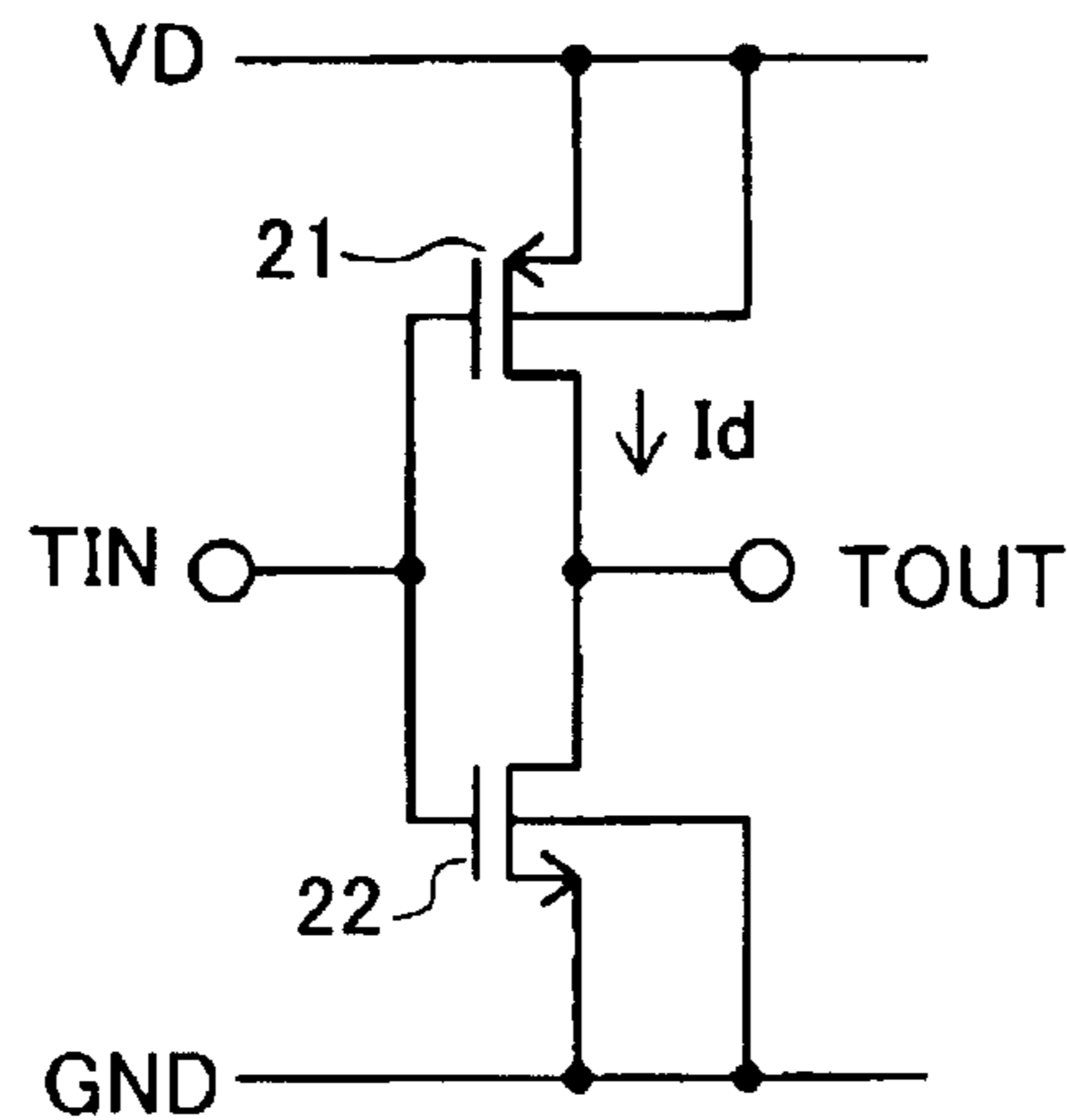
CIRCUIT DIAGRAM SHOWING CIRCUIT CONSTRUCTION OF INVERTER ELEMENT
