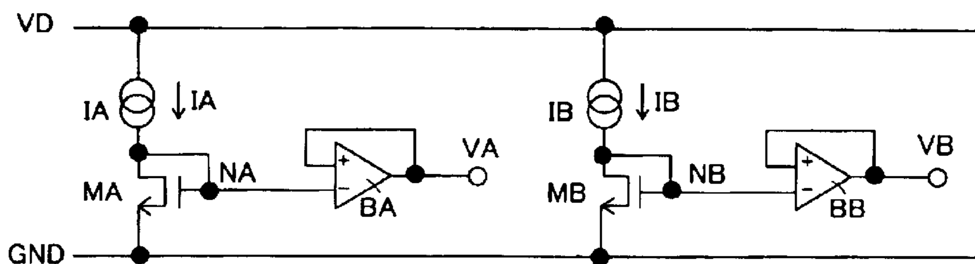
CIRCUIT DIAGRAM OF BIAS VOLTAGE GENERATOR CIRCUIT
