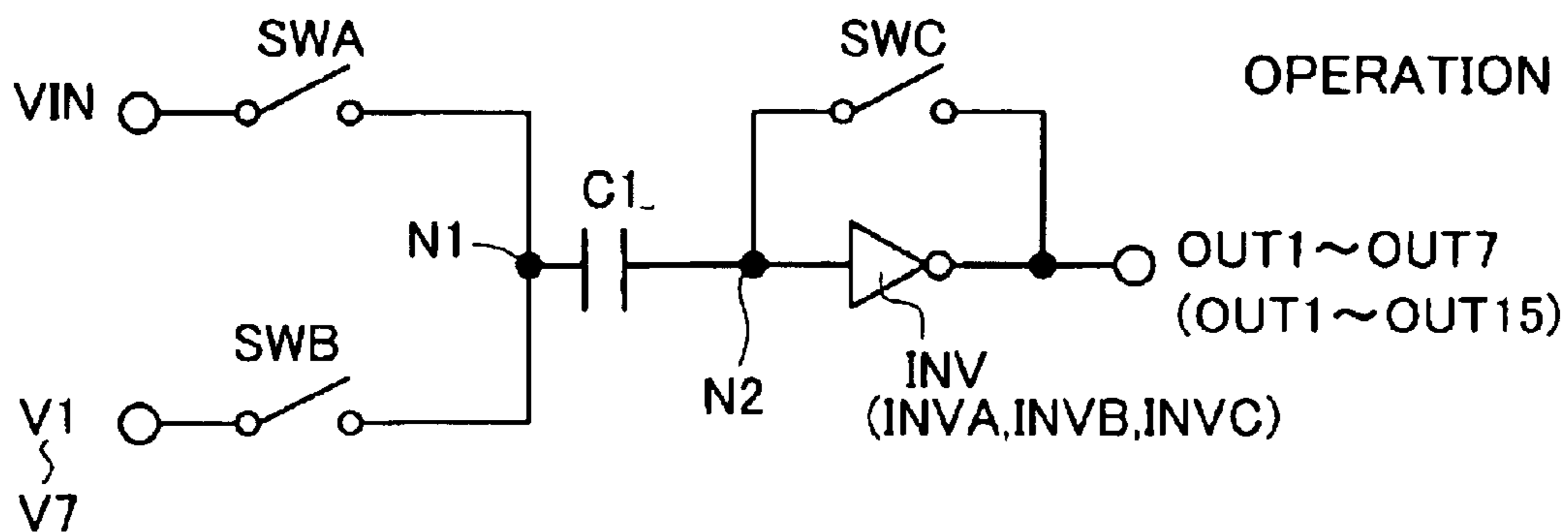
EXPLANATORY VIEW SHOWING CONSTRUCTION OF MAIN PART OF CHOPPER-TYPE CONVERSION COMPARATOR
