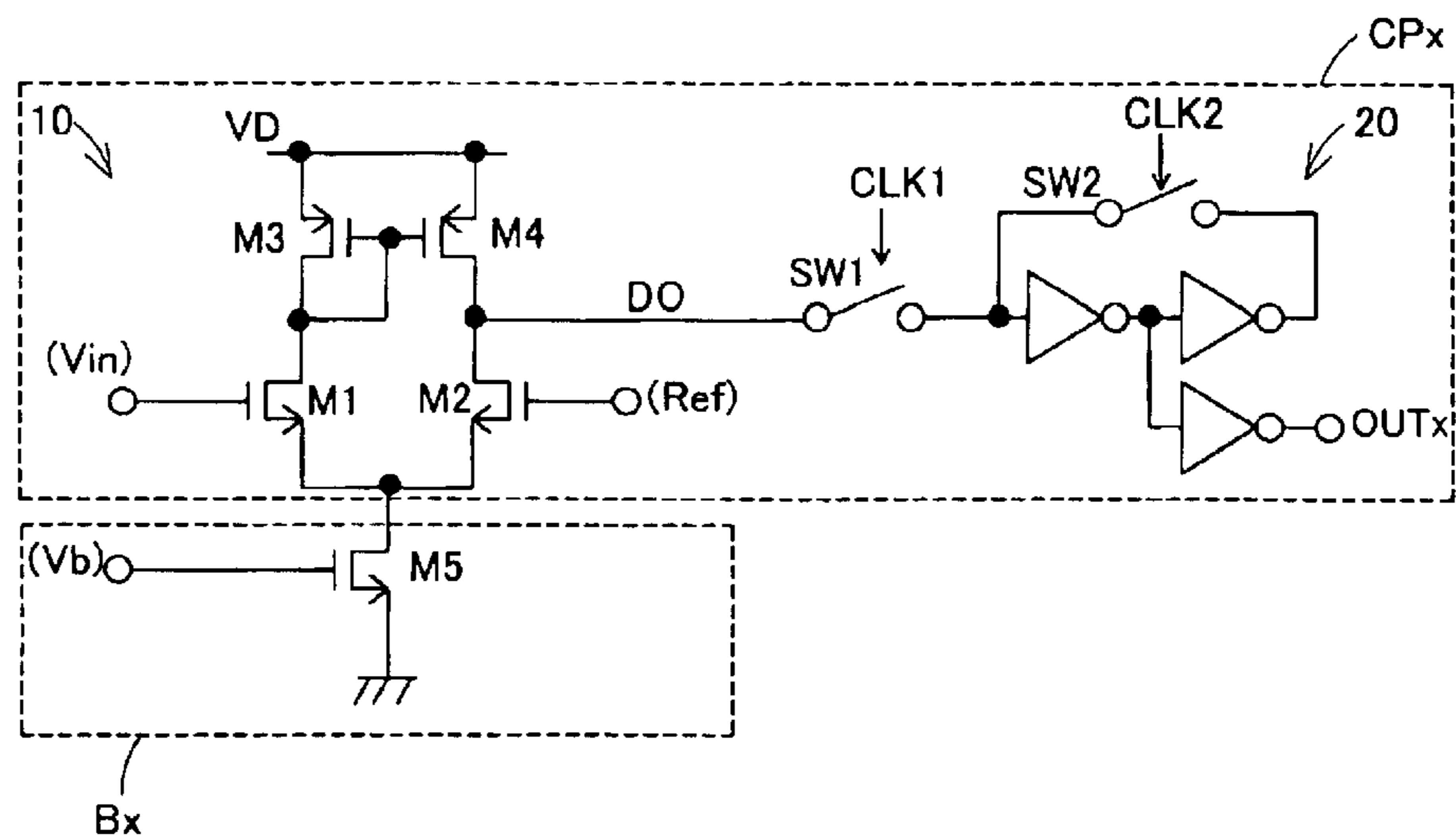
CIRCUIT DIAGRAM OF DIFFERENTIAL-TYPE COMPARATOR
