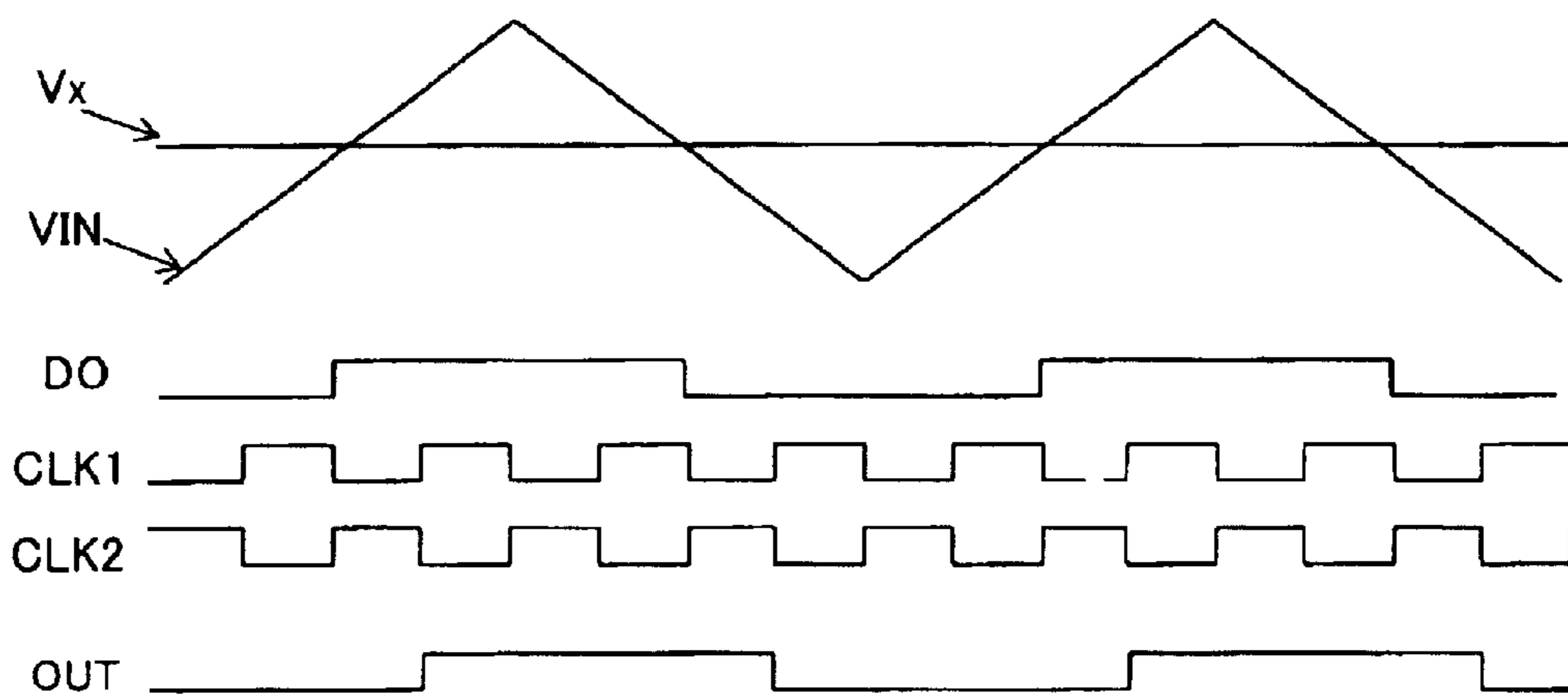
OPERATIONAL WAVEFORM OF DIFFERENTIAL-TYPE COMPARATOR
