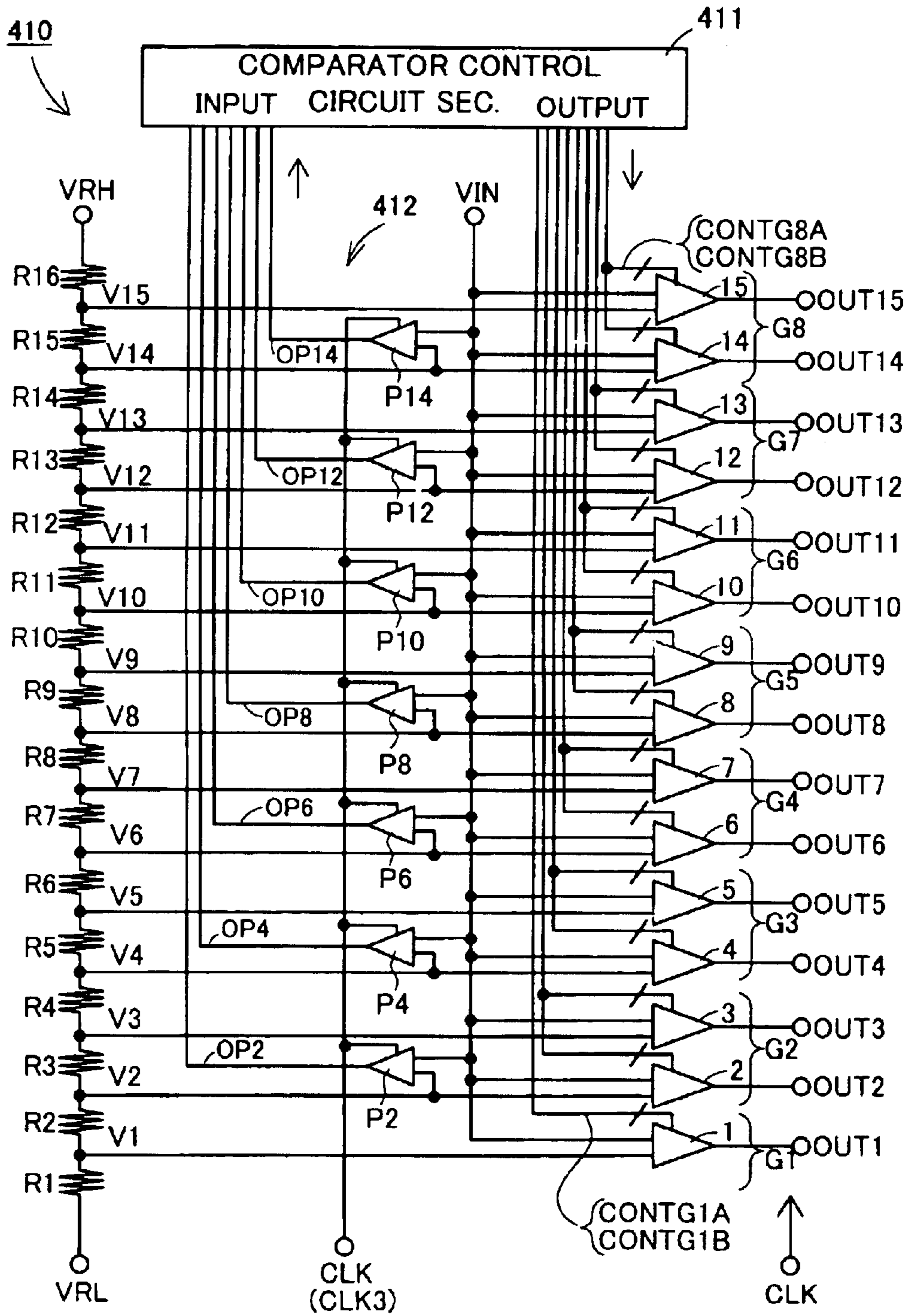
EXPLANATORY VIEW SHOWING OUTLINE OF COMPARISON SECTION OF A/D CONVERTER CIRCUIT DIRECTED TO EMBODIMENT 4
