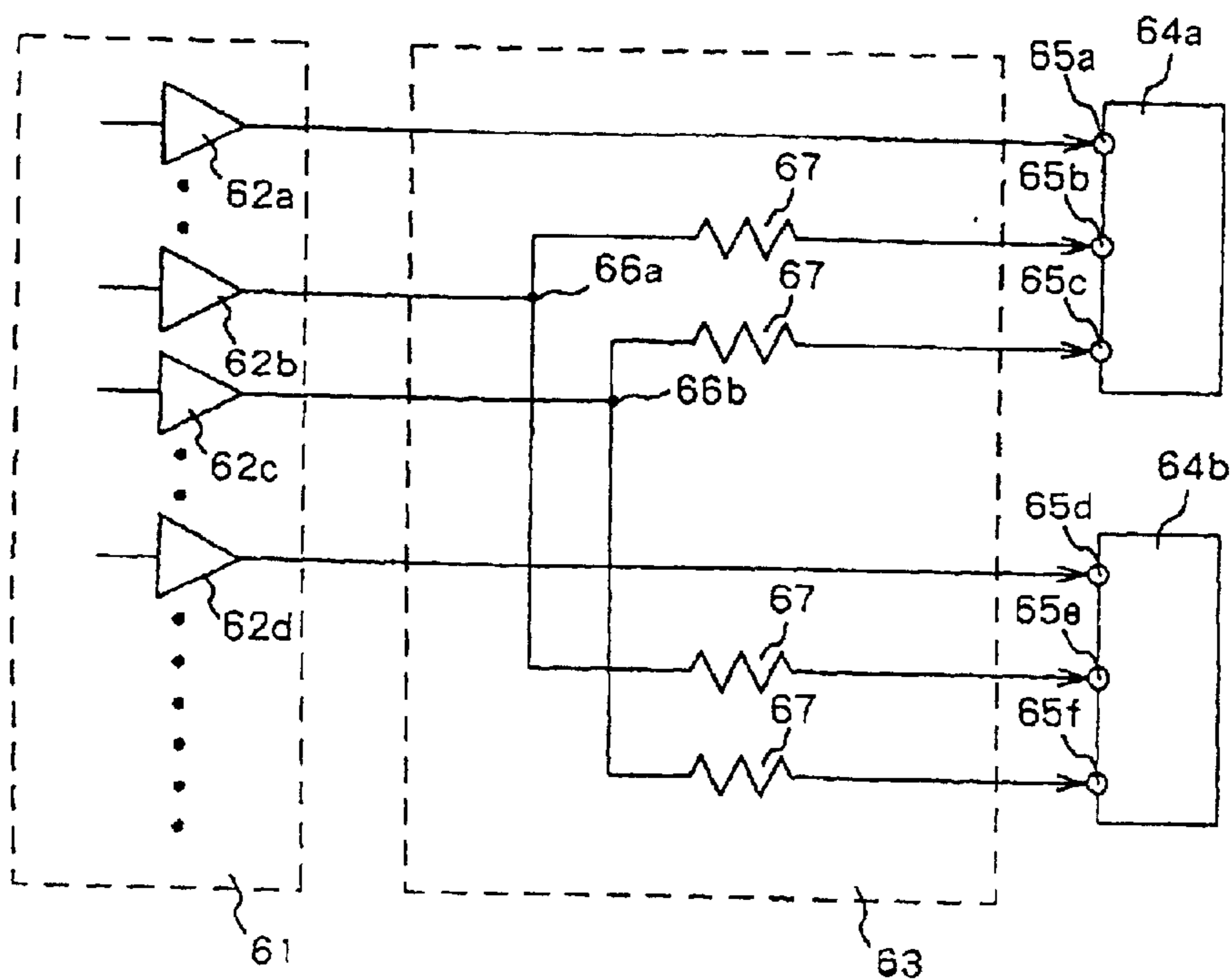
FIG. 3 (PRIOR ART)
