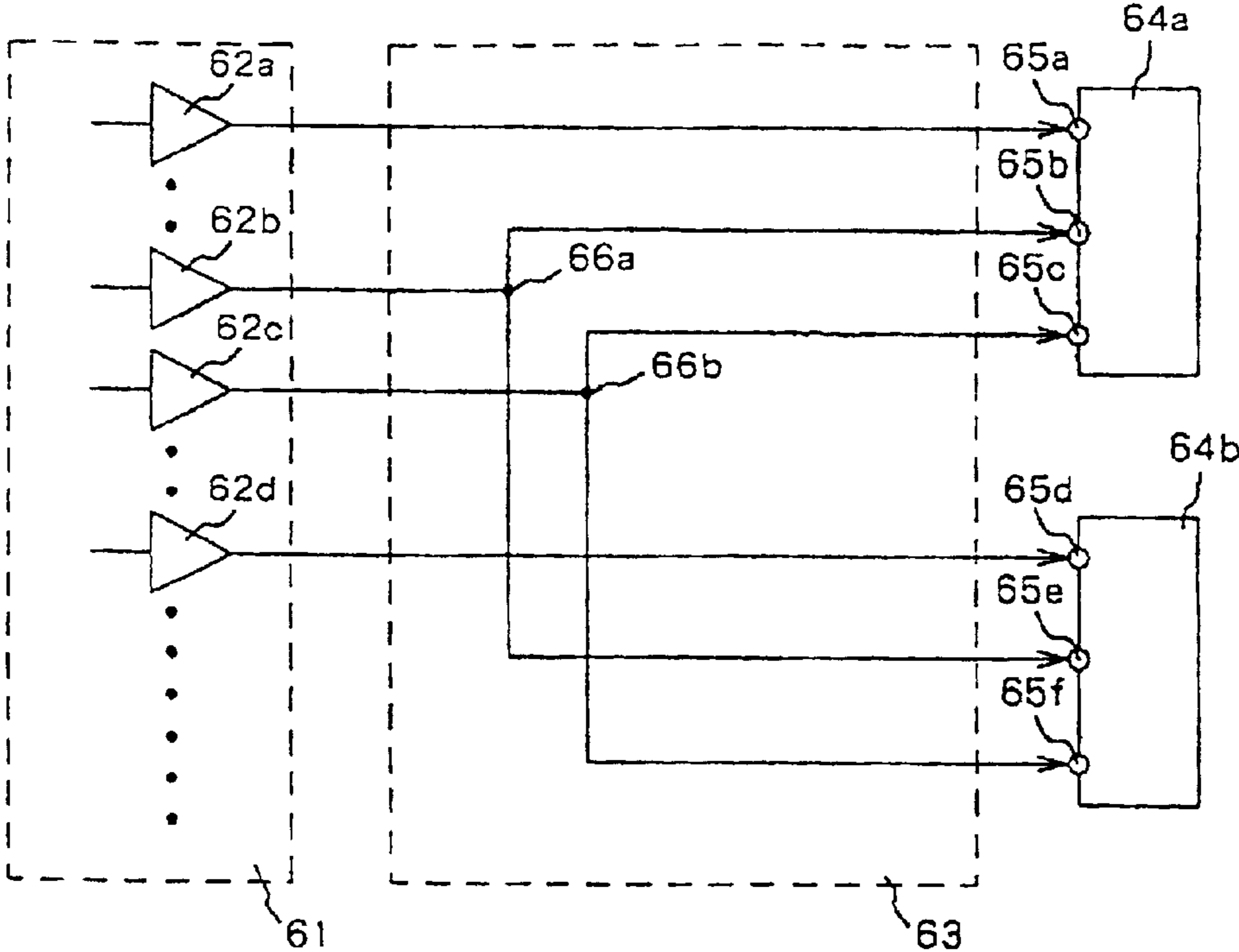
FIG. 2 (PRIOR ART)
