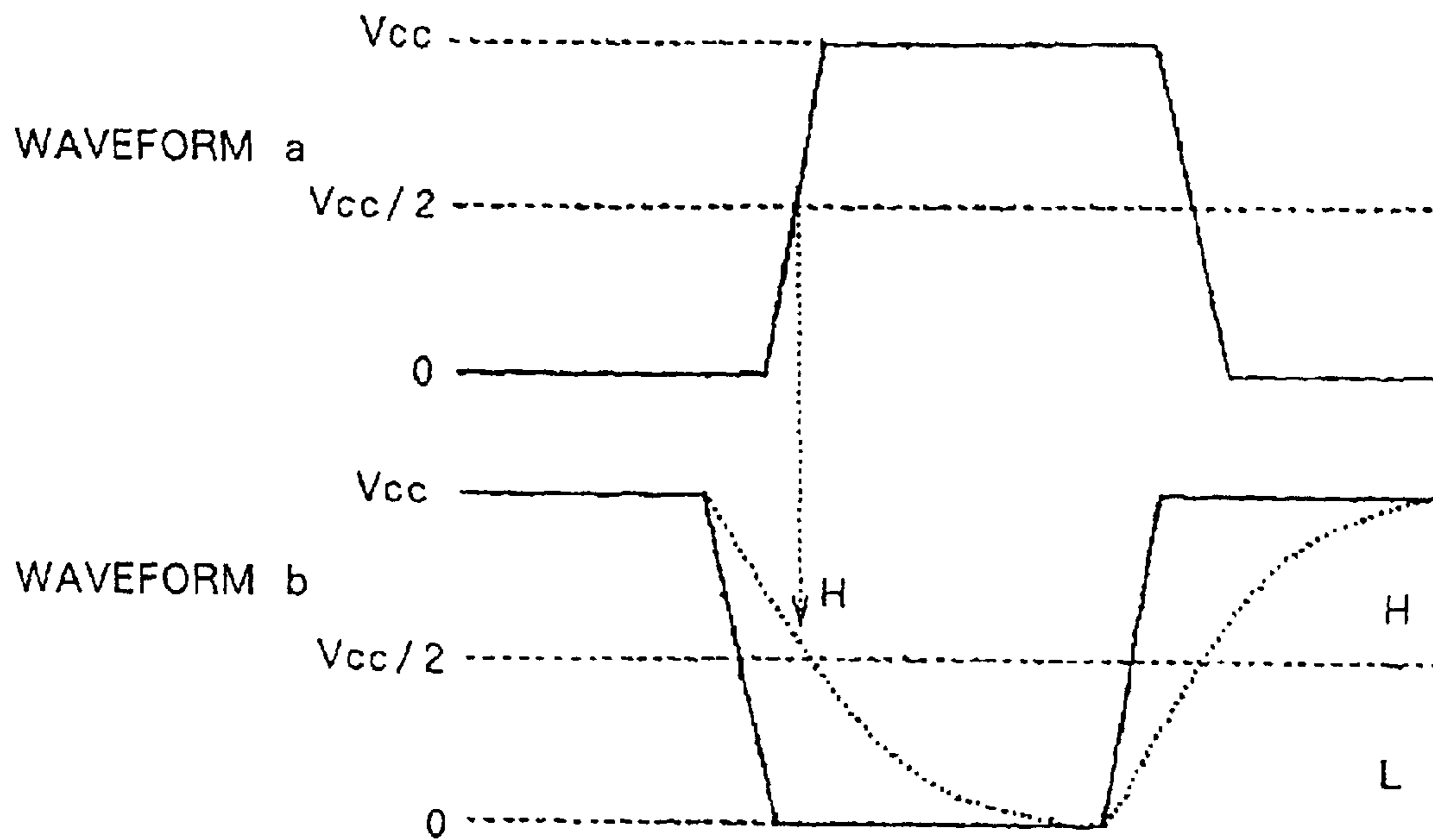
FIG. 4 (PRIOR ART)
