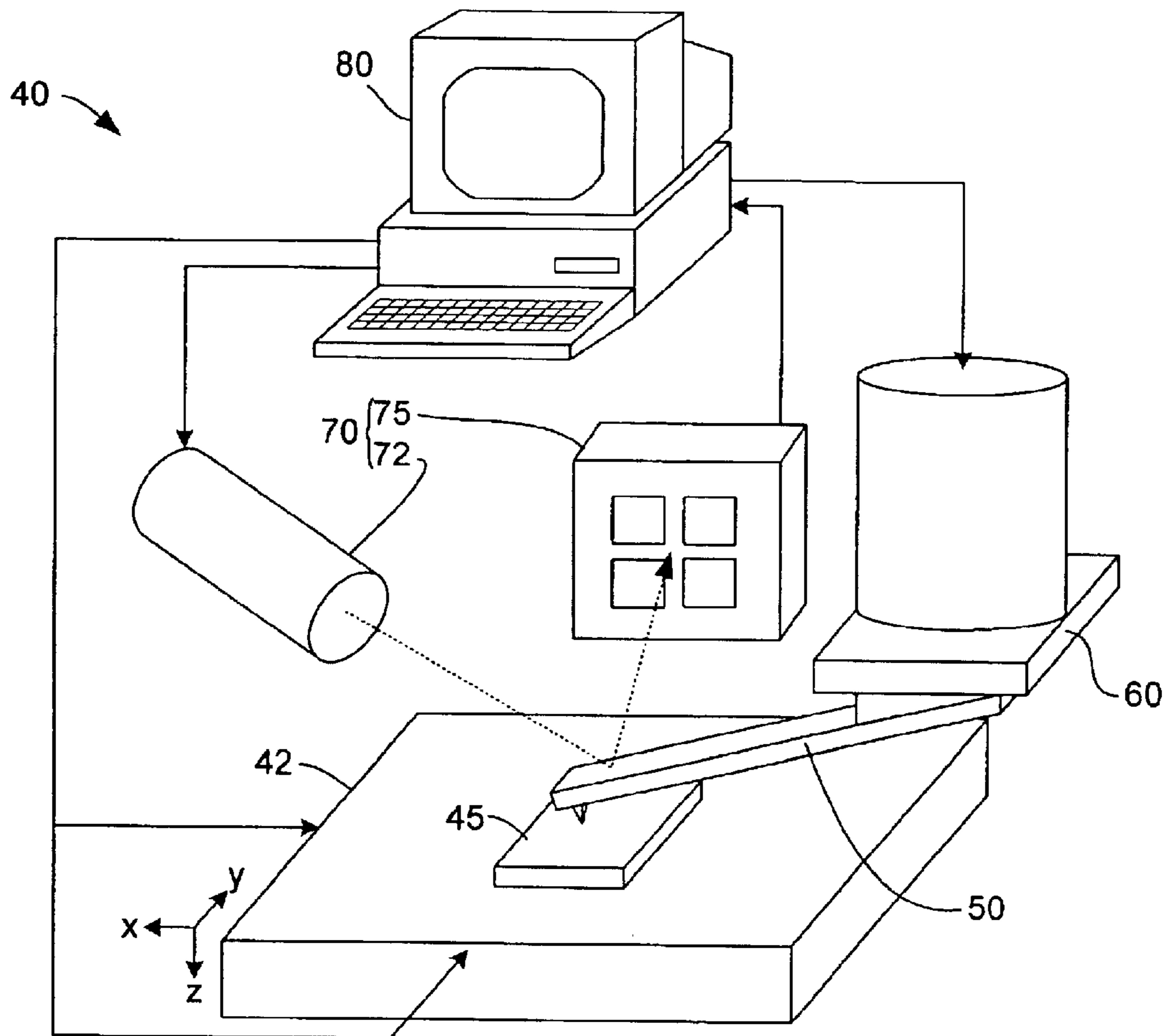
FIG. 24 (PRIOR ART)
