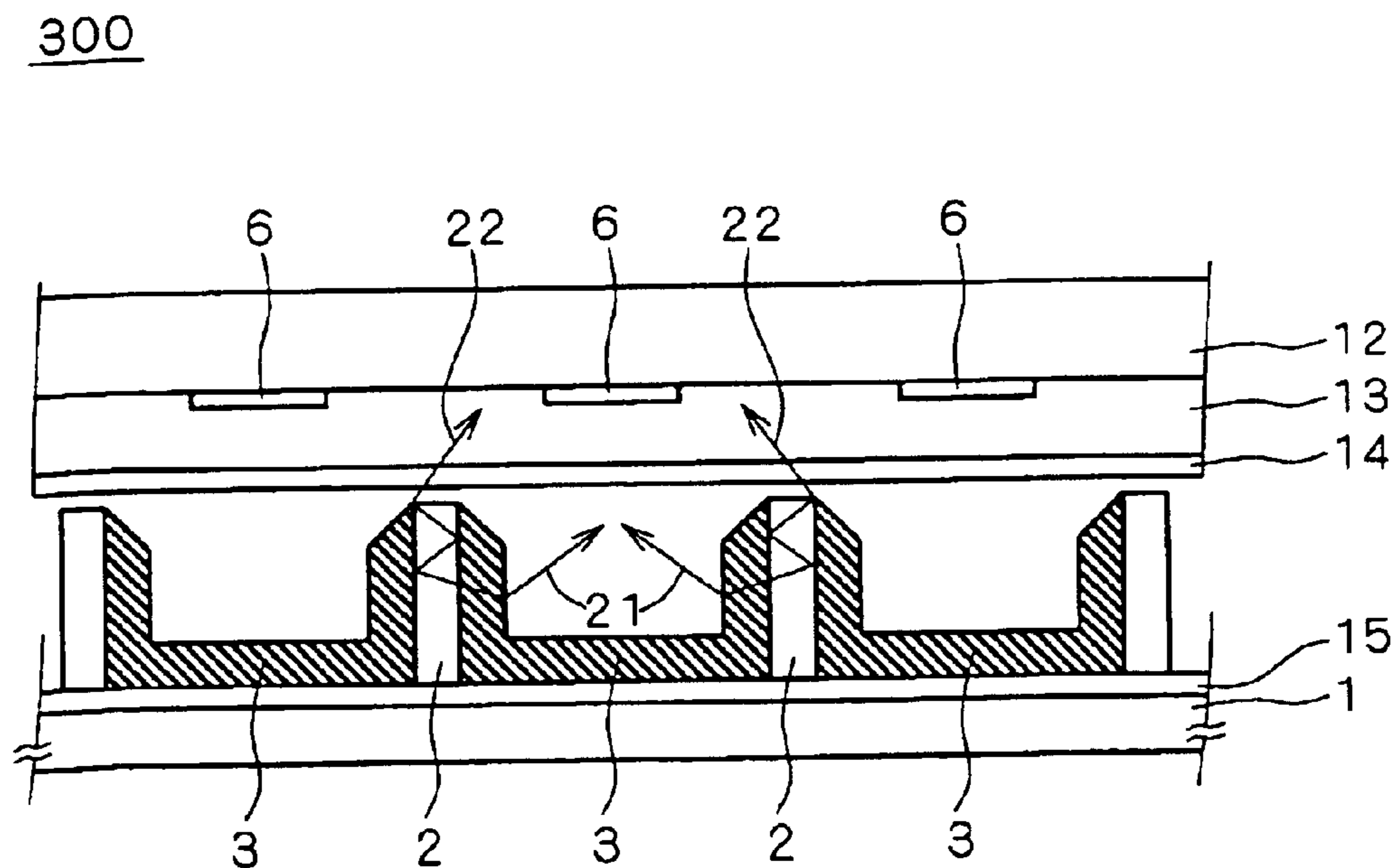
FIG. 22 — PRIOR ART —
