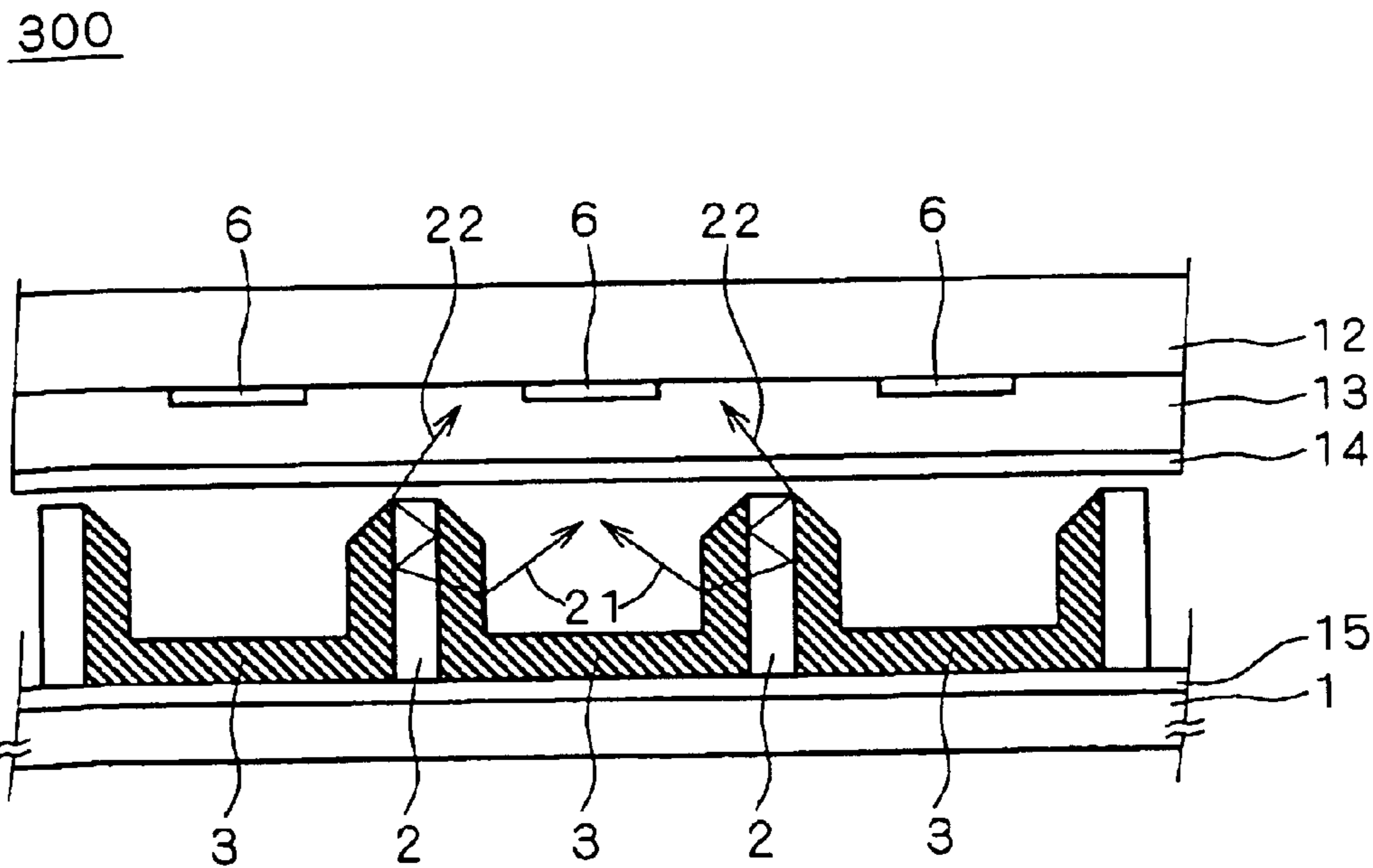
FIG. 22 — PRIOR ART —
