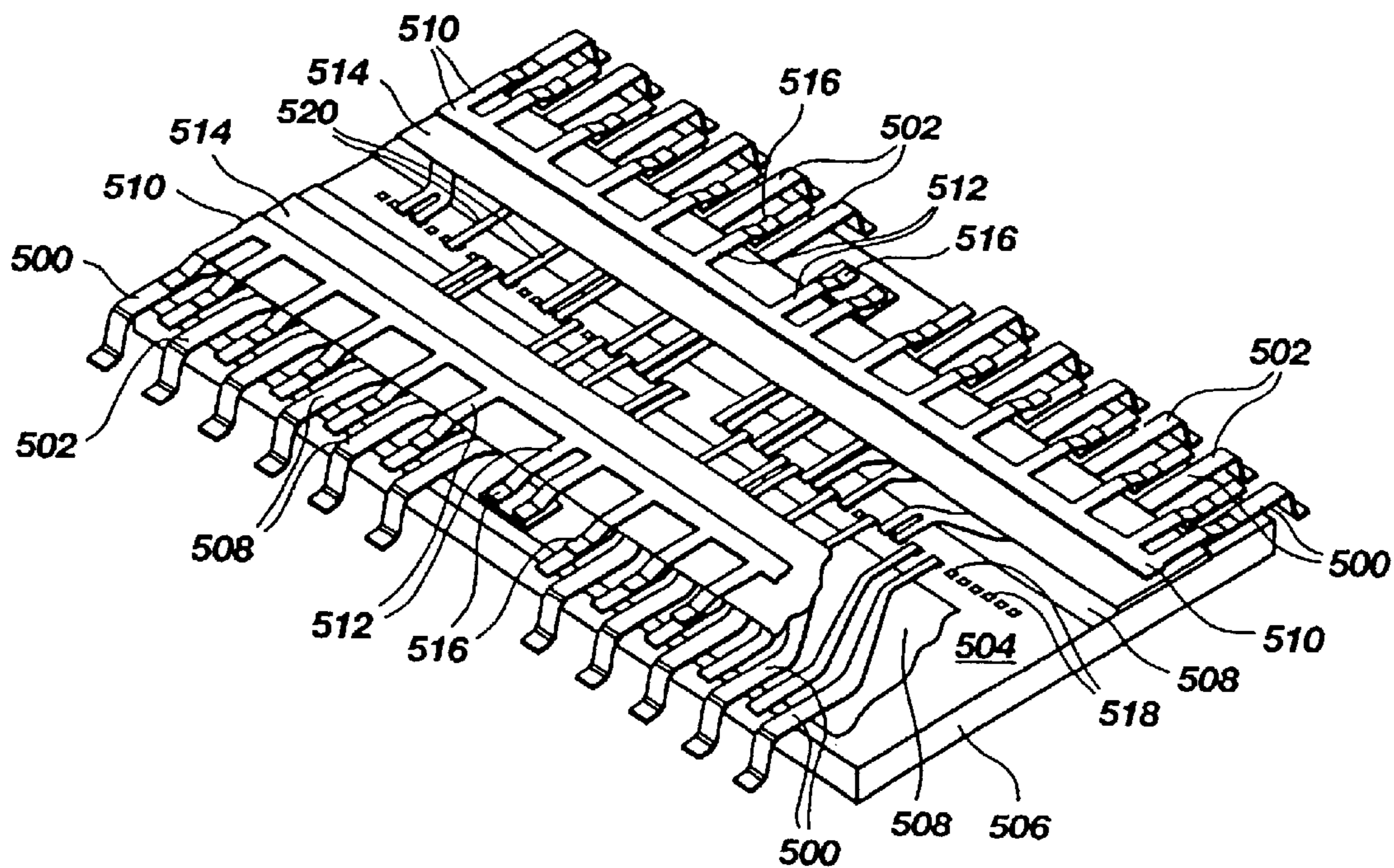
Fig. 19 (PRIOR ART)
