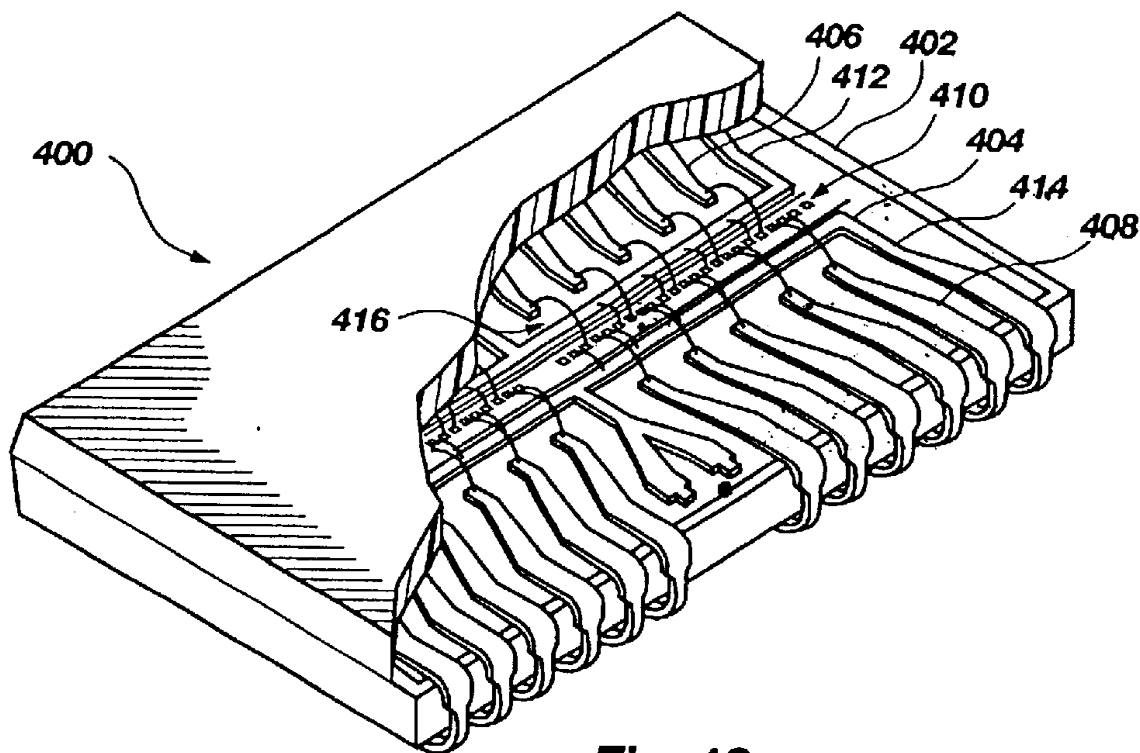
Fig. 18 (PRIOR ART)
