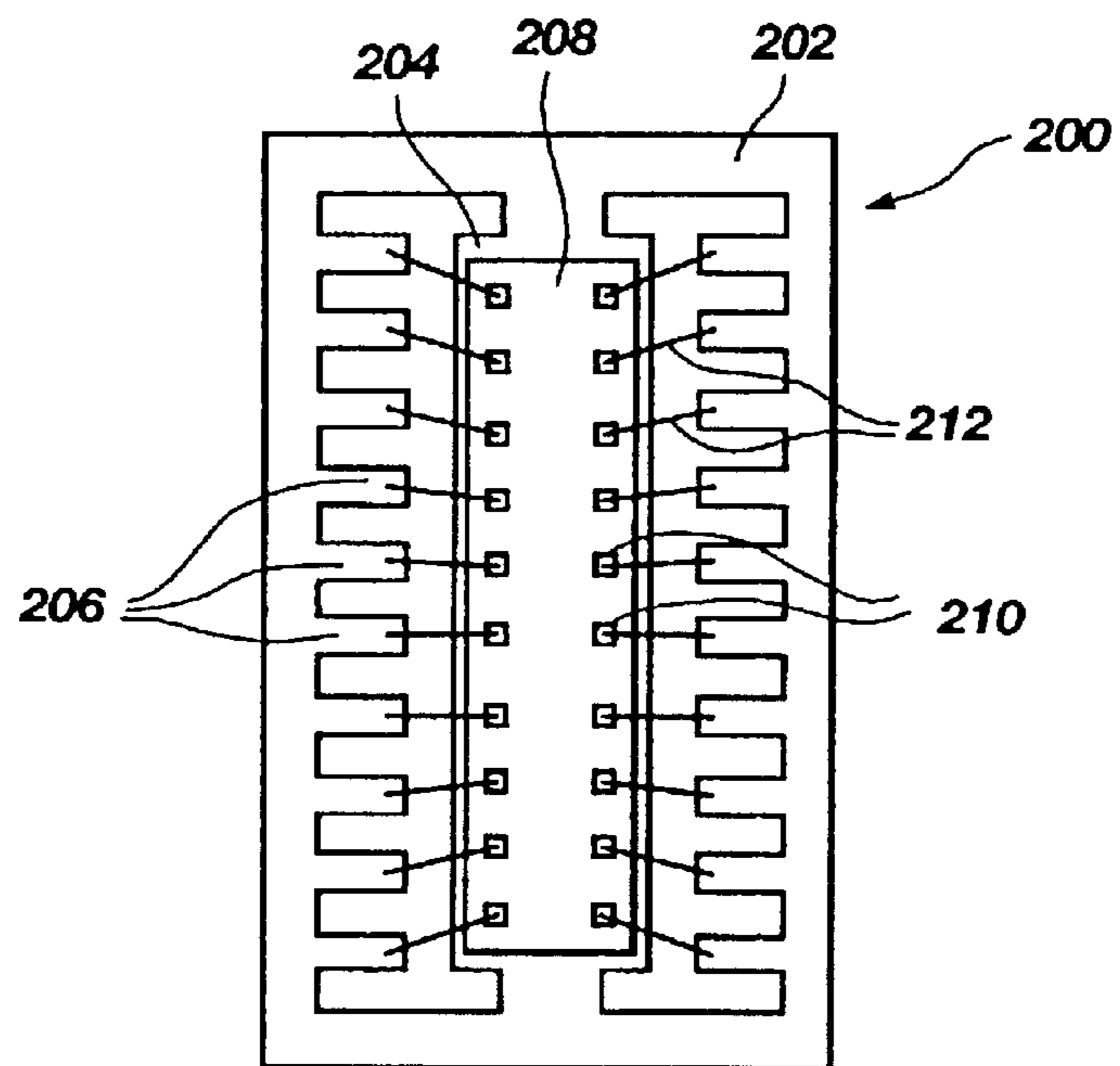
Fig. 16 (PRIOR ART)
