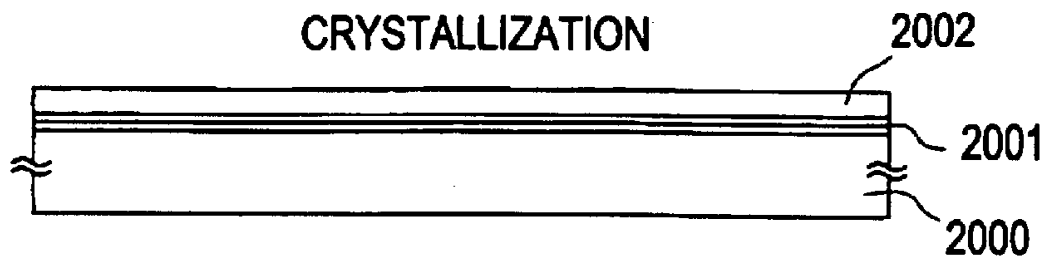
FIG. 37B FORMATION OF BARRIER LAYER AND FORMATION OF SEMICONDUCTOR FILM
