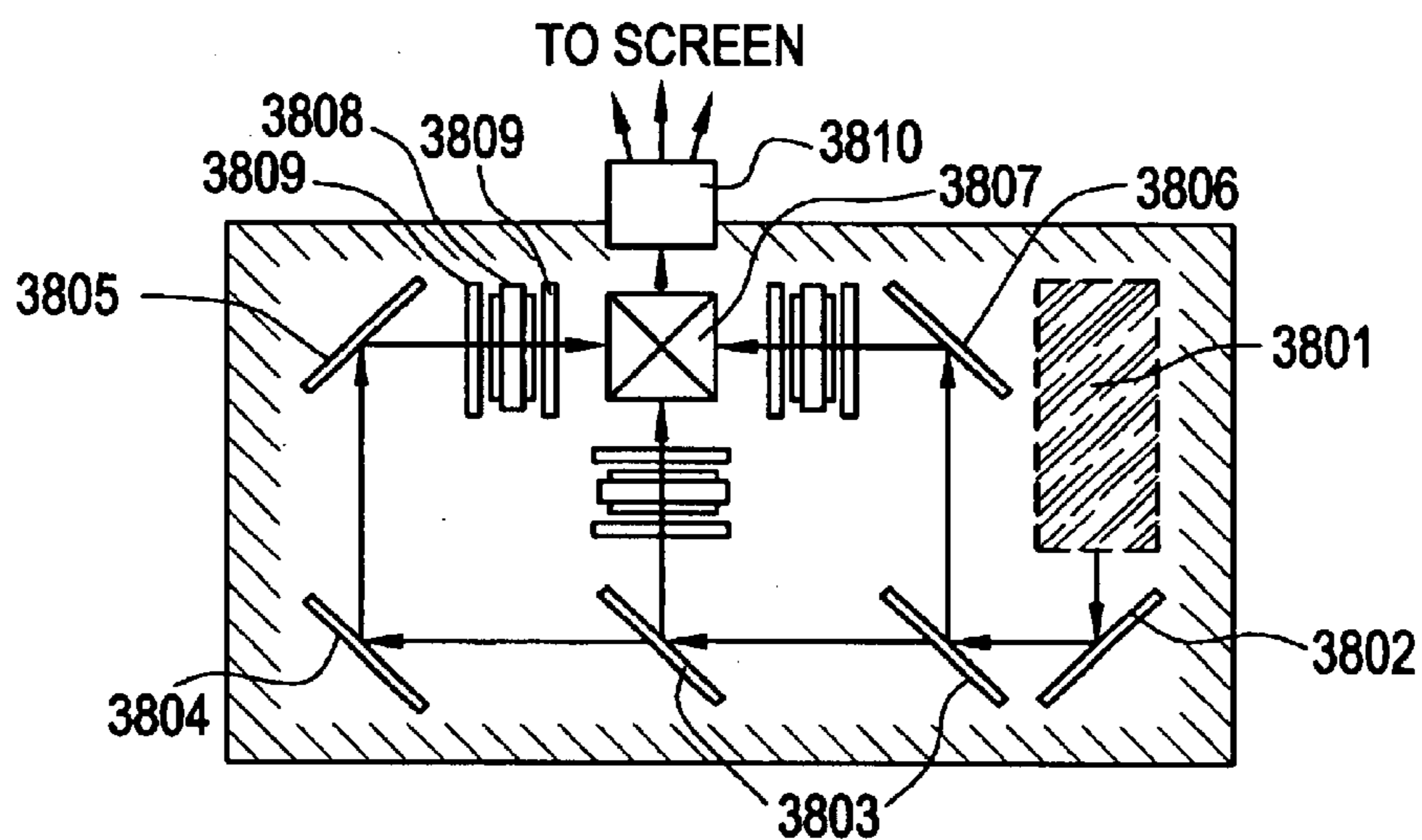
PROJECTING APPATUS (THREE PLATE TYPE)
