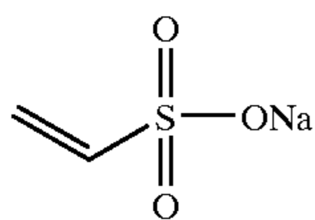
e. Vinyl sulfonic acid sodium salt
