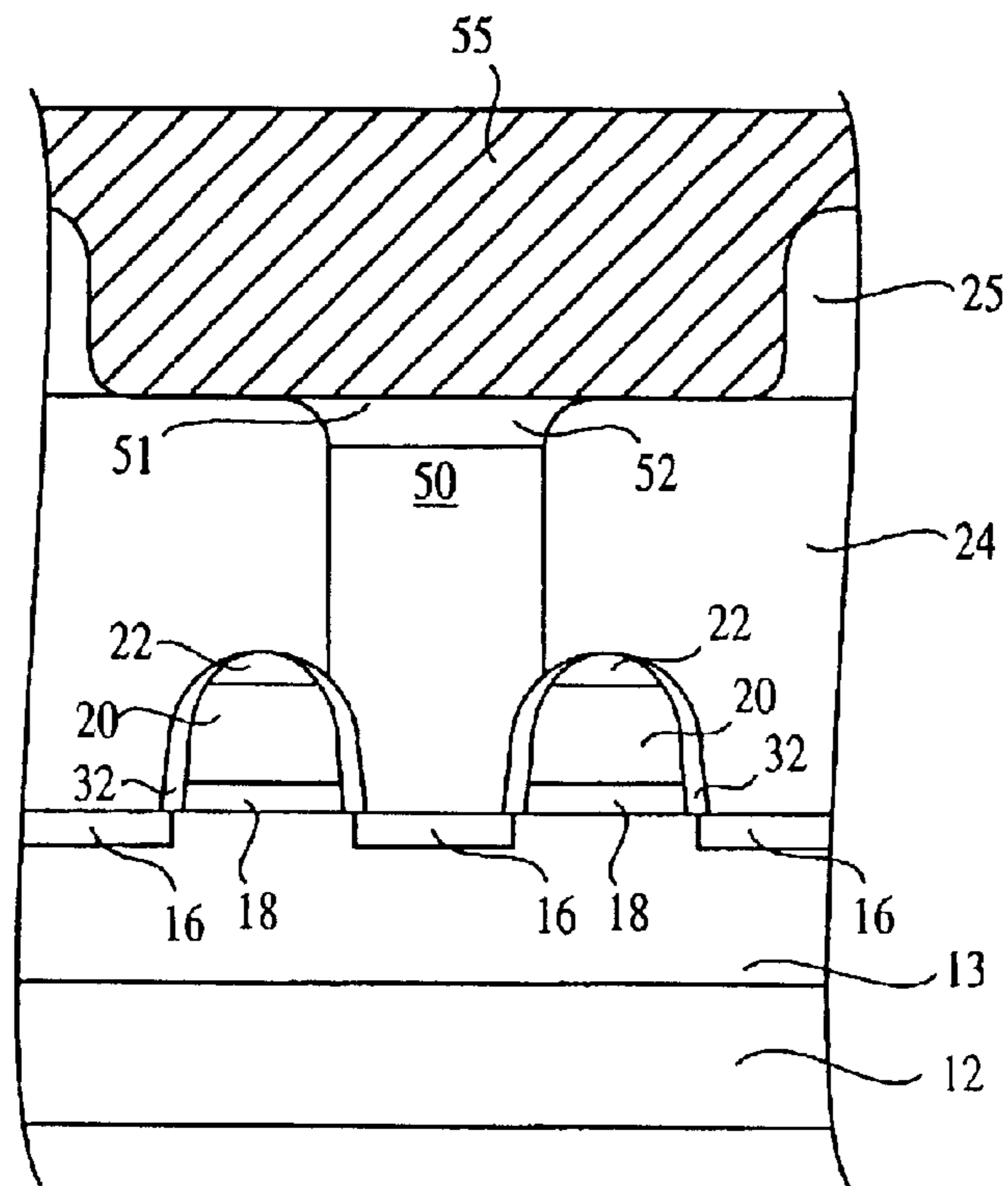
FIG. 2 PRIOR ART
