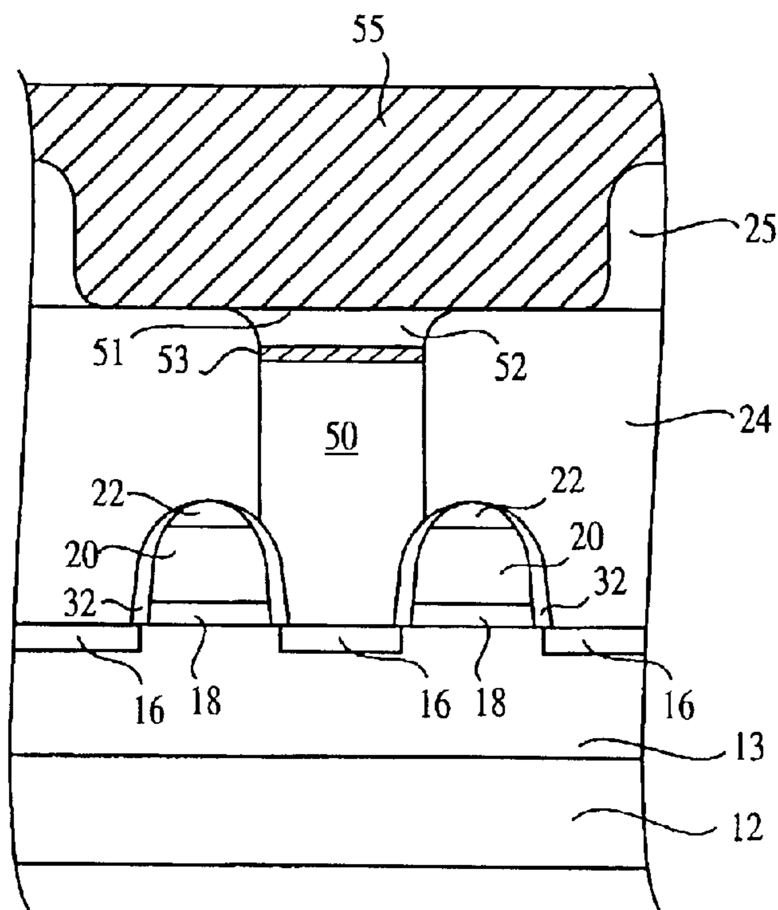
FIG. 3 PRIOR ART
