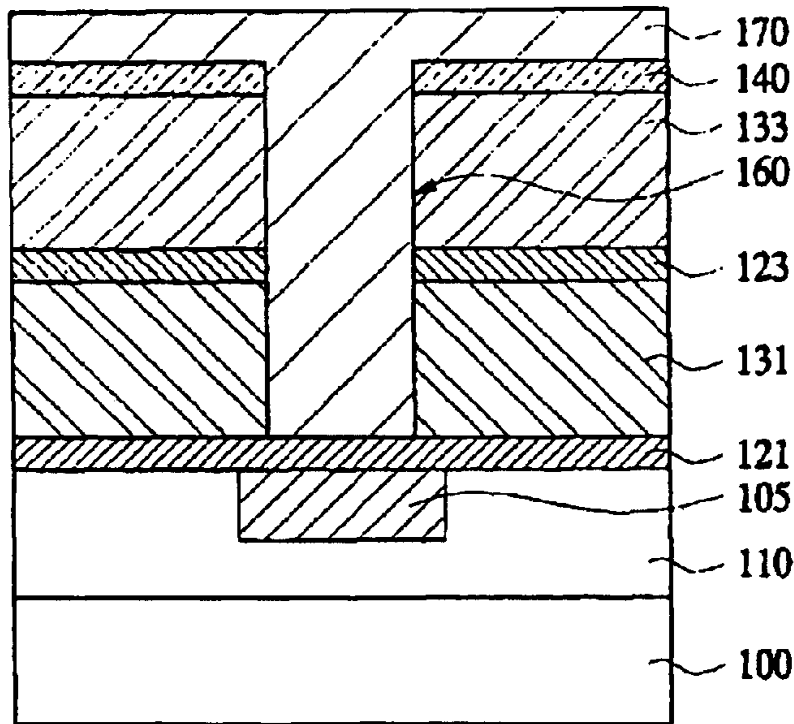
FIG. 1C (PRIOR ART)
