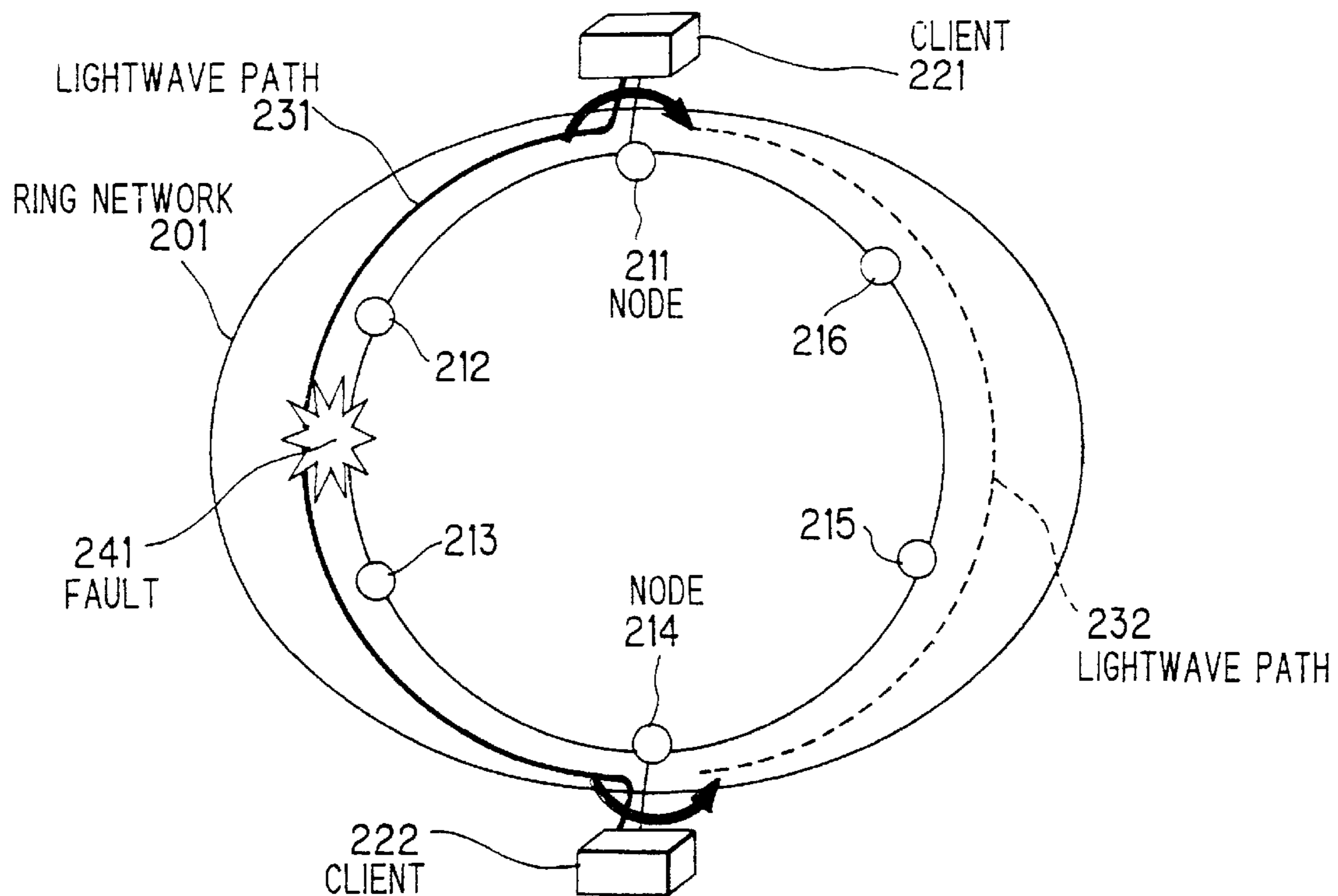
FIG. 2 PRIOR ART
