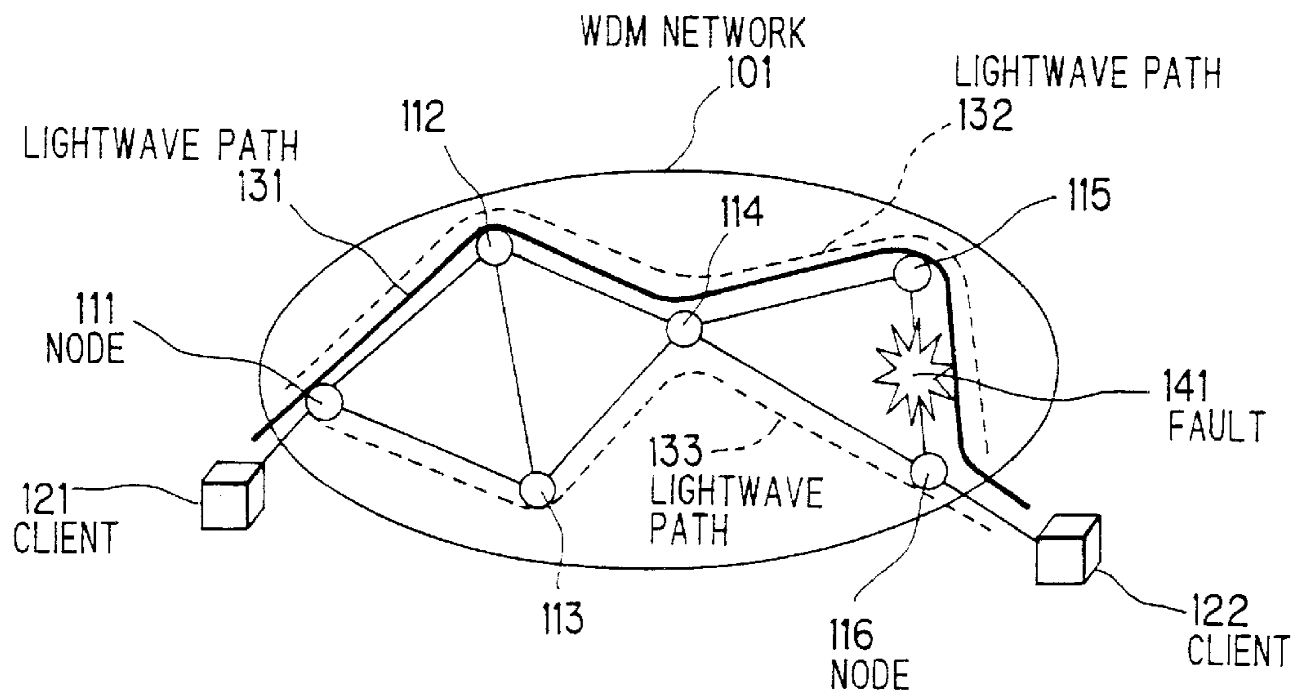
FIG. 1 PRIOR ART
