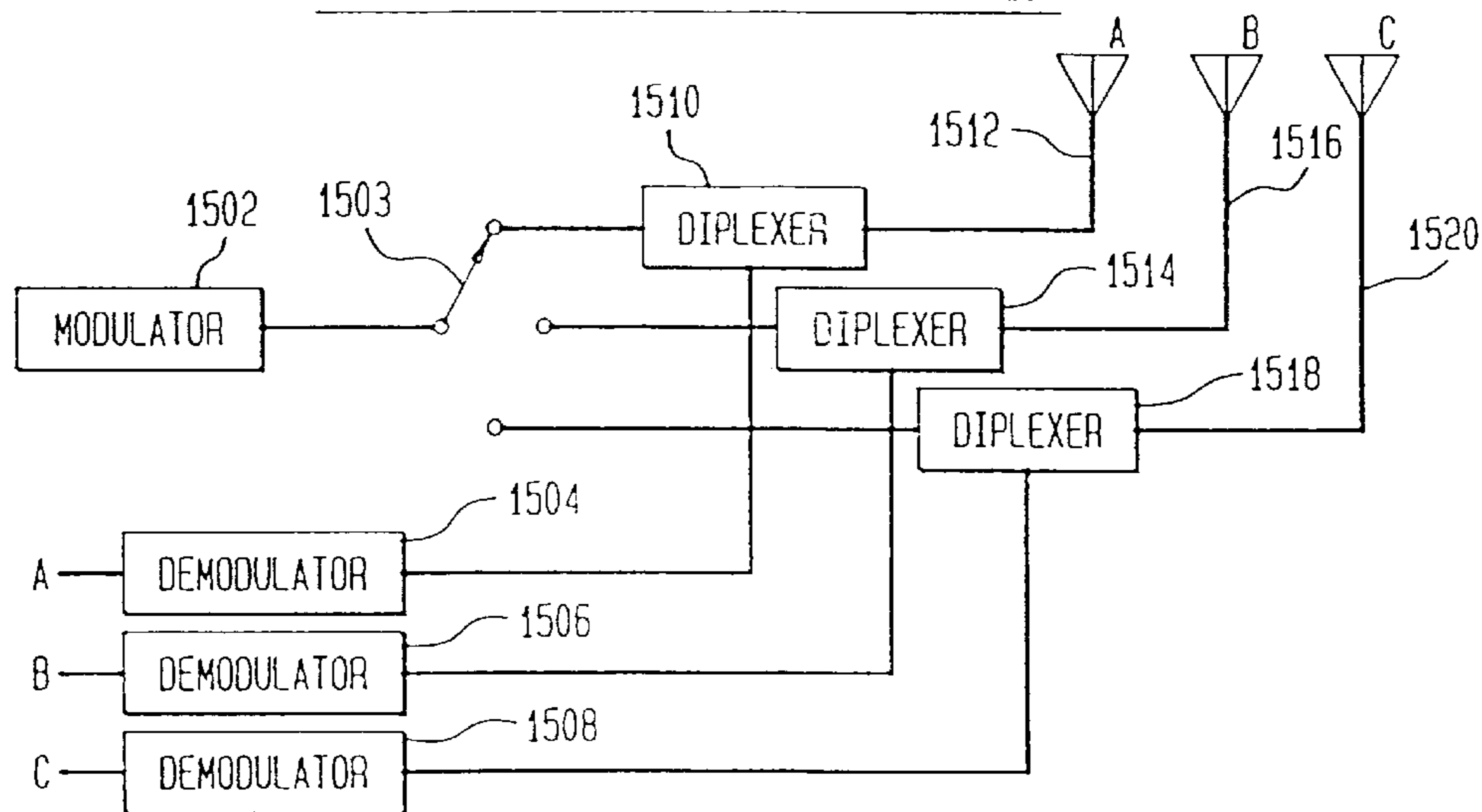
TRANSFER STATION ANTENNA IMPLEMENTATION
