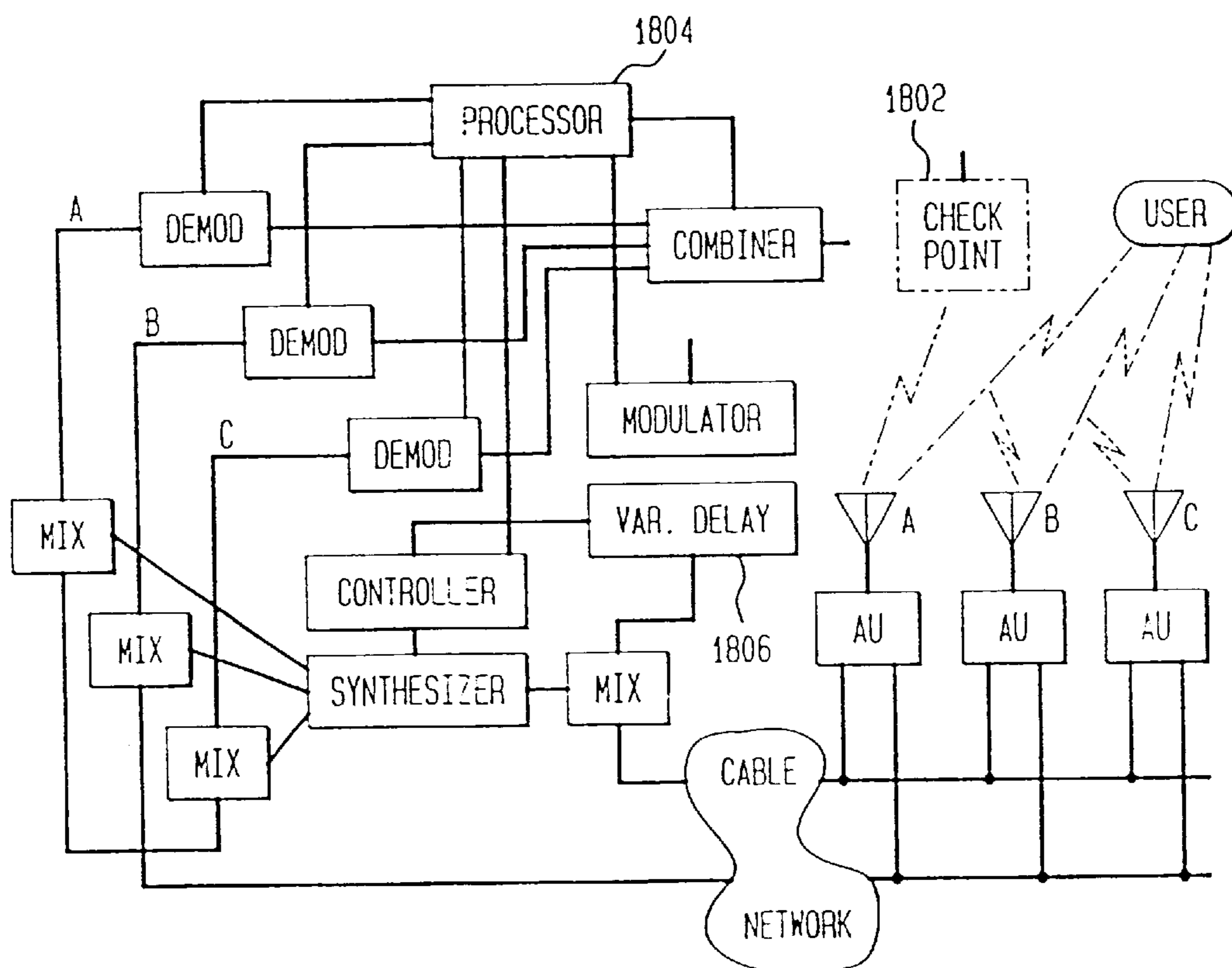
TIME CALIBRATION FOR DISTRIBUTED ANTENNA IMPLEMENTATION
