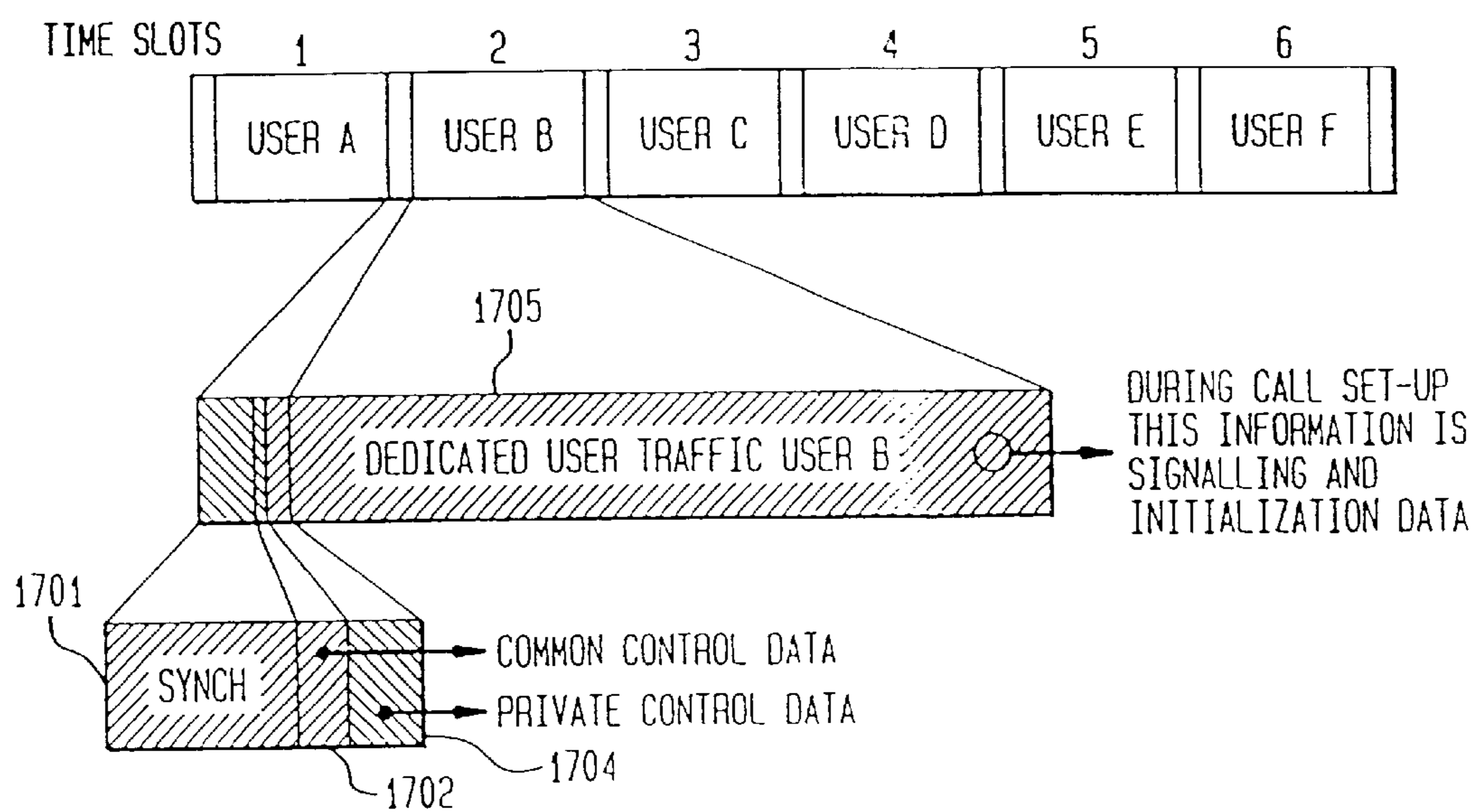
SYNCH AND CONTROL CHANNEL STRUCTURE
