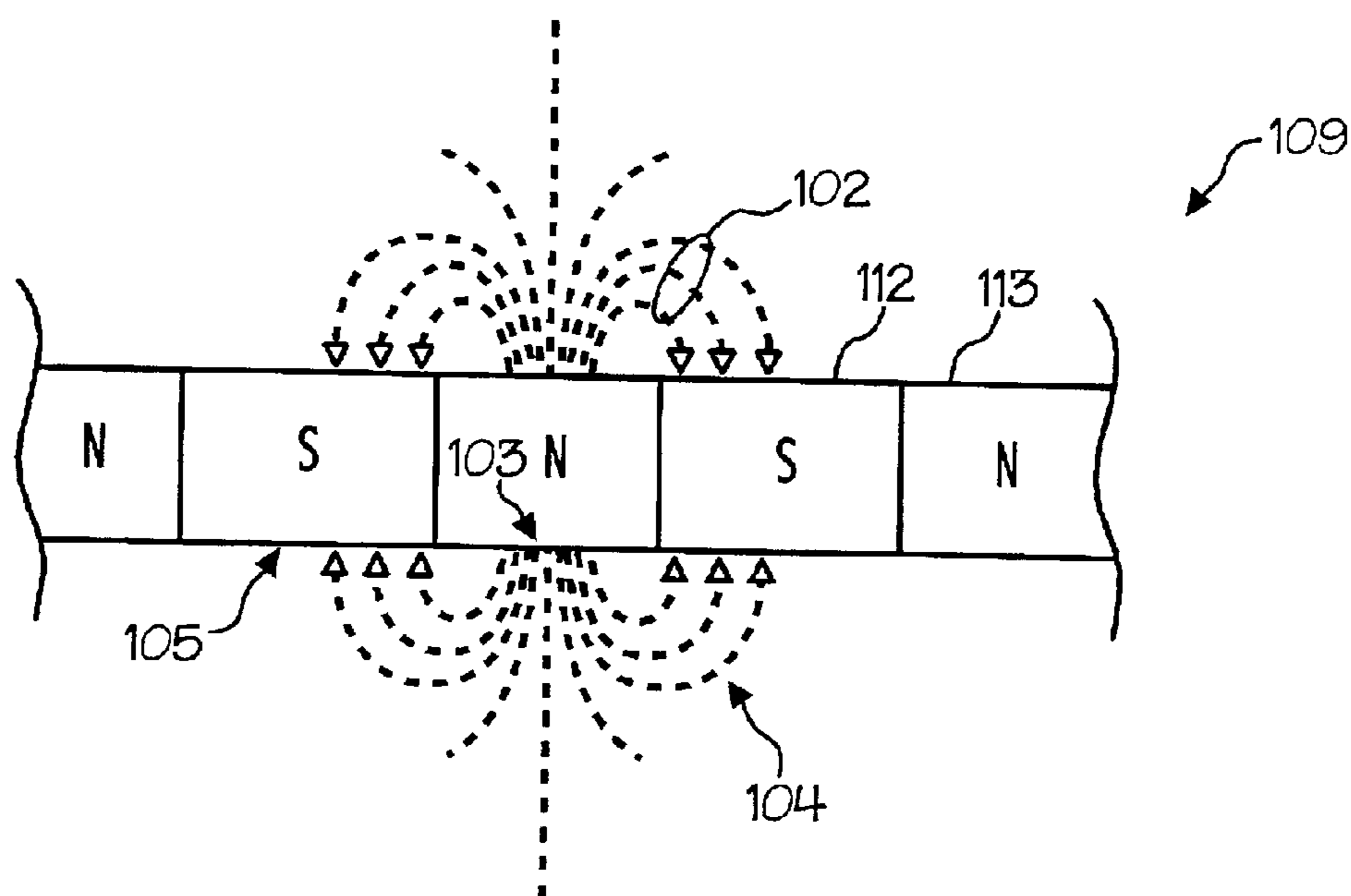
FIG. 1C PRIOR ART
