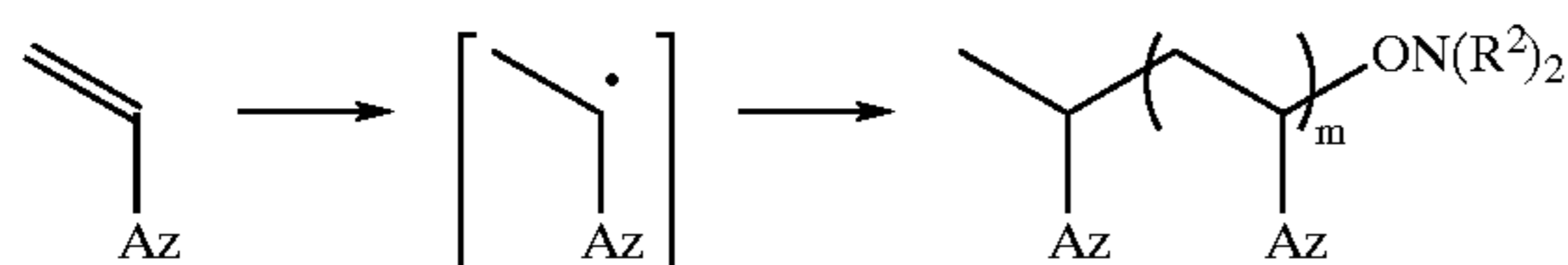
Scheme I
