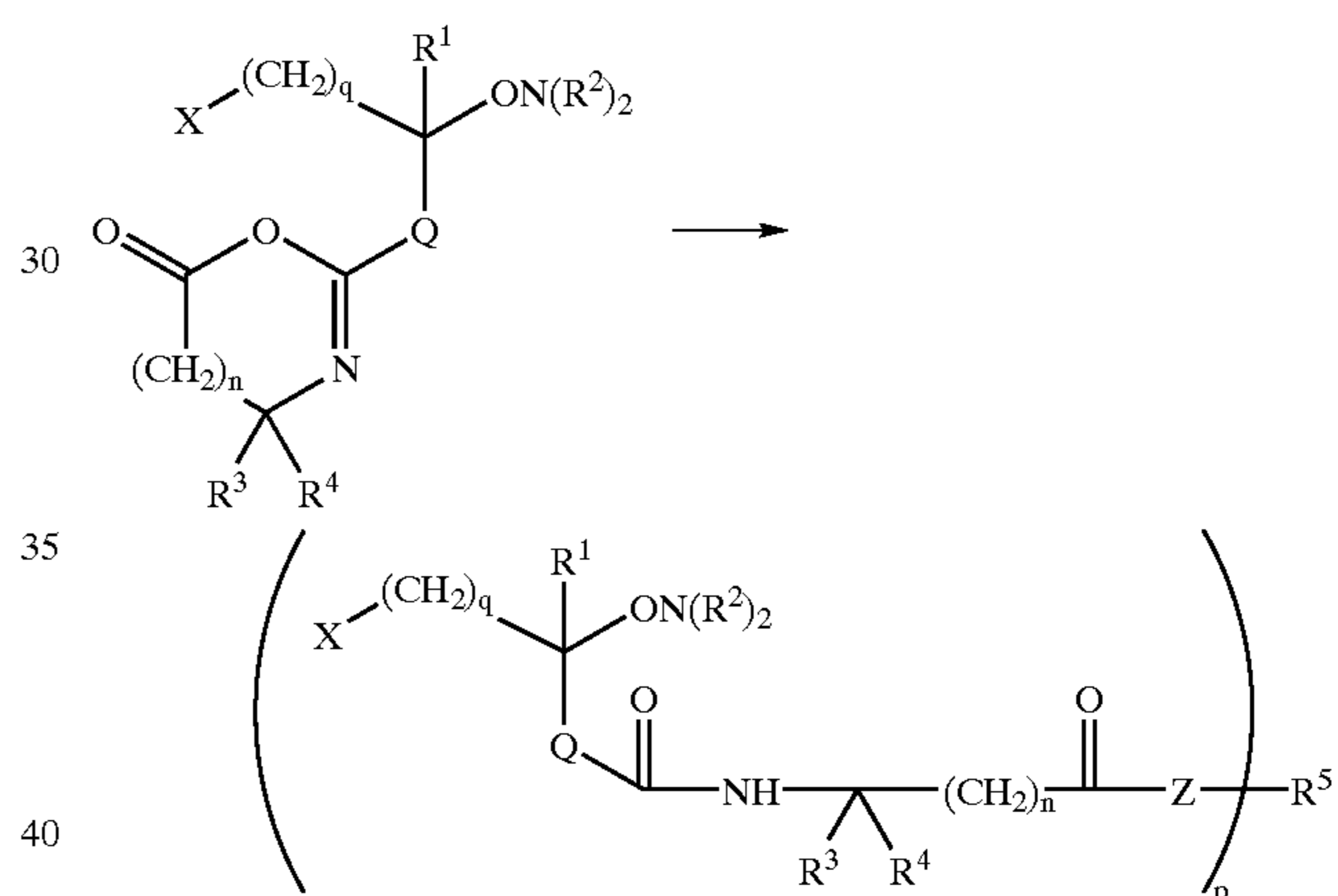
Scheme III
