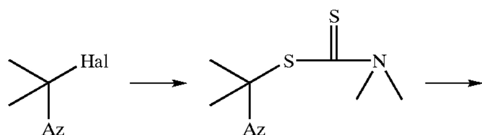
Scheme II
