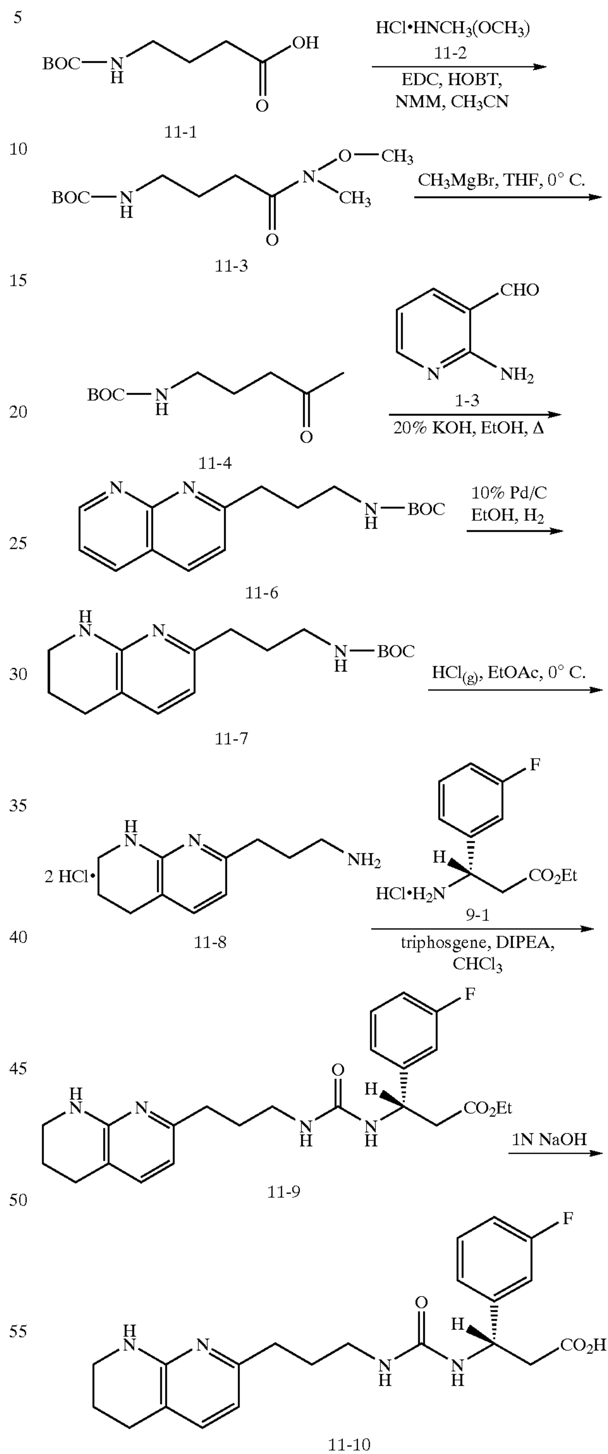
SCHEME 11
