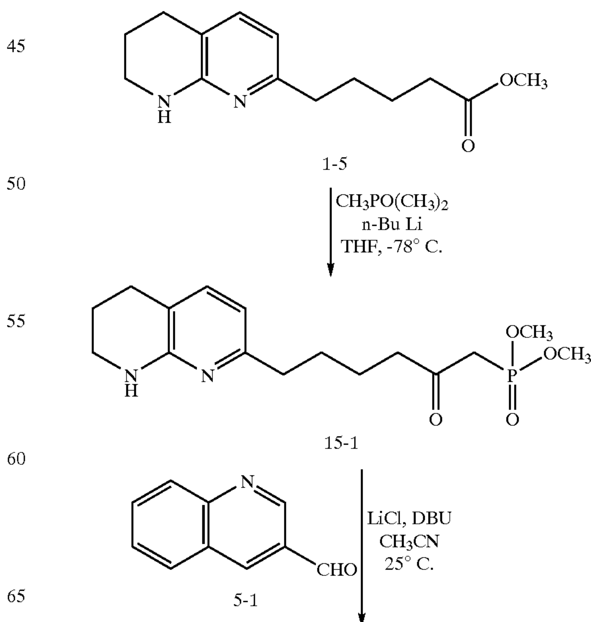
SCHEME 15
