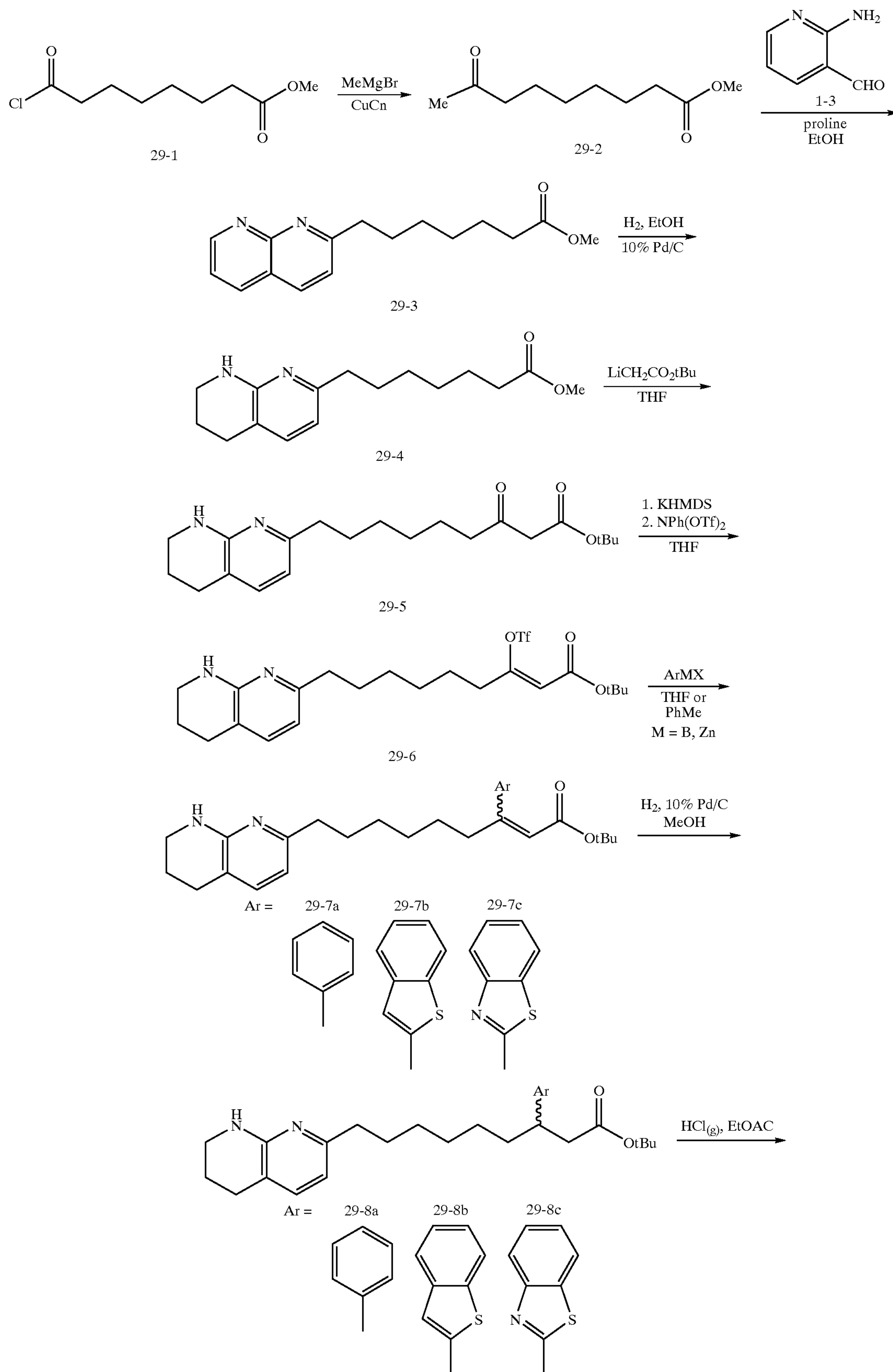
SCHEME 29
