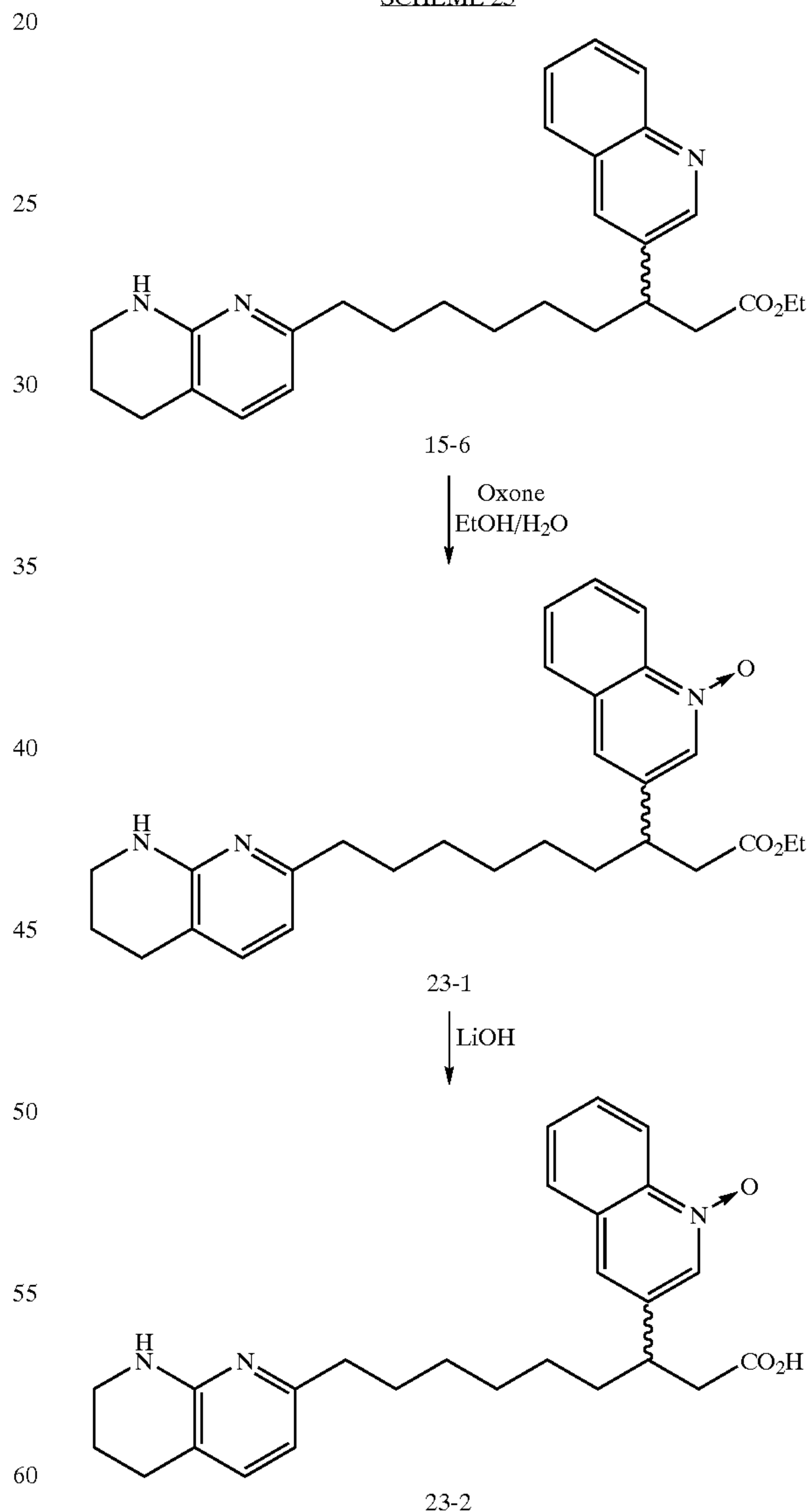
SCHEME 23
