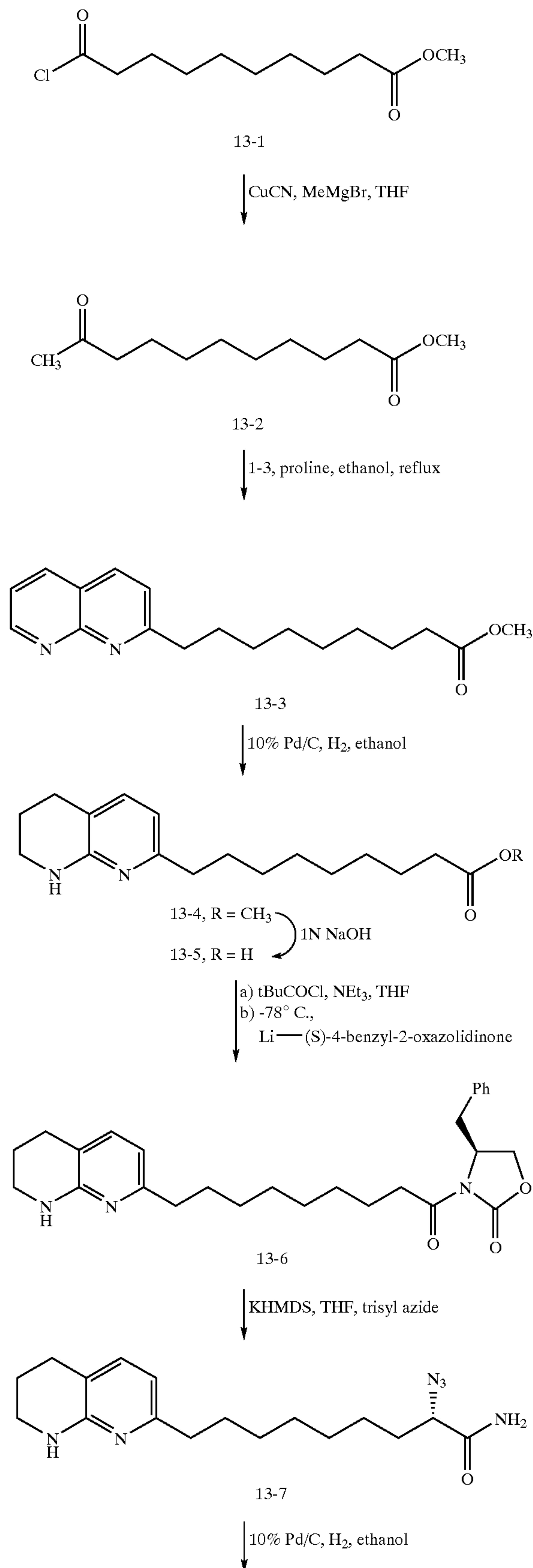
SCHEME 13
