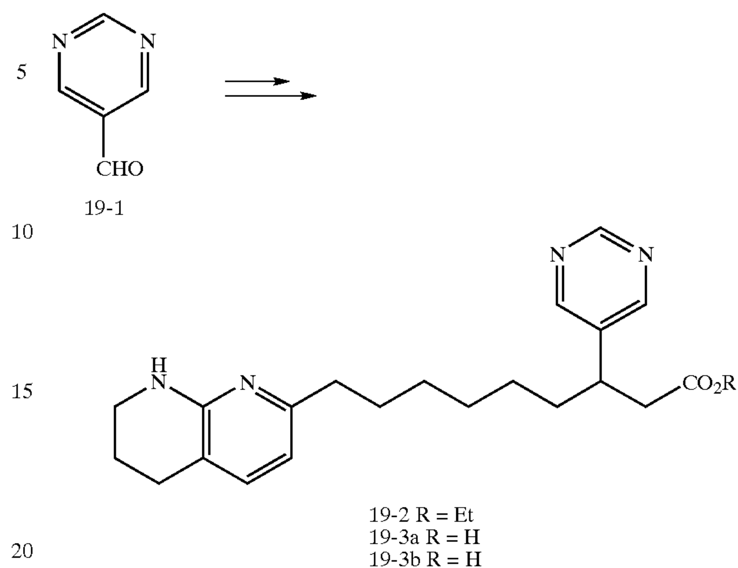
SCHEME 19
