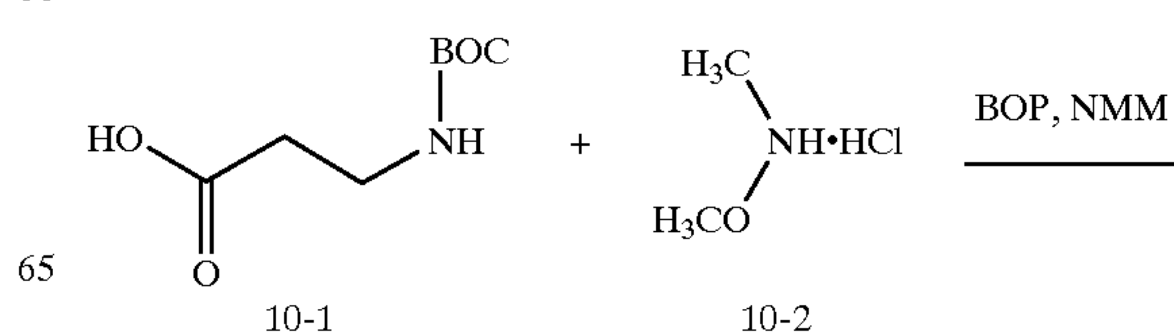
SCHEME 10
