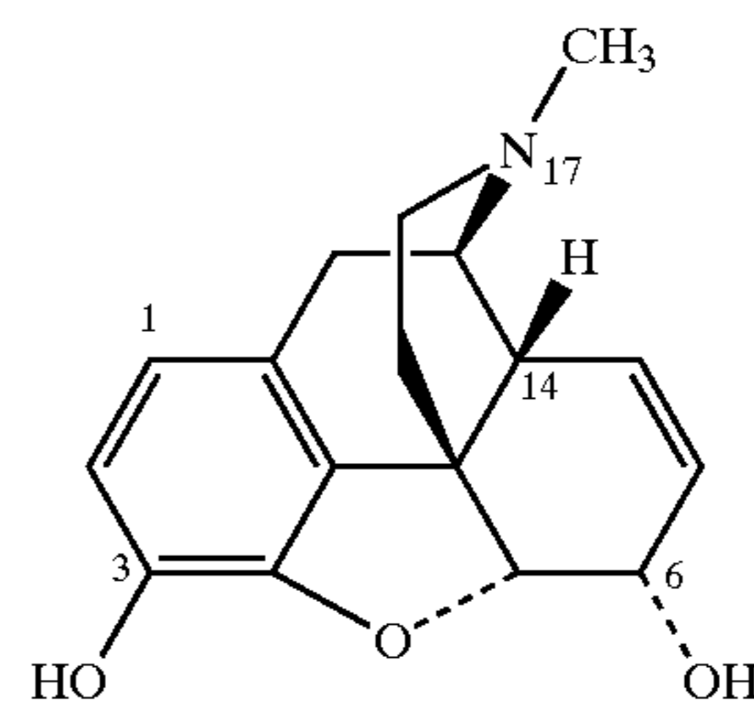
Morphine
