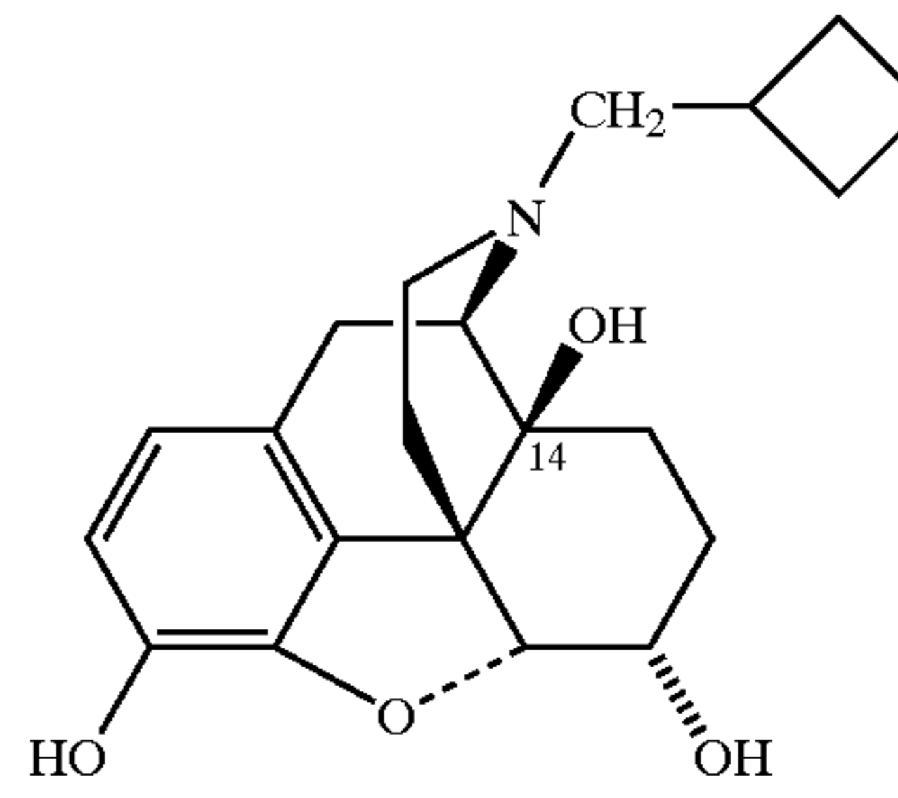
Nalbuphine
