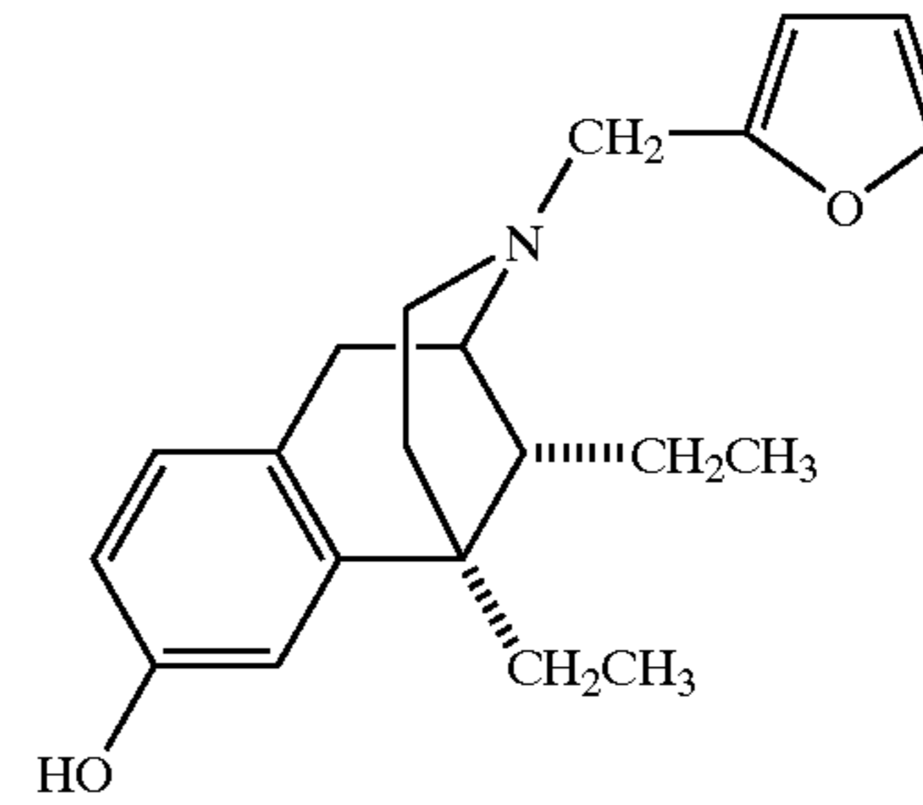
MR2266
