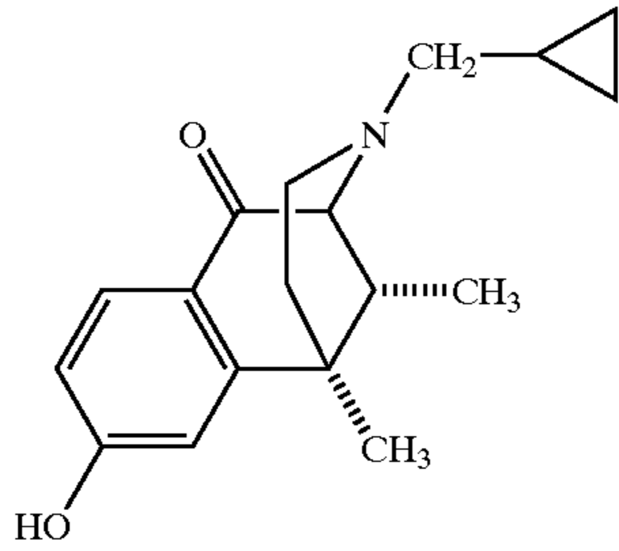
Ketocyclazocine
