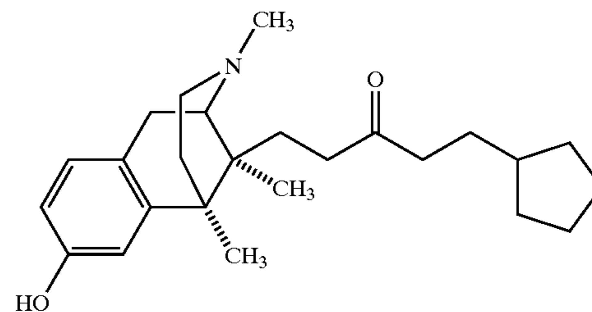
WIN 44,441
