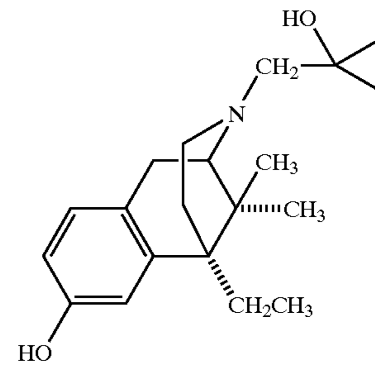
Bremazocine
