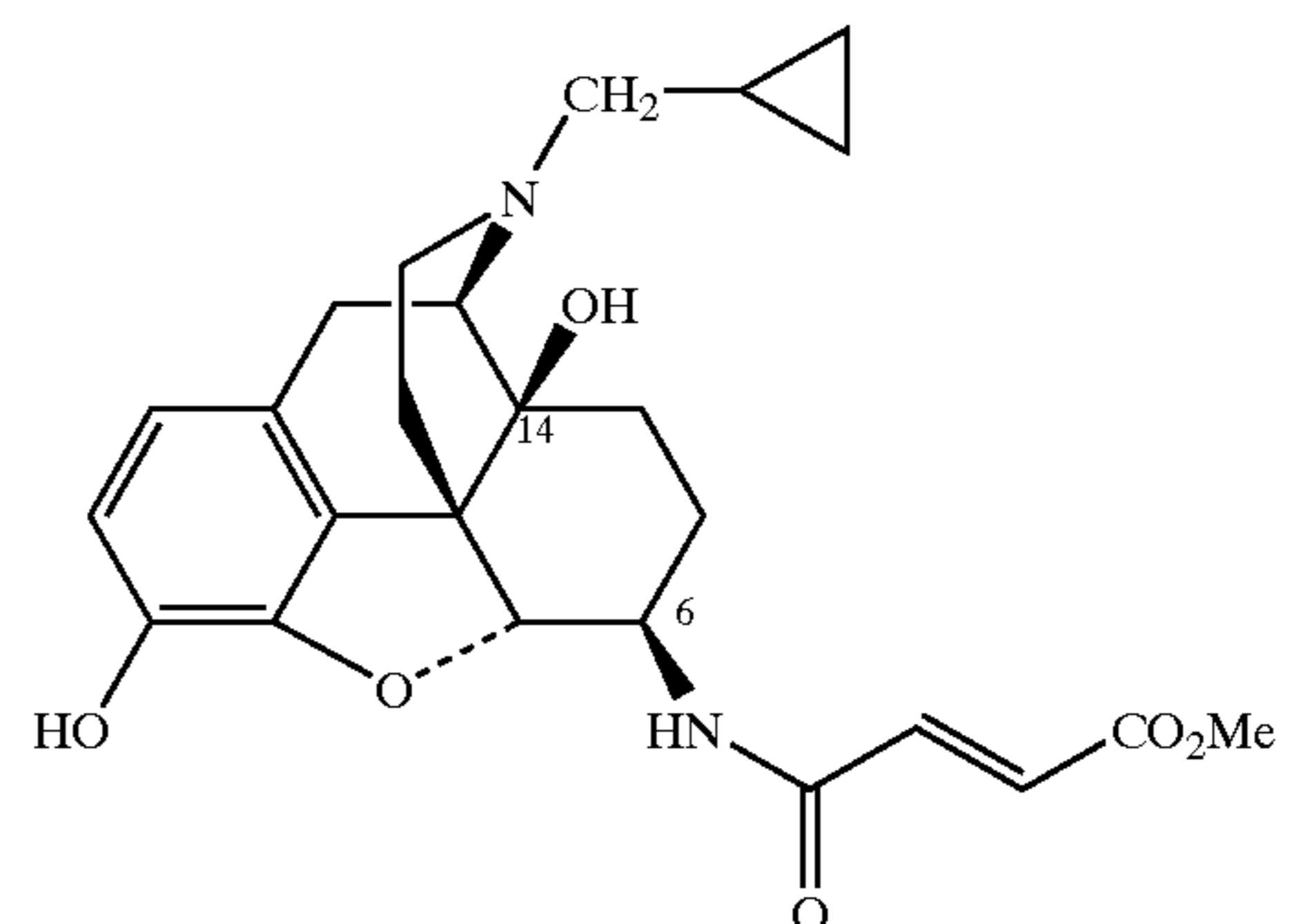
β-FNA
