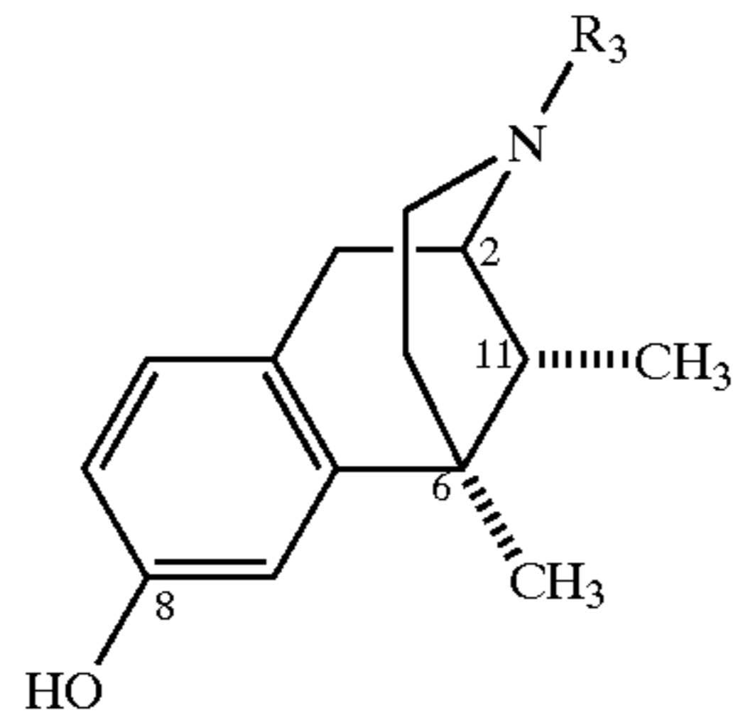
Chart 1. Opioid Receptor Ligands Benzomorphanins (a.k.a 2,6-Methano-3-benzazocines)
