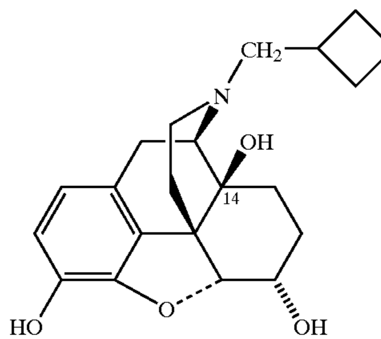
Nalbuphine
