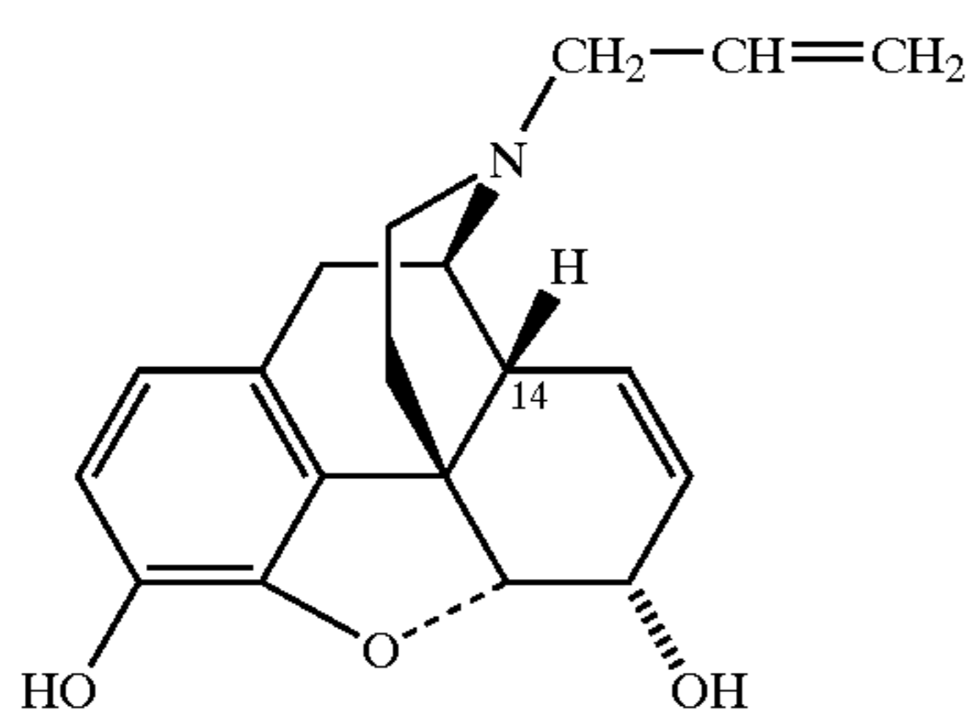
Nalorphine
