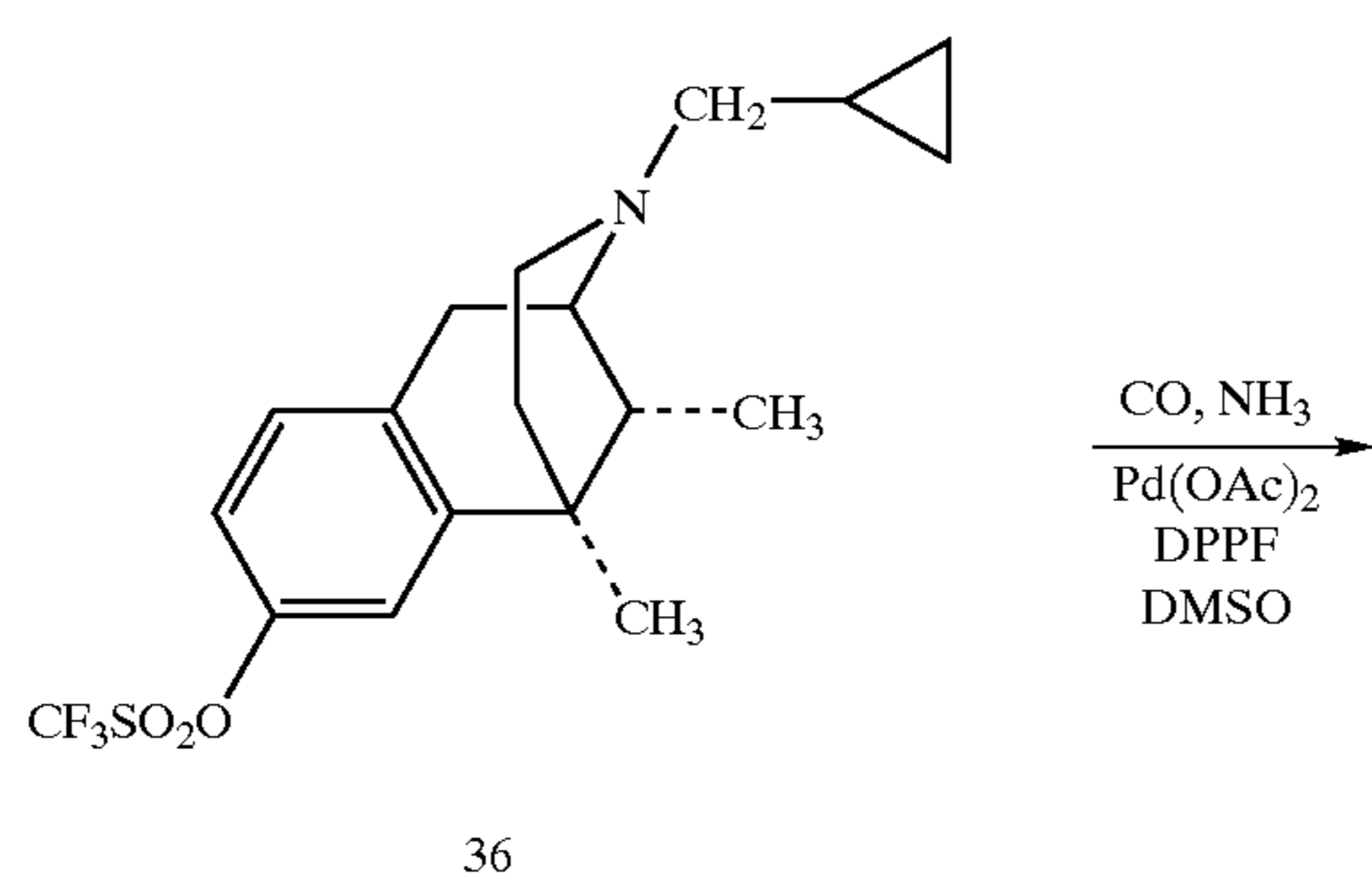
Scheme 2 - Alternate Carboxamide Synthesis
