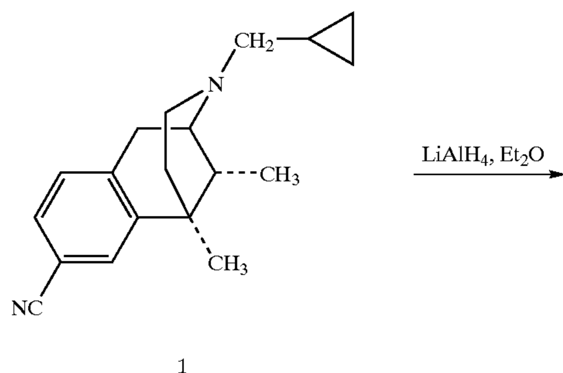
Scheme 3 - Miscellaneous Syntheses
