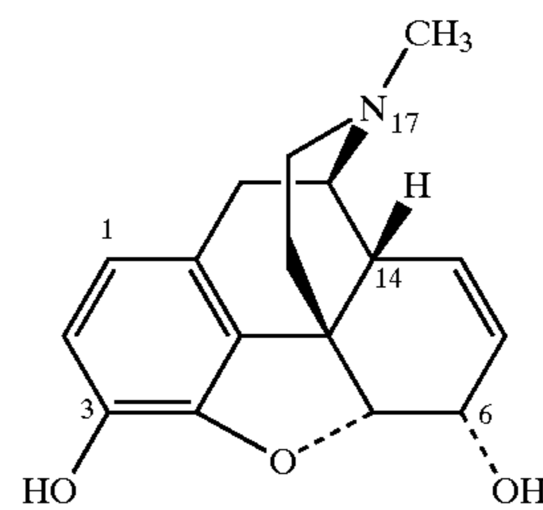
Morphine
