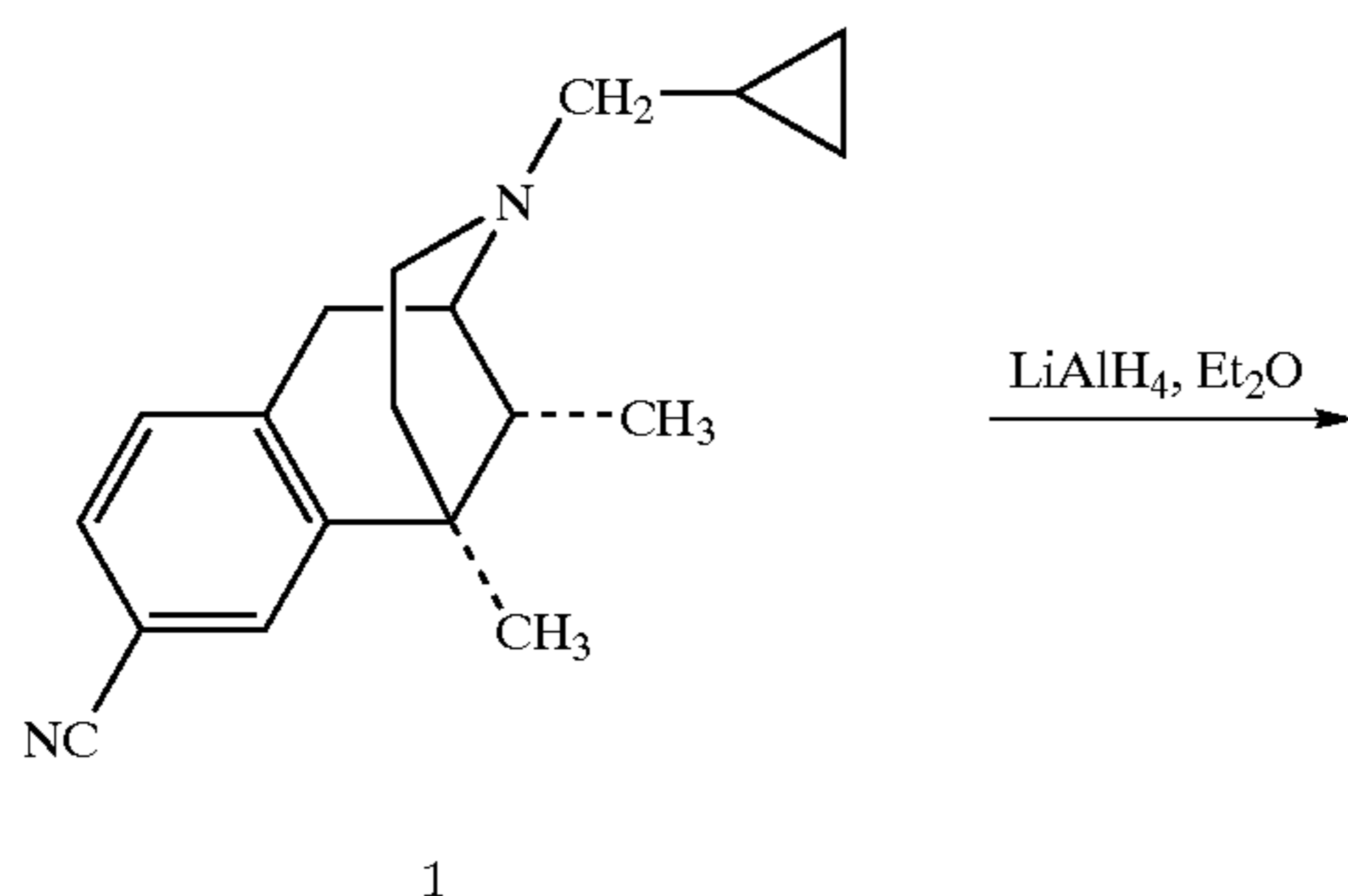
Scheme 3 - Miscellaneous Syntheses
