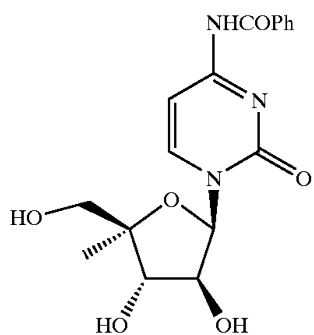
N4-Benzoyl-1-[4-C-methyl-beta-D-arabinofuranosyl]cytosine T. Yamaguchi et al., Nucleosides Nucleotides , 1997, 16(7), 1347
