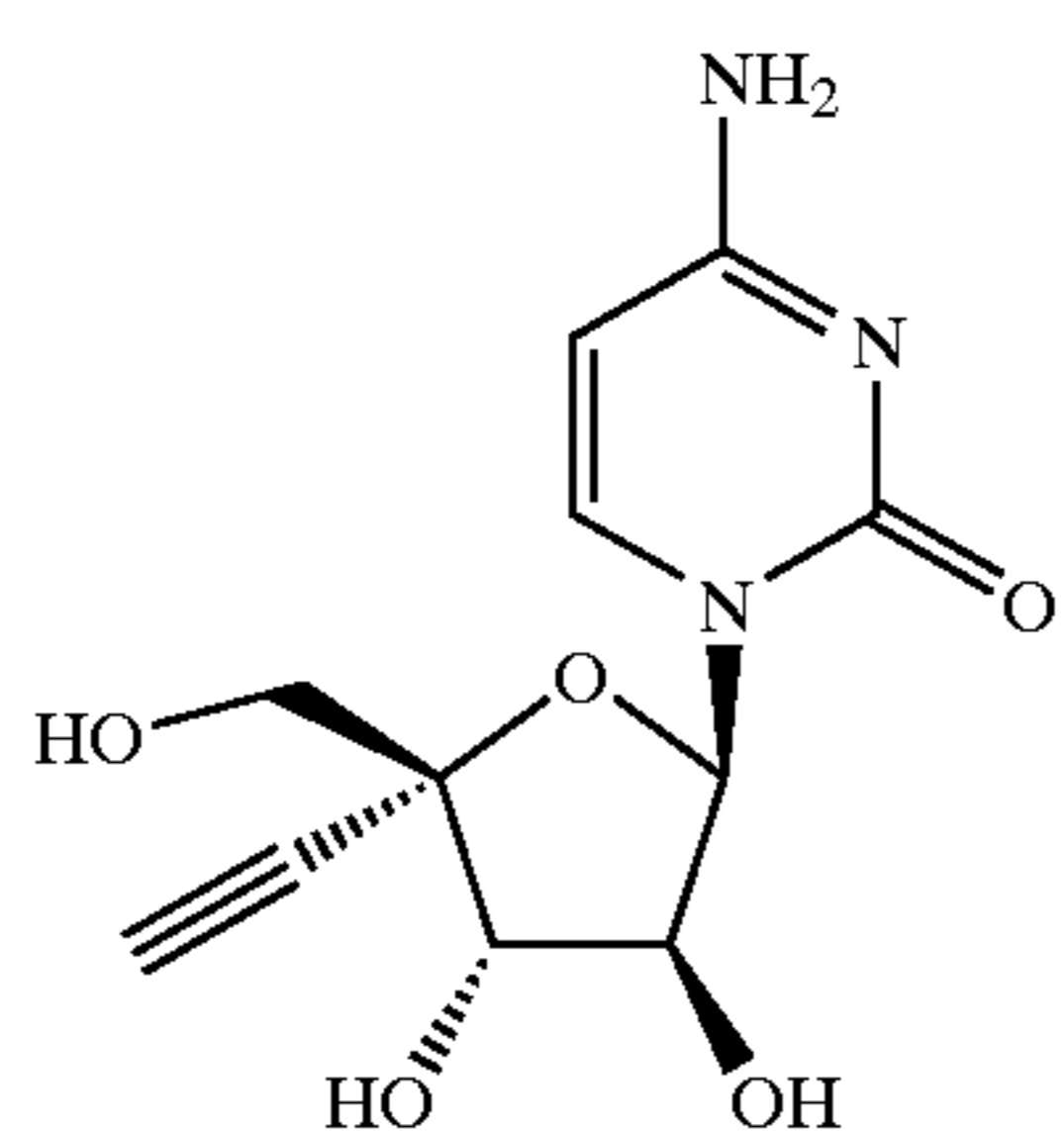
1-(4-C-Ethynyl-beta-D-arabinofuranosyl)cytosine H. Ohri et al, J. Med. Chem. , 2000, 43(23), 4516 or S. Kohgo et al., Biosci. Biotechnol. Biochem. , 1999, 63(6), 1146
