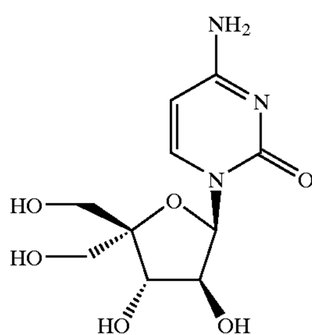
1-[4-C-(Hydroxymethyl)-beta-D-arabinofuranosyl]cytosine T. Waga et al., Nucleosides Nucleotides , 1996, 15(1-3) 287-304
