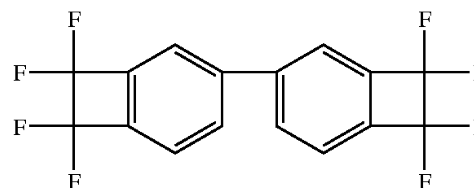
fluorobenzocyclobutene (BCB-F8)
