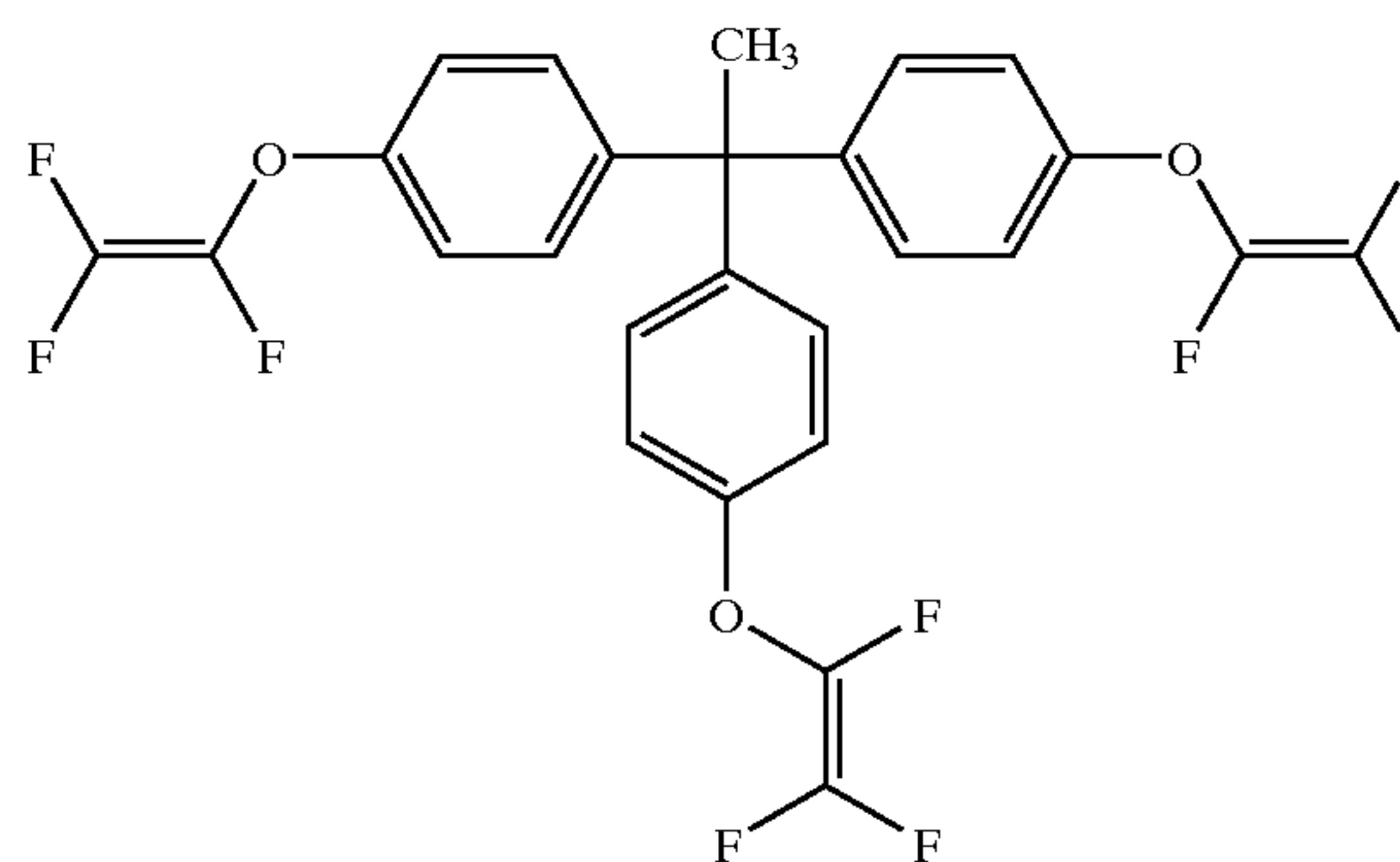
fluorobenzocyclobutene (BCB-F8)
