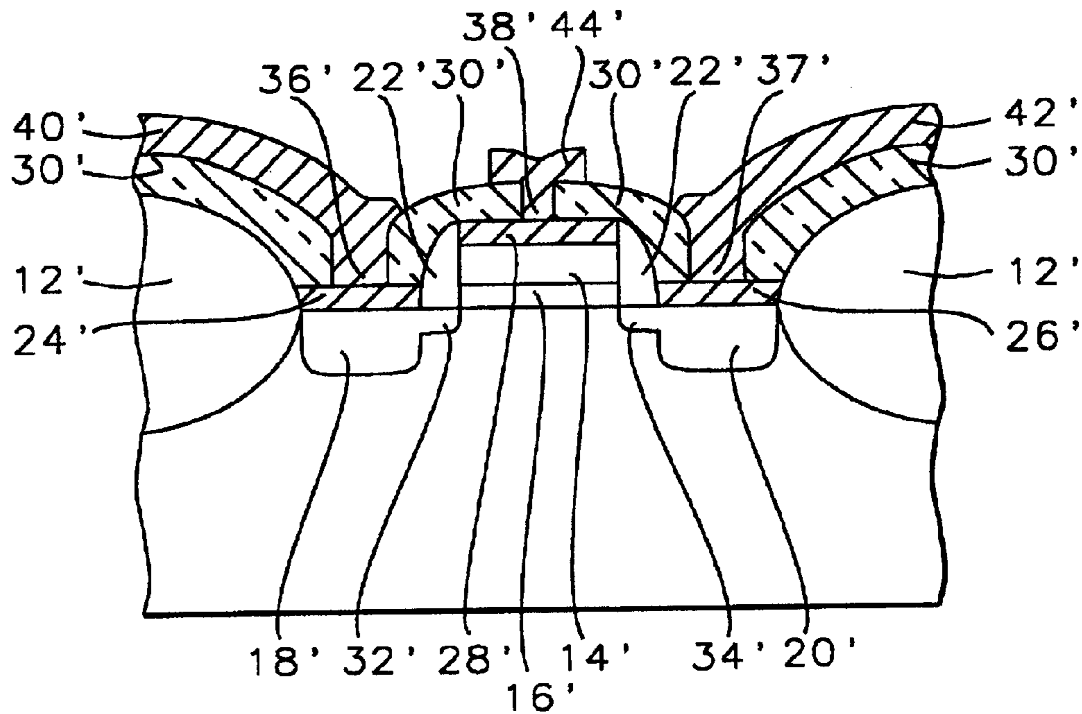
FIG. 1 - Prior Art
